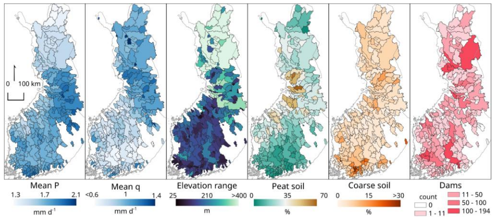
Figure 5: Multiple attributes exhibit great spatial variation over Finland. It should be noted that color scale for daily mean specific discharge runoff starts from has been limited to 0.6 mm d -1 on the low end, because due to anomalously low average the anomalously low discharges of gauge 3727 (0.19 mm d -1 ) would have made variation of other catchments harder to see runoff of gauge 3727 (0.19 mm d -1 ) . Similarly, shown elevation range was capped at 400 m (max. 804 m) to keep variation outside of Lapland visible and coarse soil percentage was capped at 30 % (max. 48 %) due to a few small outlier catchments covered by major glaciofluvial deposits.
