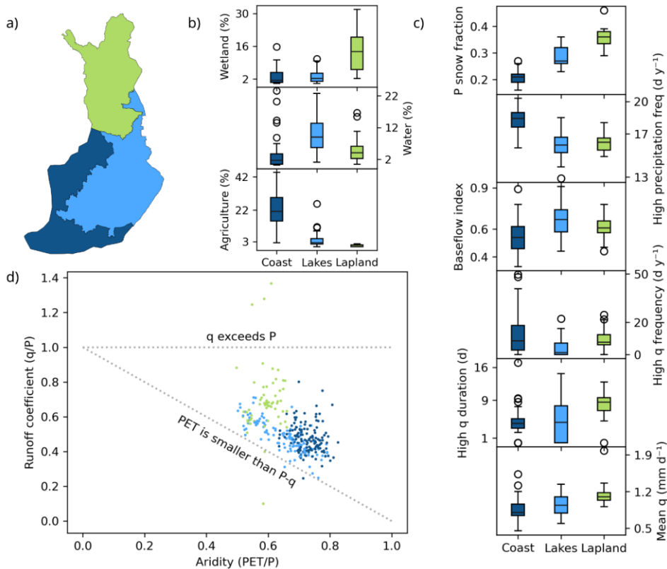
Figure 3: a) Map of the colours used to mark hydrological regions for the rest of the figure b) Variation in land cover between regions c) Variation in climate and dischargeflow regime between regions. Baseflow calculated with the methodology of Ladson et al. (2013) d) Gauges plotted by runoff ratioefficient and aridity. Inspiration for the figure from figure 2 of Coxon et. al. (2020)
