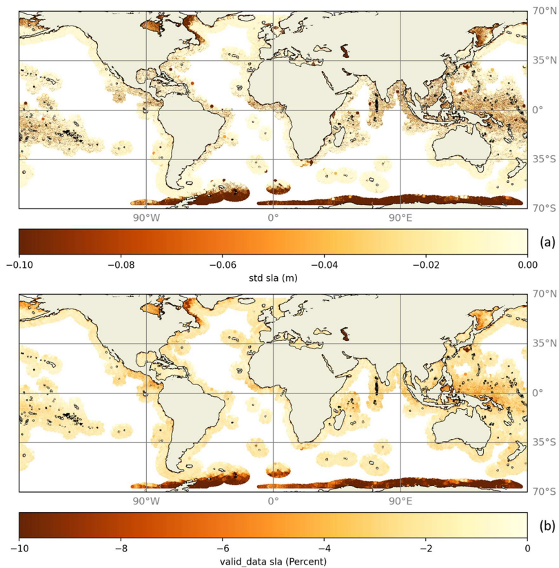
Figure 3: (a) Difference of ALTICAP SLA STD (in meters) before and after the validation flag is applied (edited-raw). (b) Percentage of SLA data lost when the validation flag is applied.
