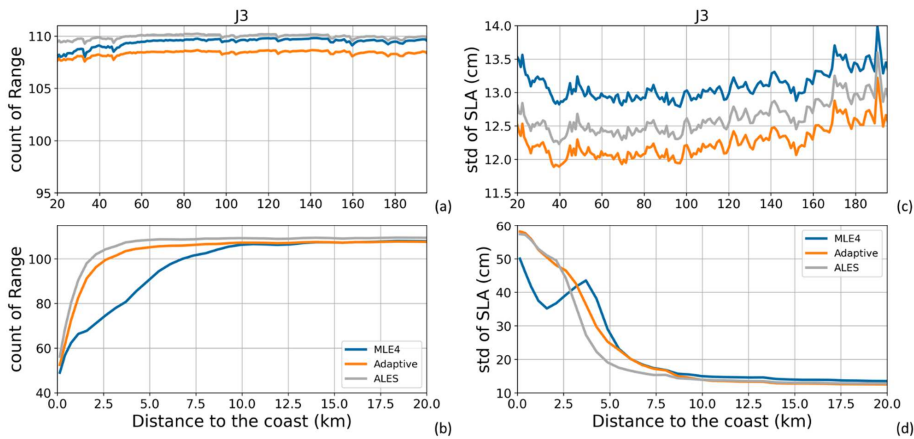
530 Figure A.1: (a, b) Global mean number of valid range data along all Jason-3 tracks for the period 17/02/2016 to 22/02/2019 (111 cycles). (c, d) Global mean of standard deviation values (in cm) of the SLA along all Jason-3 tracks for the same period, when using the different range solutions. Results are presented as a function of the distance to the coast (in km) between 200 and 20 km (a, c) and between 20 and 0 km (b, d) from the coast.
