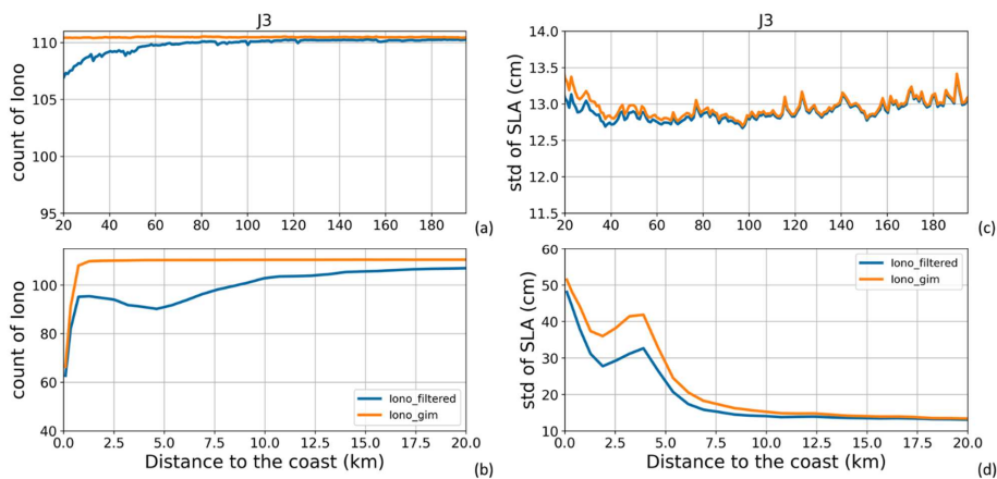
555 Figure A.3: (a, b) Global mean number of valid ionospheric correction data along all Jason-3 tracks for the period 17/02/2016 to 22/02/2019 (111 cycles). (c, d) Global mean of standard deviation values (in cm) of the SLA along all Jason-3 tracks for the same period, when using the different ionospheric correction solutions. Results are presented as a function of the distance to the coast (in km) between 200 and 20 km (a, c) and between 20 and 0 km (b, d) from the coast.
