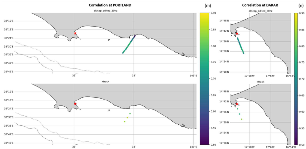
665 Figure B.1: (a to n) Maps of the correlation between each of the 14 tide gauge stations (red star on each map) and the along track altimetry SLAs (dots in color) from the ALTICAP 20 Hz dataset (upper plots) and the X-TRACK 1 Hz dataset (lower plots). Only altimetry points located at a distance lower than 20 km from the coast and 50 km from the tide gauge station are considered. The dot and dash-dot lines show the 200 m and 1000 m isobaths respectively.
