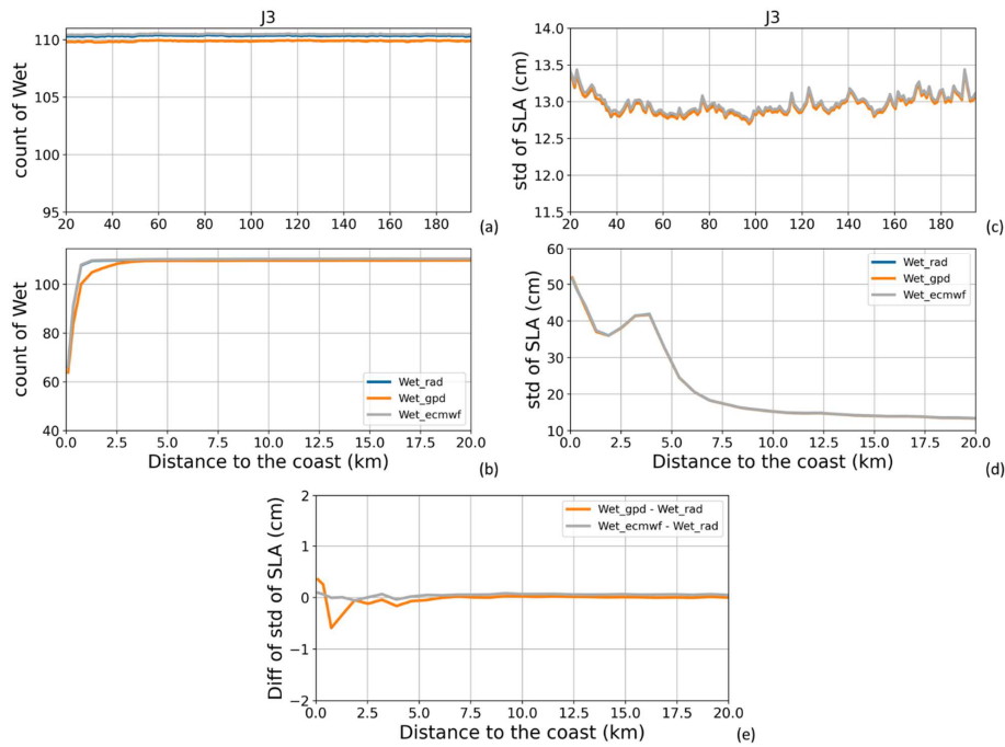
580 Figure A.4: (a, b) Global mean number of valid wet tropospheric correction data along all Jason-3 tracks for the period 17/02/2016 to 22/02/2019 (111 cycles). (c, d) Global mean of standard deviation values (in cm) of the SLA along all Jason-3 tracks for the same period, when using the different wet tropospheric correction solutions. (e) Difference (in cm) between the global mean of standard deviation values of the SLA along all Jason-3 tracks for the same period, when using the different wet tropospheric solutions and when using the reference solution (radiometer). Results are presented as a function of the distance to the coast (in km) between 200 and 20 km (a, c) and between 20 and 0 km (b, d, e) from the coast
