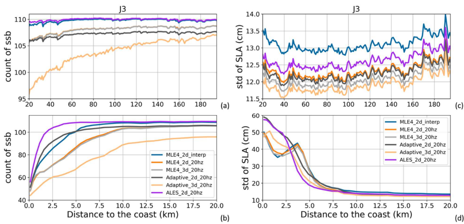
535 Figure A.2: (a, b) Global mean number of valid SSB data along all Jason-3 tracks for the period 17/02/2016 to 22/02/2019 (111 cycles). (c, d) Global mean of standard deviation values (in cm) of the SLA along all Jason-3 tracks for the same period, when using the different SSB solutions. Results are presented as a function of the distance to the coast (in km) between 200 and 20 km (a, c) and between 20 and 0 km (b, d) from the coast.
