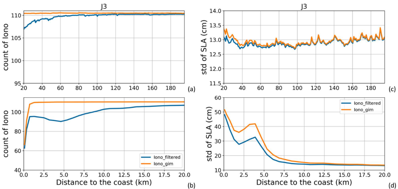
Figure A.3: (a, b) Global mean number of valid ionospheric correction data along all Jason-3 tracks for the period 17/02/2016 to 22/02/2019 (111 cycles). (c, d) Global mean of standard deviation values (in cm) of the SLA along all Jason-3 tracks for the same period, when using the different ionospheric correction solutions. Results are presented as a function of the distance to the coast (in km) between 200 and 20 km (a, c) and between 20 and 0 km (b, d) from the coast.
