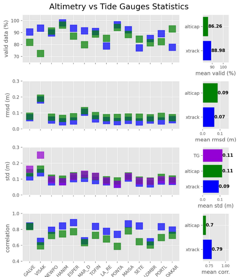
345 Figure 7: Mean statistics from the comparison between the edited ALTICAP (green) and X-TRACK (blue) SLAs and the selected tide gauges (for brevity, only the first 5 letters of the names are shown). The statistics have been computed for each altimetry point located at less than 20 km from the coast and less than 50 km from the tide gauge station and then averaged for each tide gauge. They are represented by tide gauge (left) and then averaged on a global scale (right). The standard deviation of the tide gauge SLA is also shown in purple.
