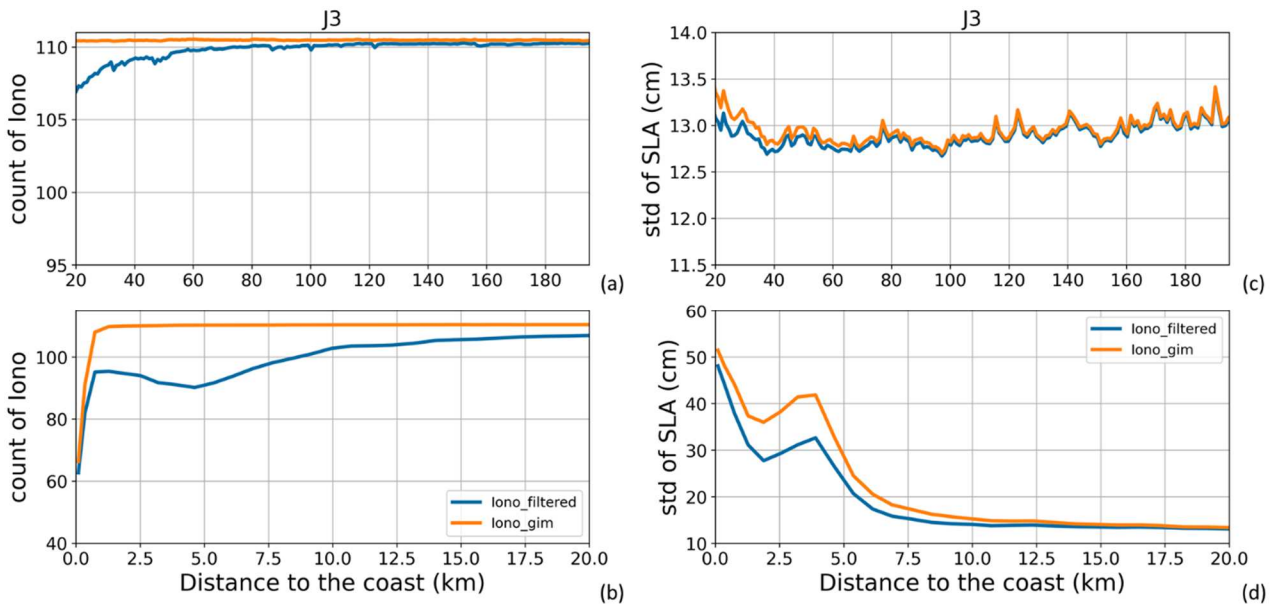
550 Figure A.3: (a, b) Global mean number of valid ionospheric correction data along all Jason-3 tracks for the period 17/02/2016 to 22/02/2019 (111 cycles). (c, d) Global mean of standard deviation values (in cm) of the SLA along all Jason-3 tracks for the same period, when using the different ionospheric correction solutions. Results are presented as a function of the distance to the coast (in km) between 200 and 20 km (a, c) and between 20 and 0 km (b, d) from the coast.
