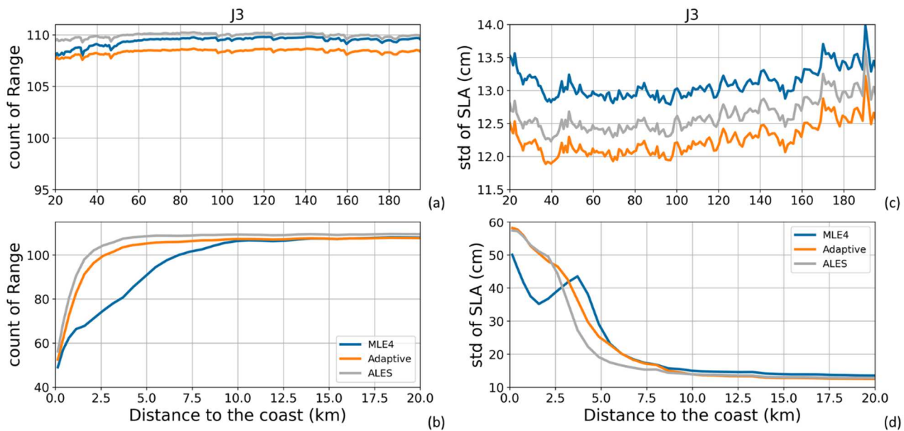
525 Figure A.1: (a, b) Global mean number of valid range data along all Jason-3 tracks for the period 17/02/2016 to 22/02/2019 (111 cycles). (c, d) Global mean of standard deviation values (in cm) of the SLA along all Jason-3 tracks for the same period, when using the different range solutions. Results are presented as a function of the distance to the coast (in km) between 200 and 20 km (a, c) and between 20 and 0 km (b, d) from the coast.
