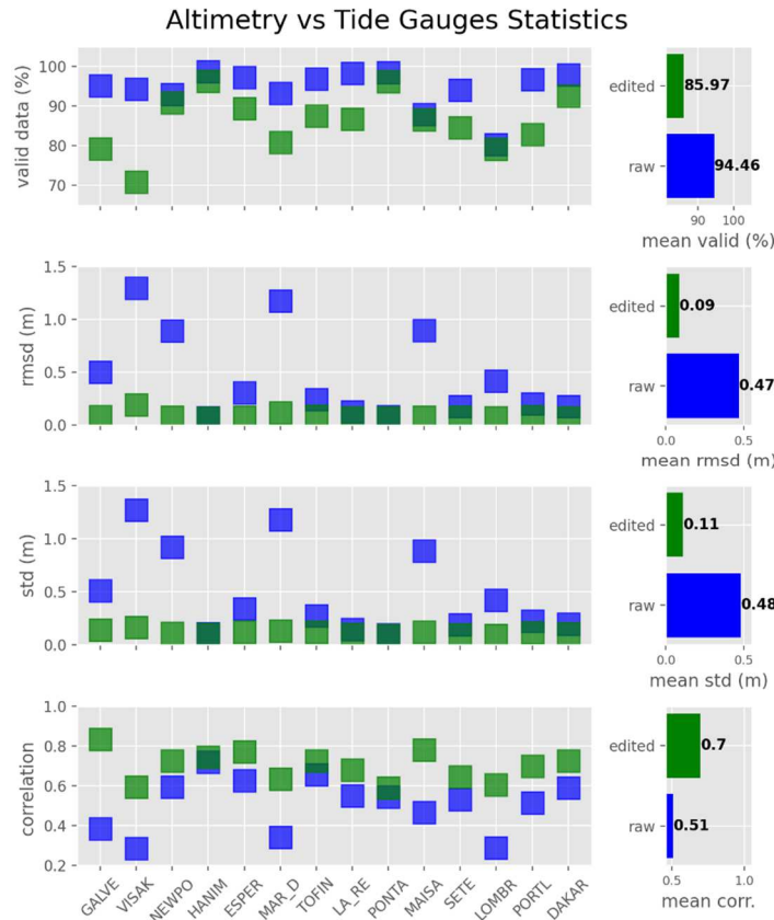
Figure 4: Mean statistics from the comparison between the raw (blue) and edited (green) SLAs of the ALTICAP product and the selected tide gauges (for brevity, only the first 5 letters of the names are shown). The statistics have been computed for each altimetry point located at less than 20 km from the coast and less than 50 km from the tide gauge station, and then averaged for each tide gauge. They are presented for each tide gauge (left) and then averaged on a global scale (right).
