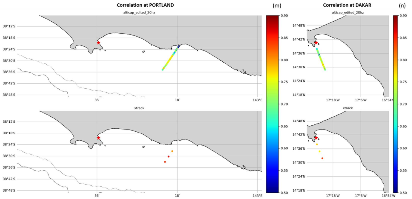
Figure B.1: (a to n) Maps of the correlation between each of the 14 tide gauge stations (red star on each map) and the along track altimetry SLAs (dots in color) from the ALTICAP 20 Hz dataset (upper plots) and the X-TRACK 1 Hz dataset (lower plots). Only altimetry points located at a distance lower than 20 km from the coast and 50 km from the tide gauge station are considered. The dot and dash-dot lines show the 200 m and 1000 m isobaths respectively.
