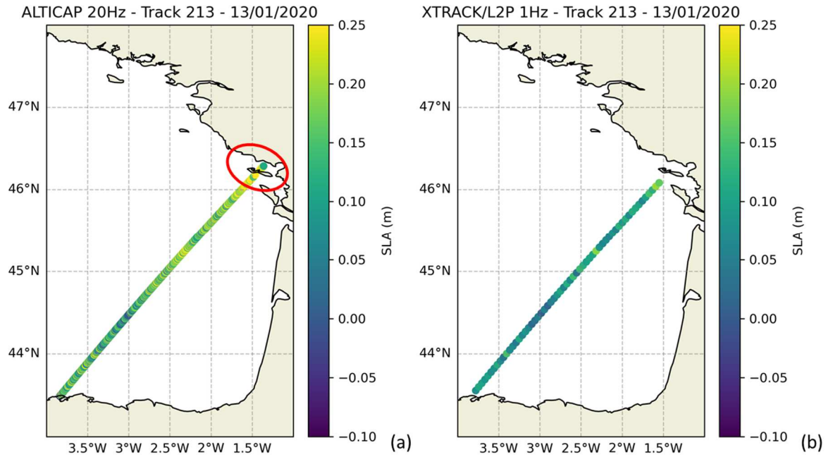
370 Figure 8: SLA (in meters) from the edited ALTICAP 20 Hz product (a) and the X-TRACK 1 Hz product (b) along the Jason-3 track 213, for cycle 142 (13/01/2020) in the Bay of Biscay (French Atlantic coast). The area of the Pertuis Charentais where the ALTICAP product brings additional data compared to the X-TRACK product is encircled in red.
