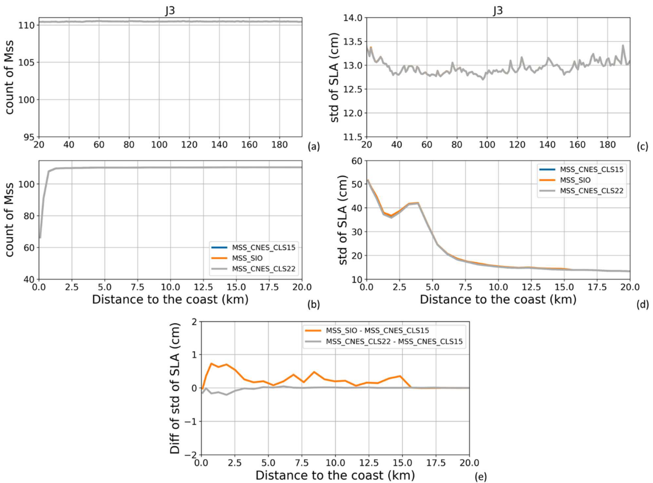
635 Figure A.6: (a, b) Global mean number of valid MSSH data along all Jason-3 tracks for the period 17/02/2016 to 22/02/2019 (111 cycles). (c, d) Global mean of standard deviation values (in cm) of the SLA along all Jason-3 tracks for the same period, when using the different MSSH solutions. (e) Difference (in cm) between the global mean of standard deviation values of the SLA along all
