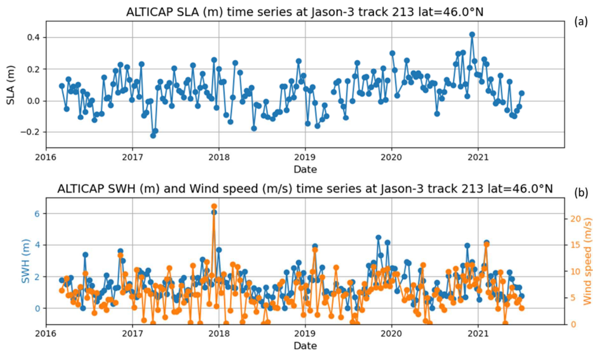
Figure 11: Time series of (a) SLAs and (b) Significant Wave Heights (SWH) and Wind speeds from the ALTICAP 20 Hz product at one point (latitude=46.0°N) of the Jason-3 track 213 in the Bay of Biscay, for the whole time period available (2016-2021). The SWHs larger than 10 m have been edited for the plot.
