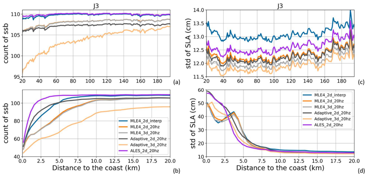
530 Figure A.2: (a, b) Global mean number of valid SSB data along all Jason-3 tracks for the period 17/02/2016 to 22/02/2019 (111 cycles). (c, d) Global mean of standard deviation values (in cm) of the SLA along all Jason-3 tracks for the same period, when using the different SSB solutions. Results are presented as a function of the distance to the coast (in km) between 200 and 20 km (a, c) and between 20 and 0 km (b, d) from the coast.
