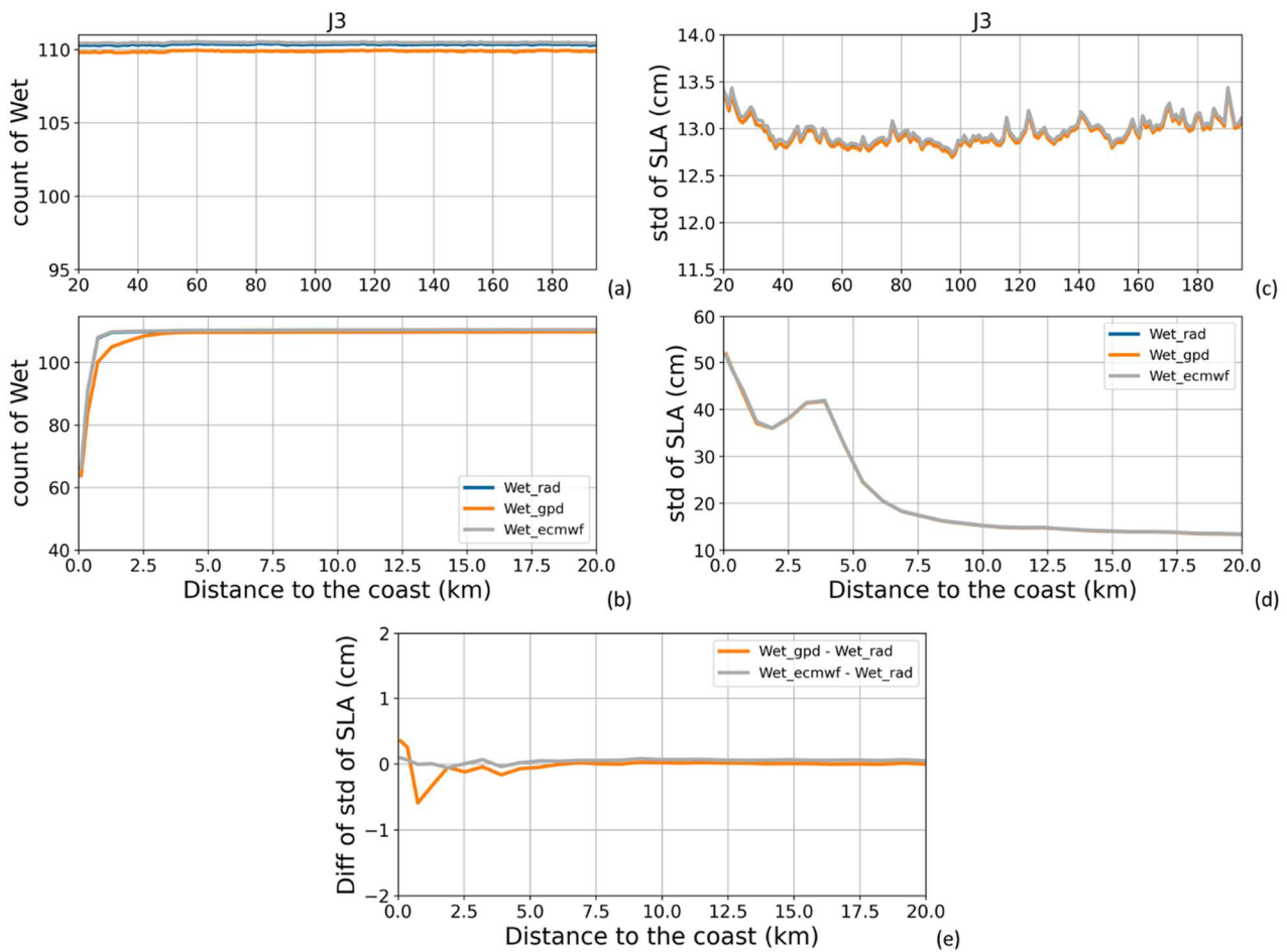
575 Figure A.4: (a, b) Global mean number of valid wet tropospheric correction data along all Jason-3 tracks for the period 17/02/2016 to 22/02/2019 (111 cycles). (c, d) Global mean of standard deviation values (in cm) of the SLA along all Jason-3 tracks for the same period, when using the different wet tropospheric correction solutions. (e) Difference (in cm) between the global mean of standard 580 deviation values of the SLA along all Jason-3 tracks for the same period, when using the different wet tropospheric solutions and when using the reference solution (radiometer). Results are presented as a function of the distance to the coast (in km) between 200 and 20 km (a, c) and between 20 and 0 km (b, d, e) from the coast
