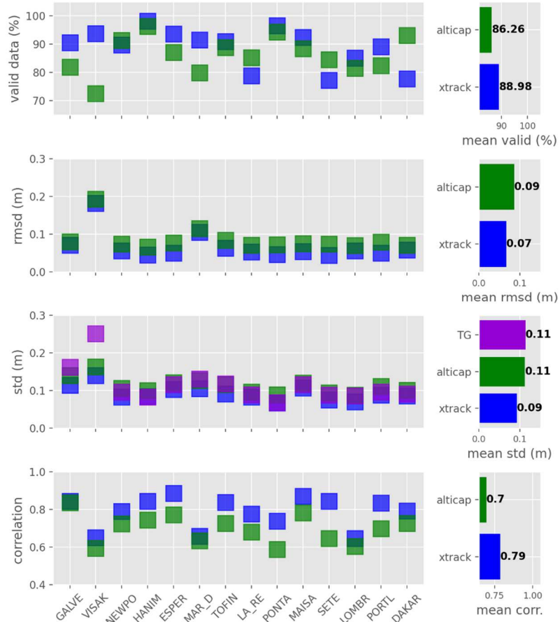
Figure 7: Mean statistics from the comparison between the edited ALTICAP (green) and X-TRACK (blue) SLAs and the selected tide gauges (for brevity, only the first 5 letters of the names are shown). The statistics have been computed for each altimetry point located at less than 20 km from the coast and less than 50 km from the tide gauge station and then averaged for each tide gauge. They are represented by tide gauge (left) and then averaged on a global scale (right). The standard deviation of the tide gauge SLA is also shown in purple.
