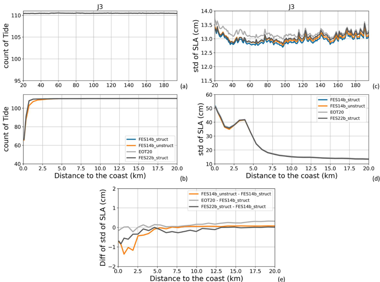
610 Figure A.5: (a, b) Global mean number of valid ocean tide correction data along all Jason-3 tracks for the period 17/02/2016 to 22/02/2019 (111 cycles). (c, d) Global mean of standard deviation values (in cm) of the SLA along all Jason-3 tracks for the same period, when using the different ocean tide correction solutions. (e) Difference (in cm) between the global mean of standard deviation values of the SLA along all Jason-3 tracks for the same period, when using the different tide solutions and when using the reference solution (FES2014b struct). Results are presented as a function of the distance to the coast (in km) between 200 and 20 km (a, c) and between 20 and 0 km (b, d, e) from the coast.
