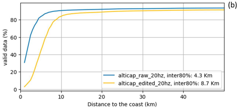
275 Figure 2: Standard deviation (a) in meters, and percentage (b) of SLA data as a function of the distance to the coast, for the raw (blue) and edited (orange) ALTICAP SLAs. Inter80% refers to the distance to the coast at which 80 % of data availability is obtained.
