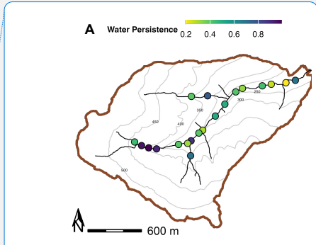
Deleted: Figure 3: (A) Flow persistence over the study period (August 2021–October 2024) at each water presence-absence sensor site across the Coastal Plain study watershed. Light colors indicate less water persistence and darker colors indicate continuous water persistence. (B) Sampling dates, (C) discharge at the watershed outlet ( Q ; L s^{-1} ) and (D) percent network wet (see Section 3.2.2 for further details) across the study period. For a given sampling date, purple circles refer to temporal sampling at the watershed outlet (sampling approach 1; Section 2.2.2) and orange squares for seasonal synoptic sampling at the seven long-term monitoring sites in the stream network (sampling approach 2; Section 2.2.3).
