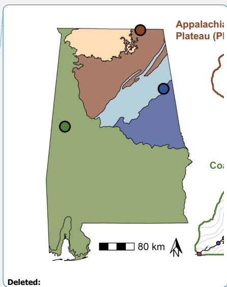
Deleted: Figure 1: (left) Map of Alabama, USA with locations of the three study watersheds. Points shown on the Alabama map as well as the outlines of the Piedmont (Talladega; TAL; right, blue), Appalachian Plateau (Paint Rock; PRF; top, brown), and Coastal Plain (Shambley Creek; WHR; bottom, green) study watersheds are colored based on their respective physiographic province. Locations of water presence-absence sensors (STIC; purple circles), long-term monitoring sites (LTM; gold triangles), and watershed outlet monitoring sites (Supersensor; pink squares) in the stream network are shown on each watershed map (see Section 2.2.1). Additional water presence-absence sensors (Bonus STIC; open circles with purple outline) were installed in the Piedmont study watershed during 2022 to correspond with sites sampled during a spatially-intensive synoptic sampling campaign in June 2022 (sampling approach 3; see Section 2.2.4).
