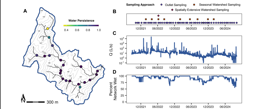
Figure 2: (A) Flow persistence over the study period (September 2021–October 2024) at each water presence-absence sensor site across the Piedmont study watershed (TAL). Light colors indicate less continuous water persistence and darker colors indicate more continuous water persistence. (B) Sampling dates, (C) discharge at the watershed outlet ( Q ; L s^{-1} ) and (D) percent network wet using the water presence-absence sensor network (see Section 3.2.2 for further details) across the study period. For a given sampling date, purple circles refer to temporal sampling at the watershed outlet (Section 2.2.2) and orange squares for seasonal synoptic sampling at the seven long-term monitoring sites in the stream network (Section 2.2.3) and pink diamonds for an extensive spatial synoptic sampling campaign across the watershed (Section 2.2.4). Contours in the watershed map refer to relative elevation change throughout the watershed.
