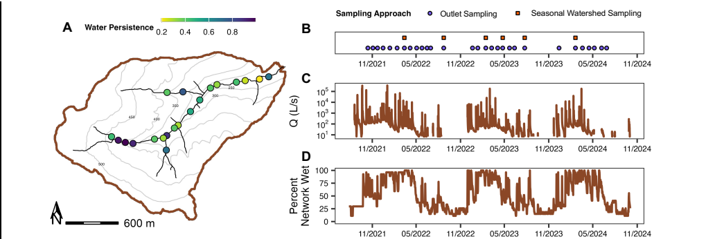
Figure 3: (A) Flow persistence over the study period (August 2021–October 2024) at each water presence-absence sensor site across the Appalachian Plateau study watershed (PRF). Light colors indicate less continuous water persistence and darker colors indicate more continuous water persistence. (B) Sampling dates, (C) discharge at the watershed outlet ( Q ; L s^{-1} ) and (D) percent network wet estimated using the water presence-absence sensor network (see Section 3.2.2 for further details) across the study period. For a given sampling date, purple circles refer to temporal sampling at the watershed outlet (Section 2.2.2) and orange squares for seasonal synoptic sampling at the seven long-term monitoring sites in the stream network (Section 2.2.3). Contours in the watershed map refer to relative elevation change throughout the watershed.
