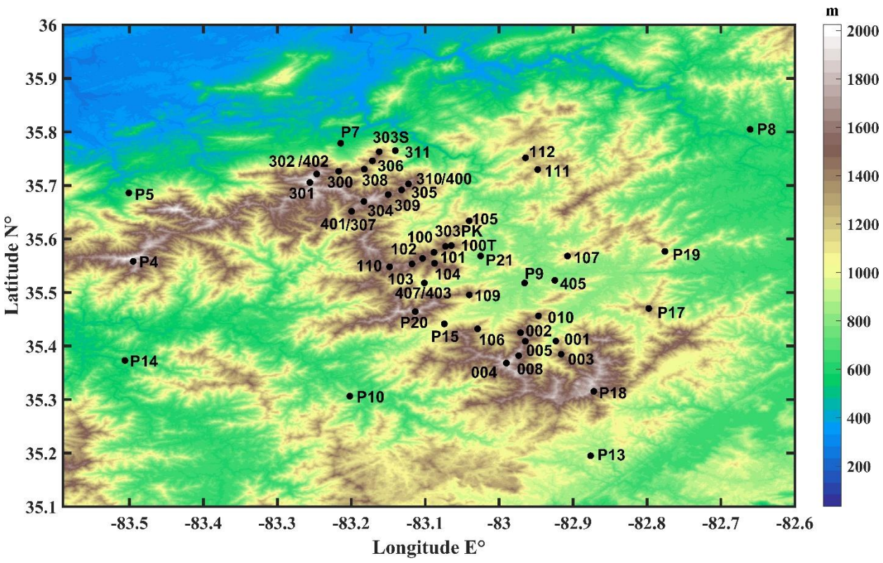
1316 Figure 1 - Map of IPHEX (Barros et al., 2014) ground-based observations in the Southern 1317 Appalachians. Raingauge is denoted as a character string starting with three-digit number 1318 potentially followed by extra letters; locations started with a letter P represent disdrometers. The 1319 basic information regarding these stations is listed in Table 1. This figure is adapted from Liao and 1320 Barros (2019).
