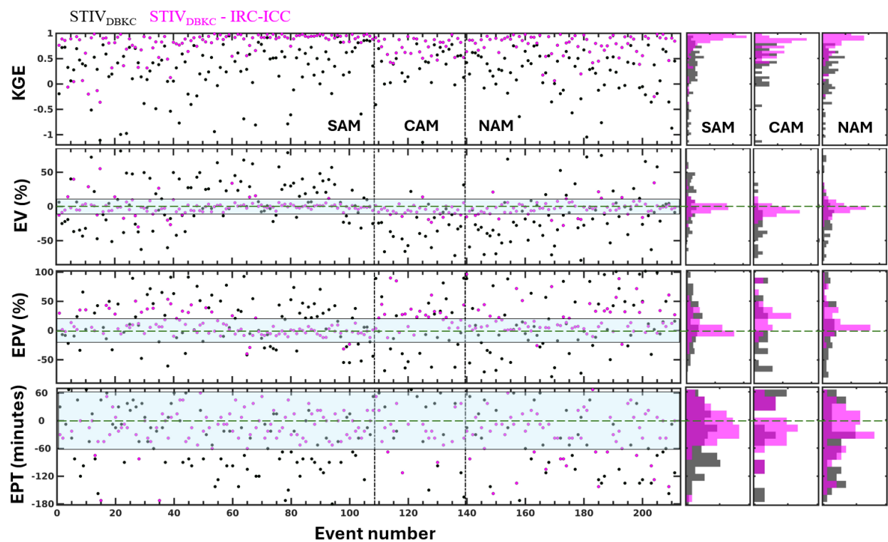
Figure 12 – Summary of hydrologic skills. Green dashed lines and associated uncertainty envelopes are only for visual illustration. Hydrologic statistics are explained in Table 2. Pink and black scatters (each scatter represent one event) represent IRC-ICC, and baseline outputs, respectively. Each horizontal panel is split into 3 subsections by vertical black lines representing the 3 subregions. Histograms graphs on the right hand side are provided for a summary view. This figure is adapted from Liao and Barros (2025b).
