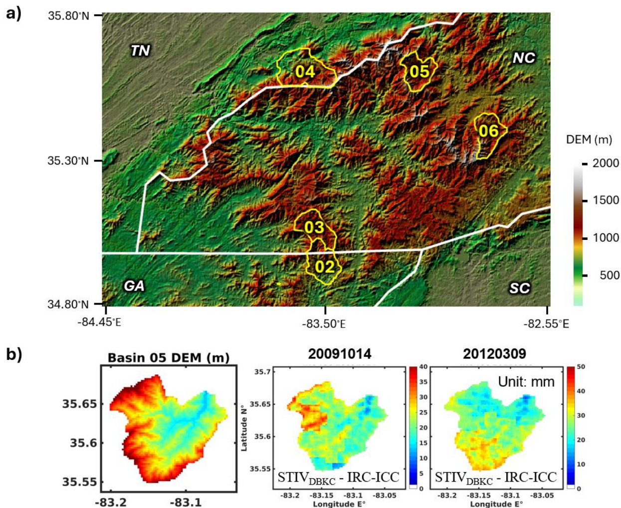
837 Figure A3 – A zoom-in map of the Figure 4 for watersheds in the Southern Appalachians (Panel 838 a). The DEM map and examples of rainfall event accumulation of Basin 05 (Panel b) to show 839 rainfall alignment with topography.
