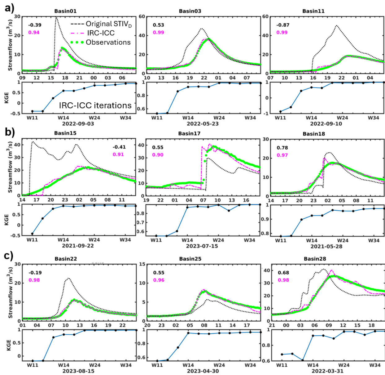
1389 Figure 9 – The IRC-ICC performance for different subregions, include a) 3 events from the 1390 Southern Appalachians; b) 3 events from the Central Appalachians; and c) 3 events from the 1391 Northern Appalachians. The IRC-ICC KGE evolution plots from iterations are included below the 1392 hydrographs. The black and pink line are from the original STIV D and the IRC-ICC equilibrium 1393 state (STIV D IRC* ), respectively, and KGE values are displayed as colored numbers in the top left 1394 corners. This figure is adapted from Liao and Barros (2025b). 1395
