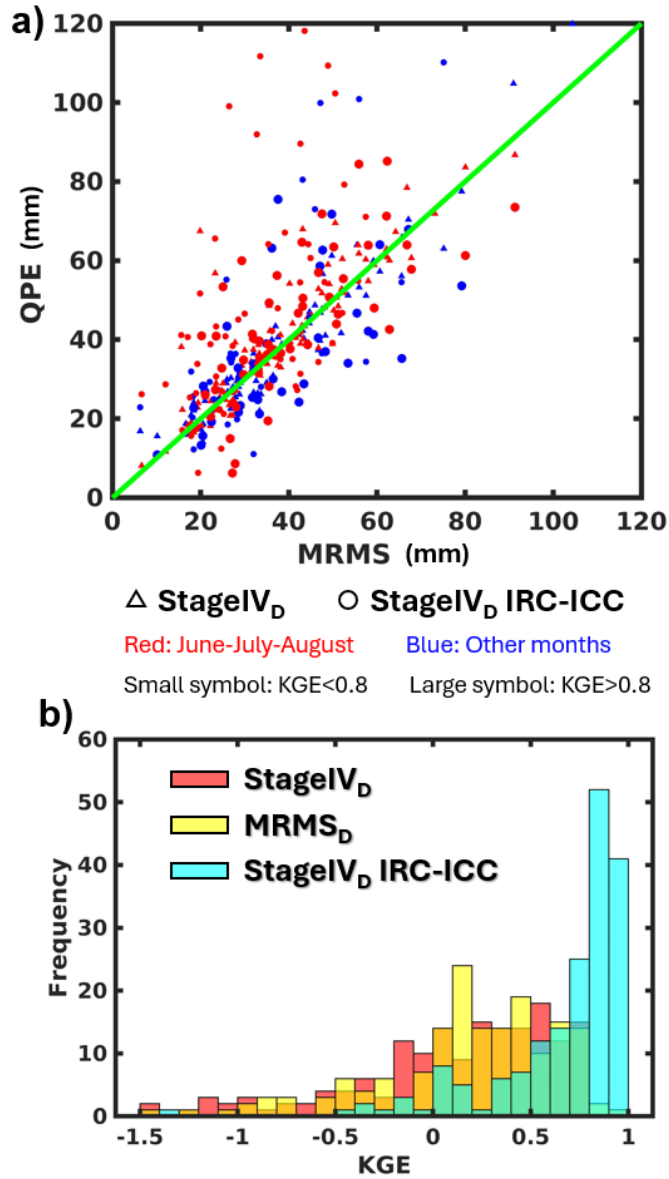
Figure 13 – a) Event total QPE plots for various QPE datasets conditional on seasons and KGE values; b) KGE distributions across events using different QPE datasets. This figure is adapted from Liao and Barros (2025b).
