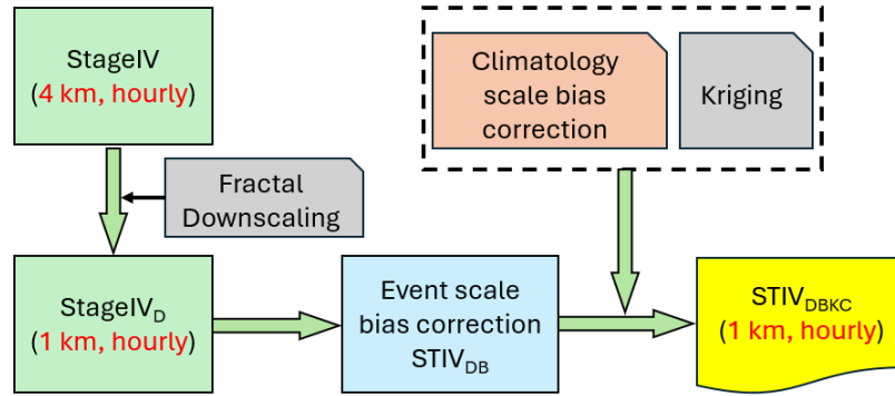
Figure 2 – Workflow to generate the product STIV DBKc .
