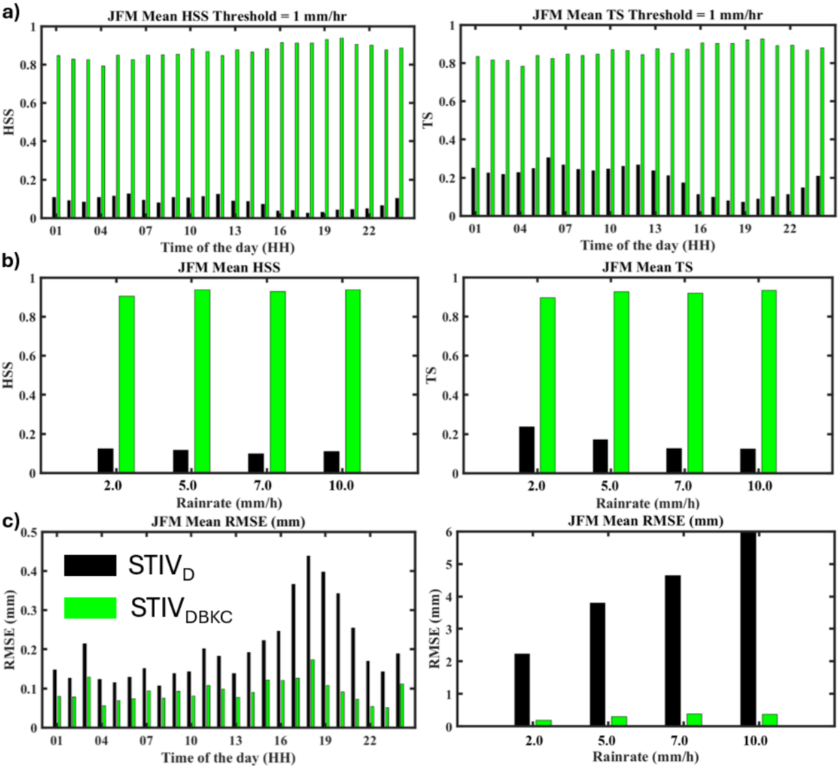
Figure 7 – Statistical evaluation summary for winter precipitation (JFM, January, February, and March): a) Diurnal cycle of mean HSS and TS statistics including all rain gauges calculated using all data from 2008 to 2017: STIV D (black) and STIV DBKC (green); b) HSS and TS statistics calculated using different rain rate thresholds over the same 10-year period; c) Diurnal cycle of rain rate RMSE at seasonal-scale, and its dependence on observed rainfall rate. This figure is from Liao and Barros (2019).
