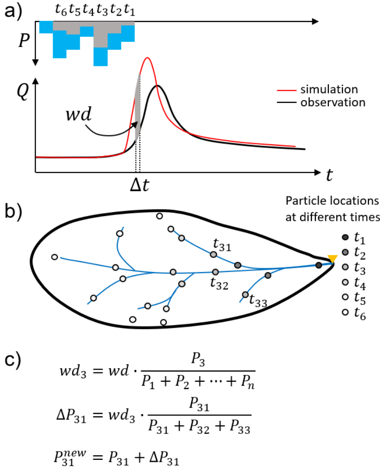
Figure A2 - Schematic depiction of the IRC framework and key mathematical equations. Panel (a) illustrates the nonlinear relationship between streamflow and precipitation, where wd represents the residual between discharge simulations and observations at the basin outlet. The variation of precipitation in the basin as a function of time is shown by the basin hyetograph in blue. The hyetograph time series (blue) spans the duration of the precipitation event between t_1 to t_n . In gray is the hyetograph over the area of interest for panels (b) and (c). To map the streamlines, water particles are launched every time step and their trajectory to the outlet is tracked and saved. Panel (b) shows the source areas of water particles launched at various time steps ( t_1, t_2, \dots, t_6, \dots ) from all locations where runoff is produced, and the particles are tracked until they eventually reach the basin outlet. The streamlines of particles that reach the outlet at the same time
