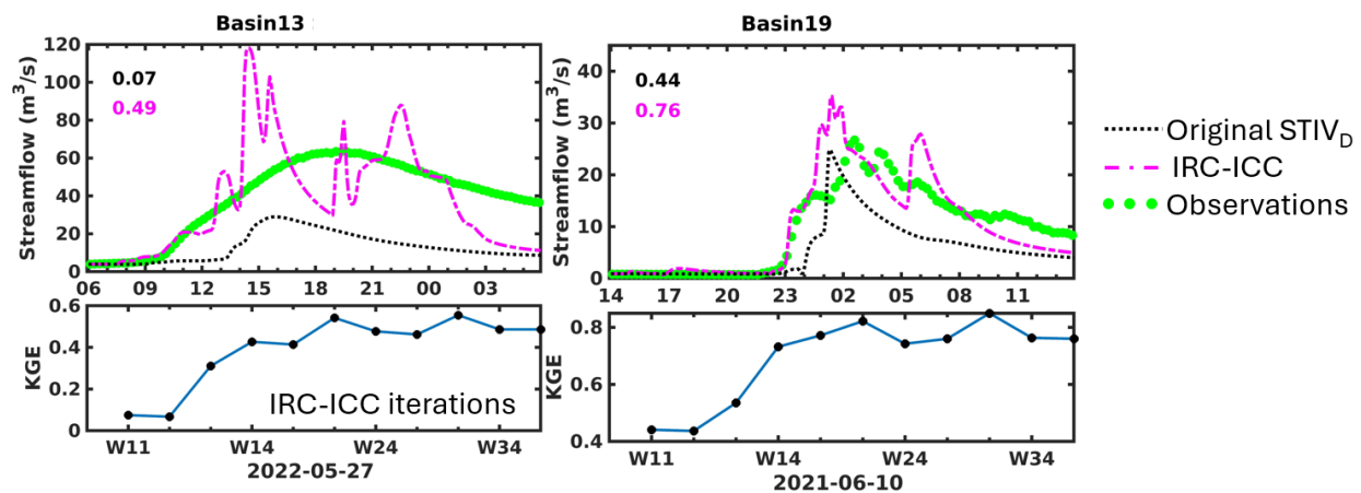
846 Figure A4 – Examples of the coupled IRC-ICC framework application in Basin 13 and Basin 19 847 for discussion in the manuscript. KGE values are displayed in the top left corners. Basin 13 is 848 located in Karst terrain, while the event in Basin 19 is an example with a complex hydrograph.
