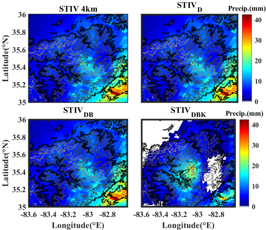
Figure A1 - Spatial rainfall fields on 2014-05-15, 06-07 UTC. Rain rates between 0 to 1mm/h are mapped in white.
