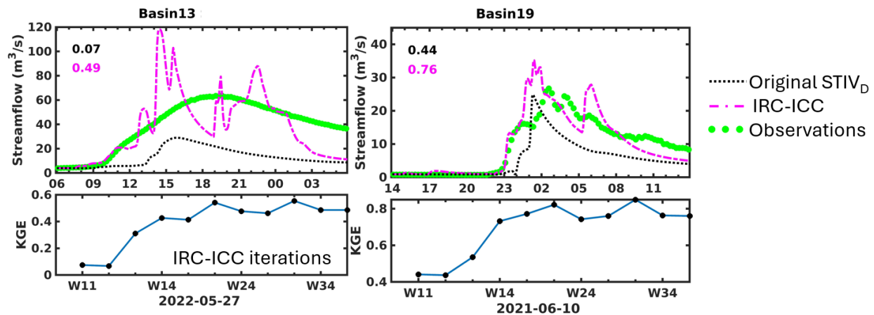
Figure A3 – Examples of the coupled IRC-ICC framework application in Basin 13 and Basin 19 for discussion in the manuscript. KGE values are displayed in the top left corners. Basin 13 is located in Karst terrain, while the event in Basin 19 is an example with a complex hydrograph.
