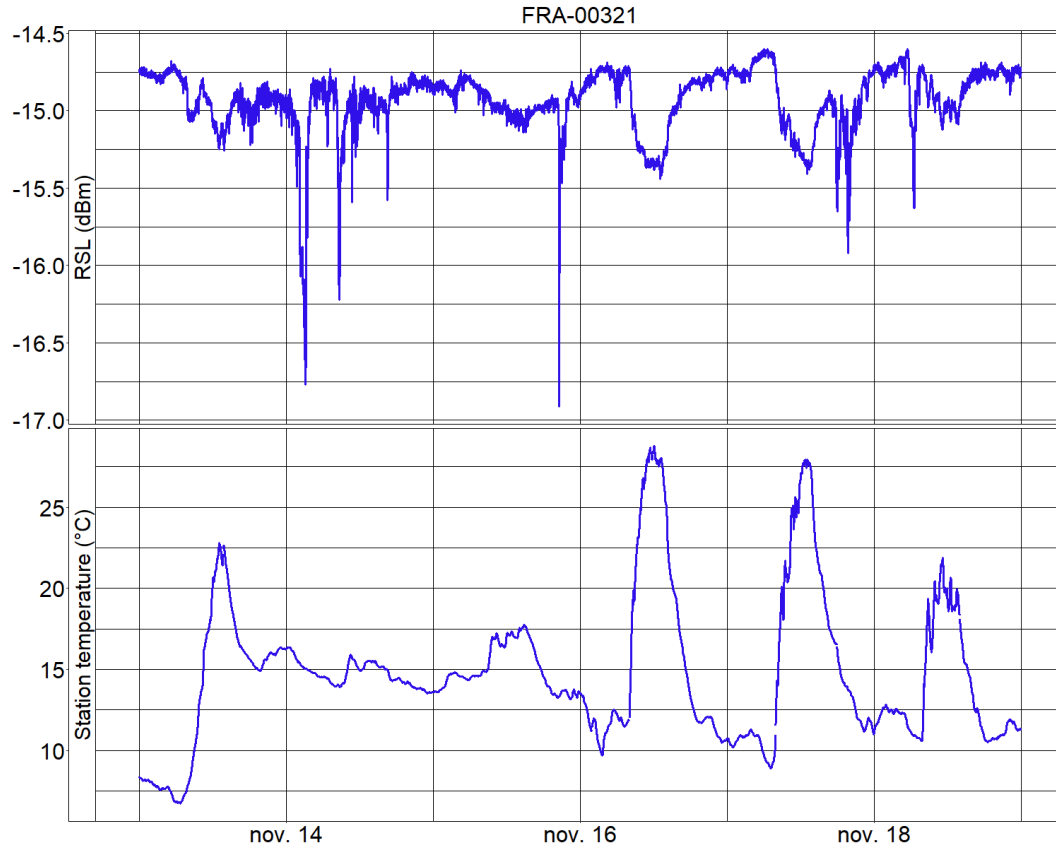
Figure 12. Example of RSL (dBm) pattern and corresponding temperature (°C) measurements. Station: FRA-00321.
