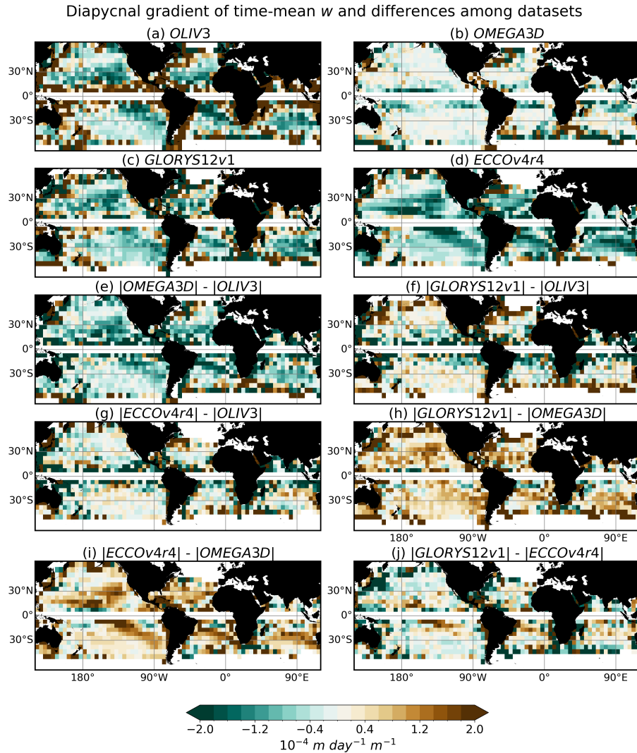
Figure 6. Diapycnal gradient of time-mean vertical velocity between the base of the maximum mixed layer depth and \sigma_{27} (Eq. 16) at 5^\circ \times 5^\circ spatial resolution, shown for: (a) OLIV3, (b) OMEGA3D, (c) GLORYS12v1, and (d) ECCOV4r4. Negative values indicate a decrease in vertical velocity magnitude with depth, while positive values depict increasing magnitude with depth. (e-j) Differences between modules in the diapycnal gradient of time-mean vertical velocity for the various datasets.
