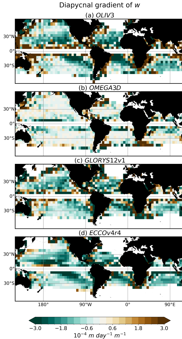
Figure A1. Diapycnal gradient of time-mean vertical velocity between the base of the maximum mixed layer depth and \sigma_{26.5} (Eq. 16) at 5^\circ \times 5^\circ spatial resolution, shown for: (a) OLIV3 , (b) OMEGA3D , (c) GLORYS12v1 , and (d) ECCOv4r4 . Negative values indicate a decrease in vertical velocity magnitude with depth, while positive values depict increasing magnitude with depth.
