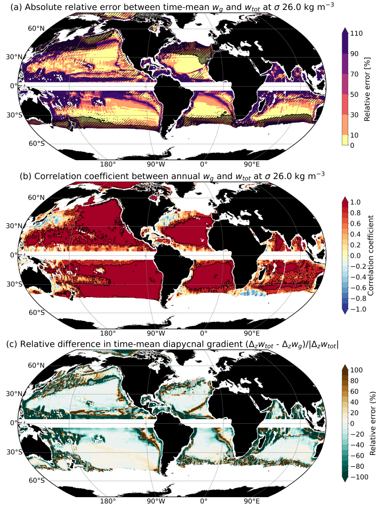
Figure 4. Assessment of OGCM geostrophic vertical velocity estimate against the OGCM total vertical velocity. (a) Absolute relative error between means of geostrophic vertical velocity and total vertical velocity at \sigma_{26} isopycnal surface. Translucent black shading represents regions within the maximum mixed layer over the study period and hatching delimits the areas where the LVB does not hold (relative error > 10%). (b) Correlation coefficient between the annual geostrophic vertical velocity and total vertical velocity at \sigma_{26} isopycnal surface. Black contours indicate correlation coefficients of 0.7 (dashed) and 0.9 (solid). (c) Relative difference in vertical diapycnal gradient of total and geostrophic time-mean vertical velocity ( \Delta_z w_{tot} and \Delta_z w_g respectively ) between the mixed layer base and \sigma_{27} , computed as (w_{\sigma_{27}} - w_{\sigma_{MLD}}) / (\sigma_{27} - \sigma_{MLD}) \Delta_z w = (|w_{\sigma_{27}}| - |w_{\sigma_{MLD}}|) / (|z_{\sigma_{27}} - z_{\sigma_{MLD}}|) normalised by the magnitude of the diapycnal gradient of the total vertical velocity. Only the regions with a MLD shallower than \sigma_{27} are considered for this analysis. Dotted (no dotted) areas indicate regions where the total vertical velocity display a positive (negative) vertical diapycnal gradient, meaning increasing ( decreasing ) magnitude with depth.
