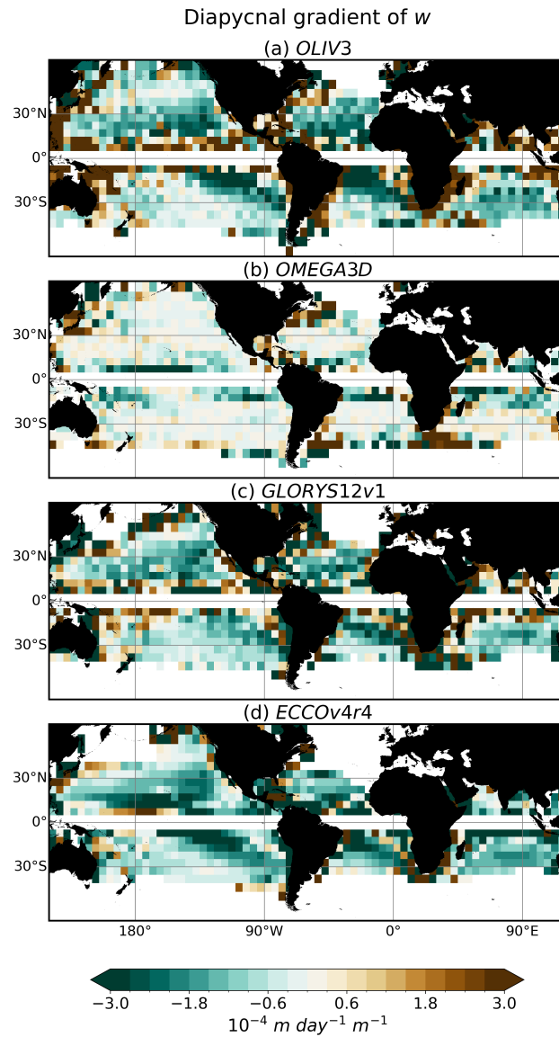
Figure A1. Vertical Diapycnal gradient of time-mean vertical velocity between the base of the maximum mixed layer depth and \sigma_{26.5} (Eq. 16) at 5^\circ \times 5^\circ spatial resolution, shown for: (a) OLIV3 , (b) OMEGA3D , (c) GLORYS12v1 , and (d) ECCOV4r4 . Negative values indicate a decrease in vertical velocity magnitude with depth, while positive values depict increasing magnitude with depth.
