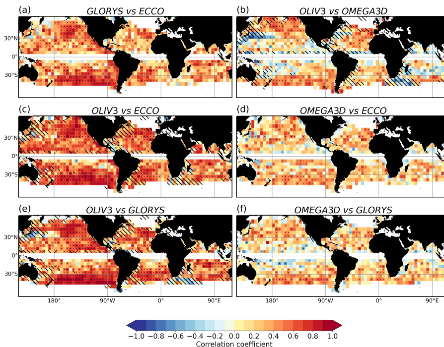
Figure 9. Correlation coefficient ( R ) between the vertical estimates from OLIV3, GLORYS12v1, ECCOv4r4, and OMEGA3D at \sigma 26 and 5^\circ \times 5^\circ resolution. Dotted squares indicate correlations significant at the 95% confidence level based on the Student t-test. Black hatching represents regions where correlation coefficient between OGCM w_{tot} and OGCM w_g is smaller than 0.5 (Fig. 4b).
