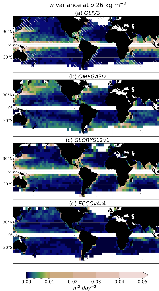
Figure 7. Annual variance (logarithmic scale) of vertical velocity at \sigma_{26} and 5^\circ \times 5^\circ spatial resolution for: (a) OLIV3, (b) OMEGA3D, (c) GLORYS12v1, and (d) ECCOv4r4. In panel (a), black-gray hatching represents regions where correlation coefficient between OGCM w_{tot} and OGCM w_g is smaller than 0.5 (Fig. 4b).
