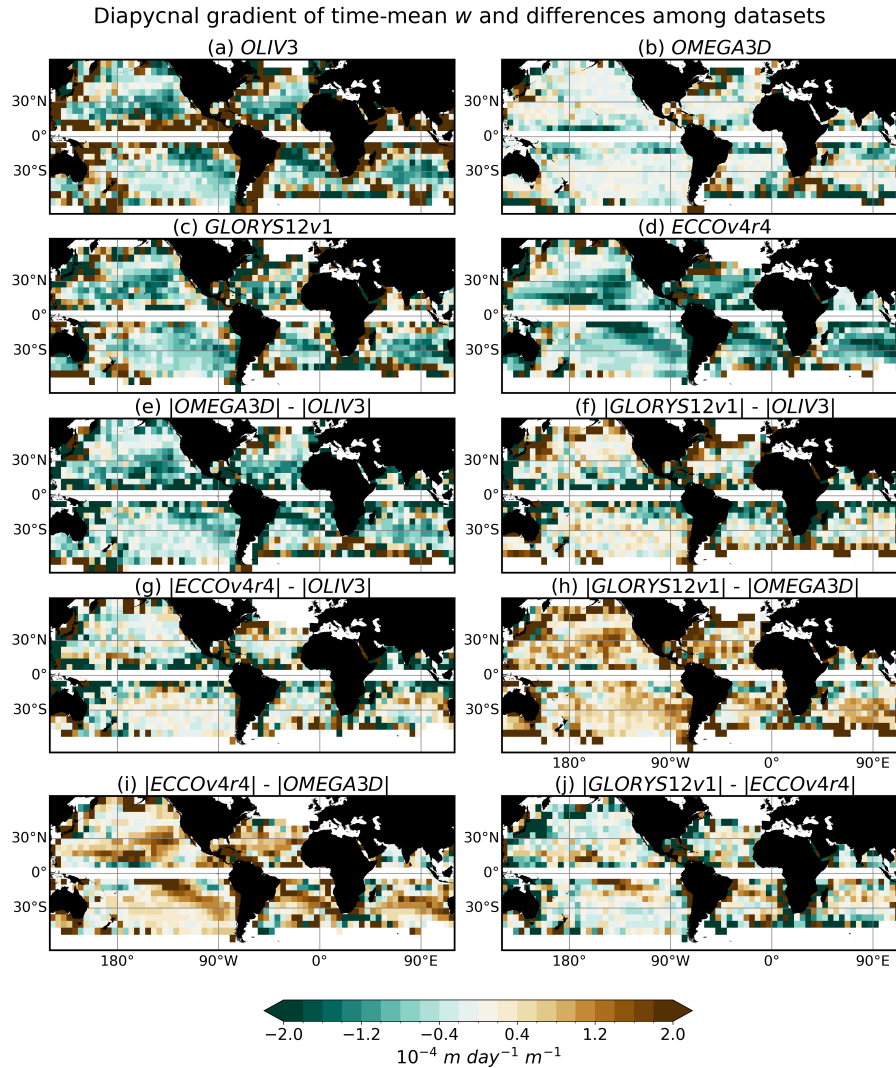
Figure 6. Vertical-Diapycnal gradient of time-mean vertical velocity between the base of the maximum mixed layer depth and \sigma_{27} (Eq. 16) at 5^\circ \times 5^\circ spatial resolution, shown for: (a) OLIV3, (b) OMEGA3D, (c) GLORYS12v1, and (d) ECCOV4r4. Negative values indicate a decrease in vertical velocity magnitude with depth, while positive values depict increasing magnitude with depth. (e-j) Differences between modules in the diapycnal gradient of time-mean vertical velocity for the various datasets.
