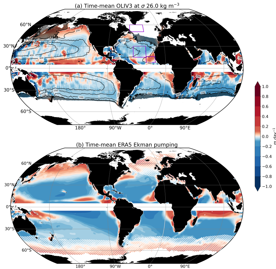
Figure 2. (a) OLIV3 time-mean (1993-2019) vertical velocity at \sigma_{26} (1993-2018)-26. The field has been smoothed with a 5^\circ running mean. Translucent black shading represents regions within the maximum mixed layer over the study period. The black contour lines represent the depth of the isopycnal surface in meters. Purple rectangles indicate the average regions for Fig. 3. (b) Time-mean Ekman pumping from ERA5. The field has been smoothed with a 5^\circ running mean. White hatching masks the regions above \sigma_{26} for comparison purposes.
