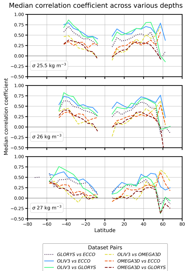
Figure 10. Median correlation coefficient ( R ) as a function of latitude for \sigma_{25.5} , \sigma_{26} , \sigma_{27} . The analysis includes only regions where the correlation between OGCM w_g and w_{tot} exceeds 0.5. Solid, dashed and dotted lines correspond to OLIV3, OMEGA3D intercomparisons, and reanalyses intercomparison respectively.
