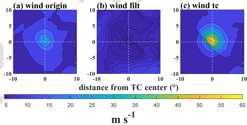
Figure 2. Plan views of surface wind speed ( \text{m s}^{-1} ) centered on Typhoon Francisco (20 October 2013) for (a) origin CCMP reanalysis dataset, (b) TC-wind filtered CCMP dataset and (c) IBTrACS TC-wind merged CCMP dataset.
