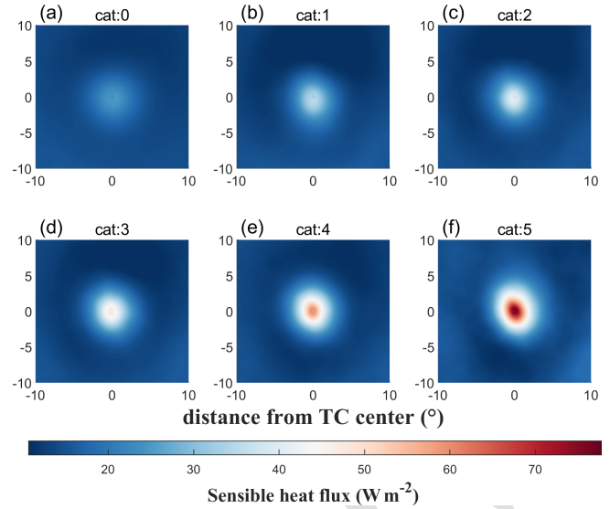
Figure 6. Plan views of composite surface sensible heat flux ( \text{W m}^{-2} ) centered on TC classified by TC intensity for (a) Cat 0, (b) Cat 1, (c) Cat 2, (d) Cat 3, (e) Cat 4, and (f) Cat 5.
