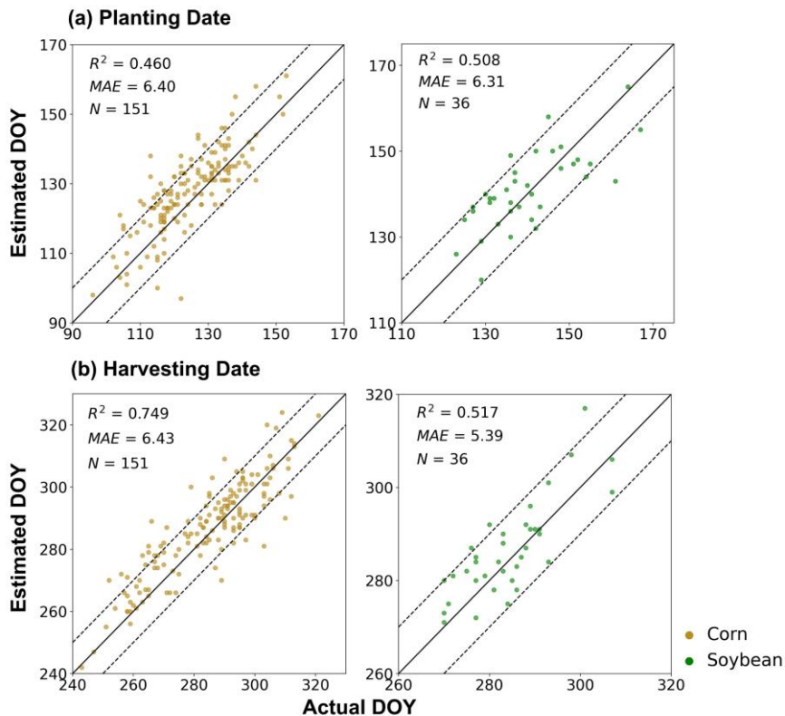
340 Figure 3. Field-level validation of estimated planting dates (a) and harvesting dates (b) for corn and soybean in the U.S. Midwest from 2016 to 2024. The solid line represents the 1:1 relationship between estimated and observed dates, and the dashed lines indicate \pm 10 days difference between estimated and observed ones.
