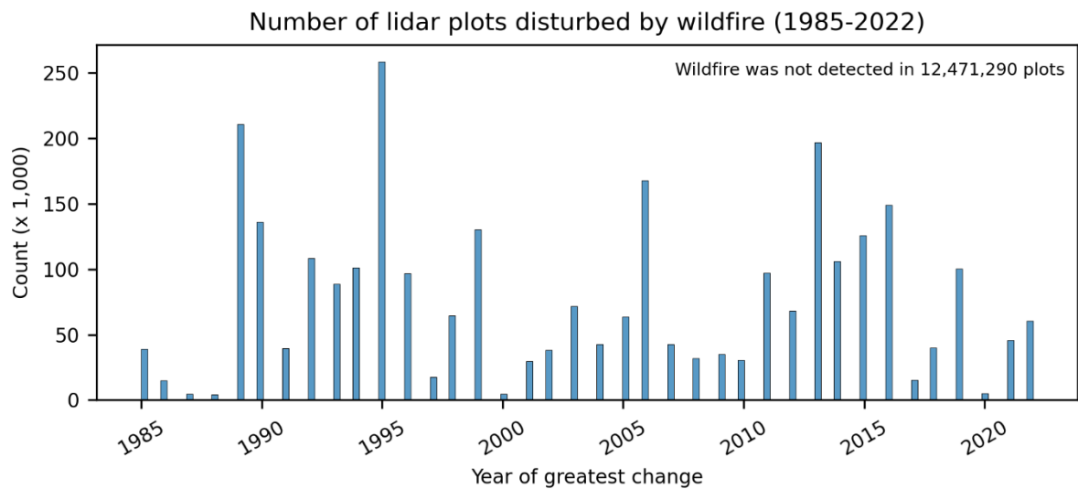
Figure 7. Comparison between lidar plots and multidecadal NTEMS satellite information products, including land cover class (excluding water) and number of plots disturbed by wildfire between 1985 and 2022 (Hermosilla et al., 2016; 2022).
