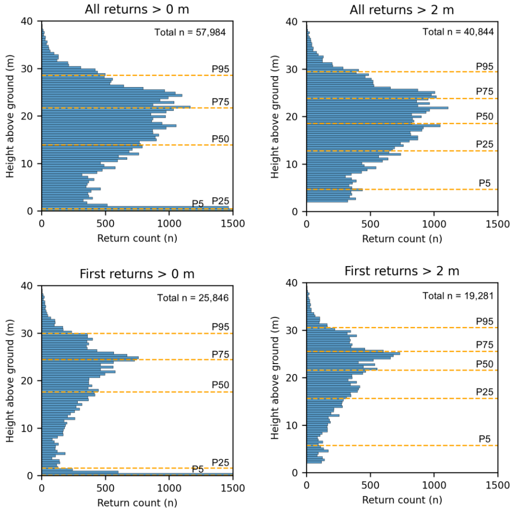
Figure 3. Comparison of vertical distributions of returns from four different processing groups for the same lidar plot: all returns above 0 m, all returns above 2 m, first returns above 0 m, and first returns above 2 m. P95 = 95 th height percentile, P75 = 75 th height percentile, and so on. The plot is located along the Prophet River in northern British Columbia (58° 17' 19" N, 122° 52' 30" W).
