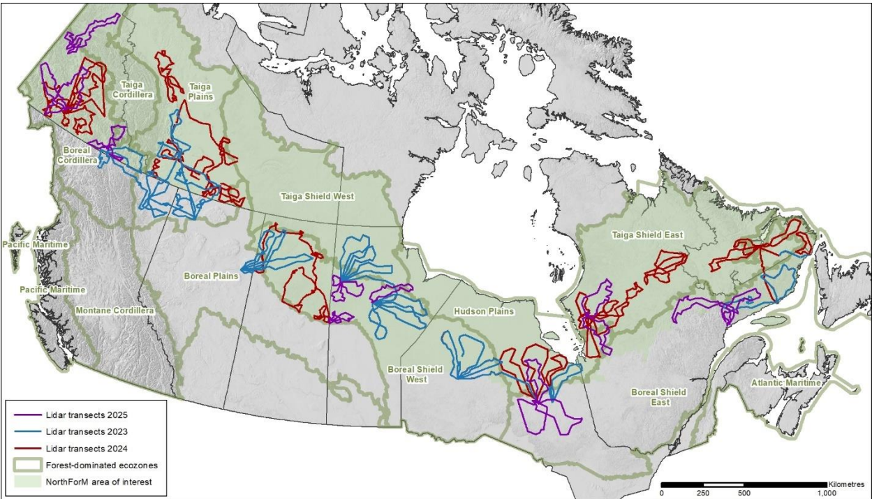
Figure 1. Airborne laser scanning (ALS) transects flown in 2023 (~20,000km), 2024 (~23,000 km), and 2025 (~12,000 km). The Northern Forest Mapping (NorthForM) acquisitions were largely focused on northern ecozones to improve mapping in unmanaged forests.
