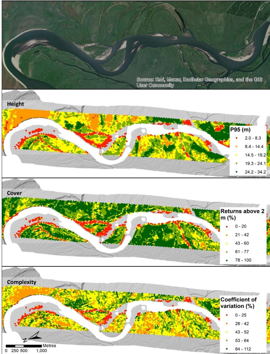
Figure 4. Examples of lidar plot metrics, including: canopy height based on the 95th height percentile of first returns greater than 2 m; canopy cover based on the proportion of first returns greater than 2 m; and canopy complexity based on the coefficient of variation of first returns heights greater than 2m. The image in the top panel extends beyond the ALS swath for added landscape context. The digital terrain model hillshade was derived from ALS returns with scan angles in excess of 20 degrees, while lidar plots are limited to returns with scan angles less than or equal to 20 degrees (Table S1). Data are located along the Liard River in northern British Columbia (59° 53' 22" N, 128° 19' 3" W).
