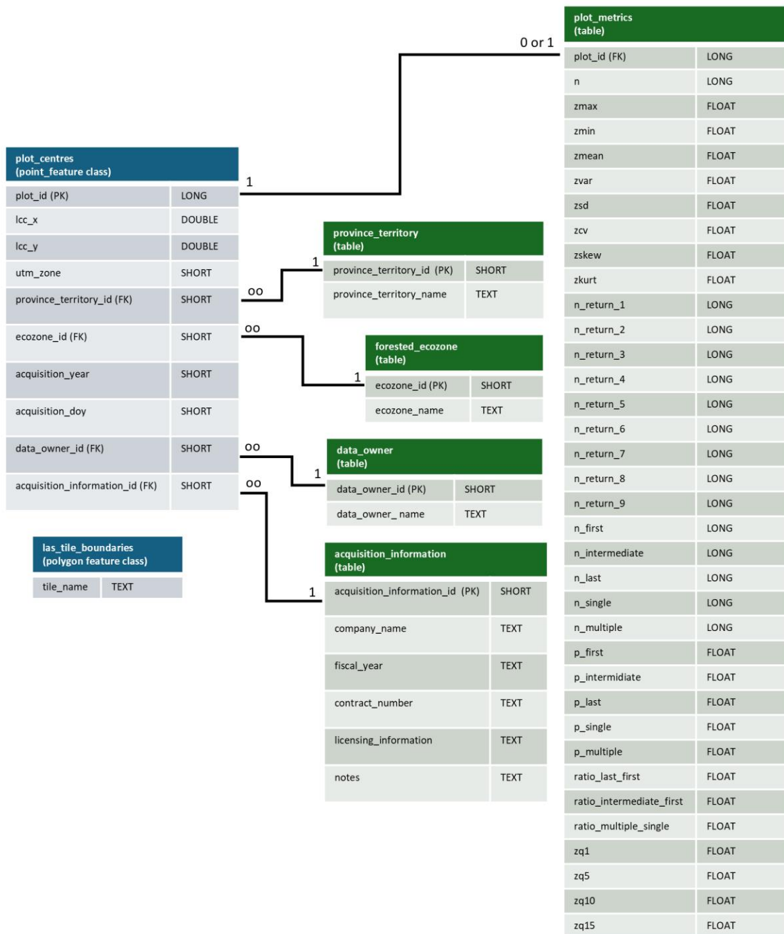
Figure 2. Entity relationship diagram describing the structure of the lidar plots database. In total, the plot metrics table includes 369 point cloud metrics for each lidar plot, with an abridged version of the database available including a subset of 40 metrics.
