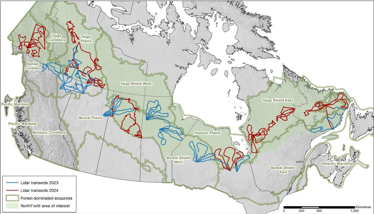
Figure 1. Airborne laser scanning (ALS) transects flown in 2023 (~20,000km) and 2024 (~23,000 km). The Northern Forest Mapping (NorthForM) acquisitions are limited to northern ecozones to improve mapping in unmanaged forests.
