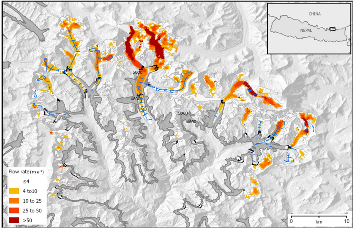
450 Figure 14 | Flow rate (after Gardner, Fahnestock et al. 2022) (colour scale) and extent (white polygons (RGI Consortium 2017)) of glaciers in this study, with the 4800-5000 m altitude band highlighted (grey polygon and black lines where this crosses glaciers) (after Shean 2017). Location of survey data is shown in blue. Background: shaded-relief topography (Jarvis, Reuter et al. 2008, Shean 2017) and glacier extents (RGI Consortium 2017) (white polygons).
