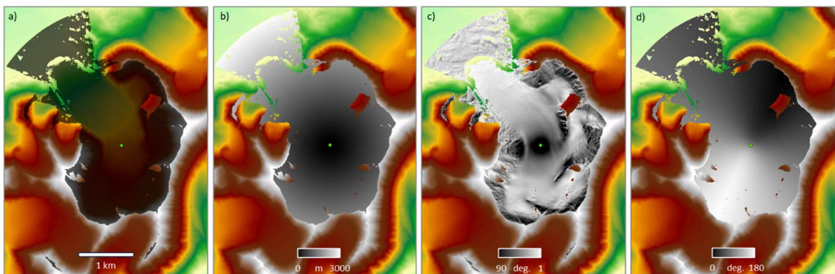
250 Figure 5 | Terrain analysis for a point (green dot in centre) along the survey flightpath in Figure 4b, including: a) the line of sight viewshed (dark grey mask), and within this viewshed; b) the distance to terrain (greyscale); c) incidence angle of the wavefront meeting the surface (greyscale); and d) directivity angle (flightpath orientation relative to the surface) (greyscale). The background colour scale shows topography as in Figure 4b.
