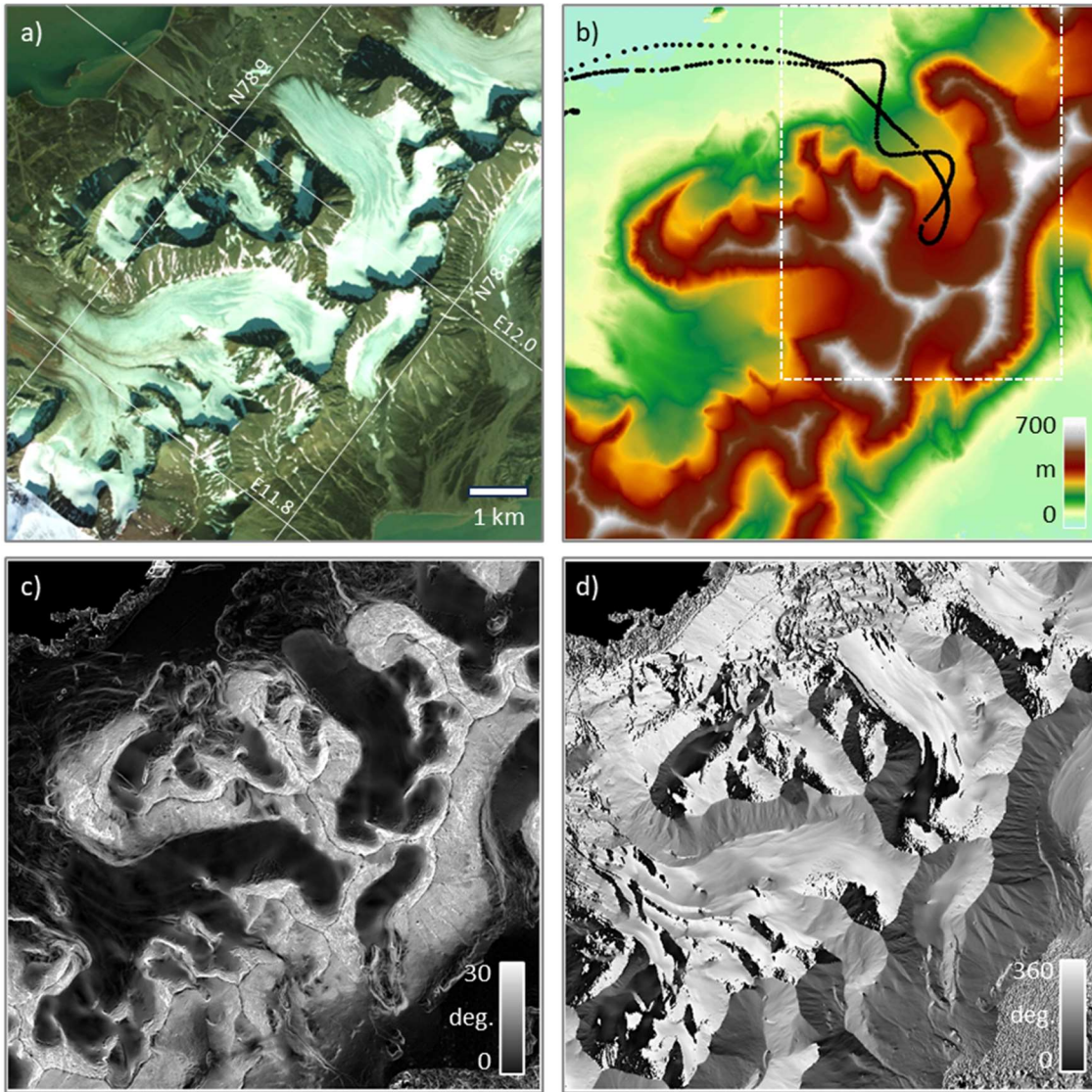
245 Figure 4 | Example of the terrain properties of a glacial catchment (a) that are used to model clutter, including: b) elevation; c) slope; and d) aspect. The black dotted line in (b) shows a survey flightpath through the landscape (Pritchard, King et al. 2020), the white box shows the area covered in Figure 5.
