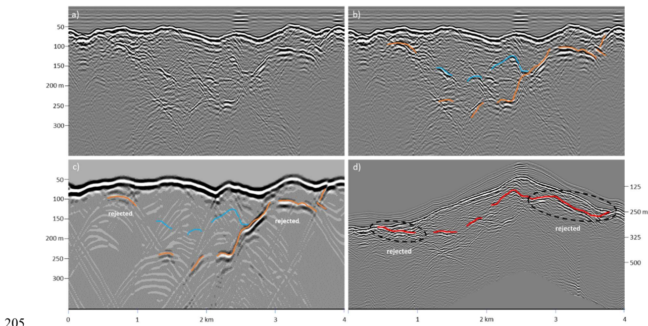
205 Figure 3 | Testing and correction of a manually picked glacier bed using output from the clutter model. a) A survey radargram from Nuptse Glacier, Nepal, with a characteristically complicated set of bright, semi-continuous linear features appearing at various ranges beyond the glacier surface; b) plausible bed picks (orange and blue lines) with ambiguity where they overlap; c) the clutter model for this survey showing that the orange lines correspond to terrain clutter but the blue lines do not, suggesting that the blue lines represent the bed; d) the 210 terrain-corrected radargram with the initial bed pick bed (red lines), highlighting the sections that were subsequently rejected following the clutter test (panel c) (panel d vertical scale differs from other panels) (see also Figure 6).
