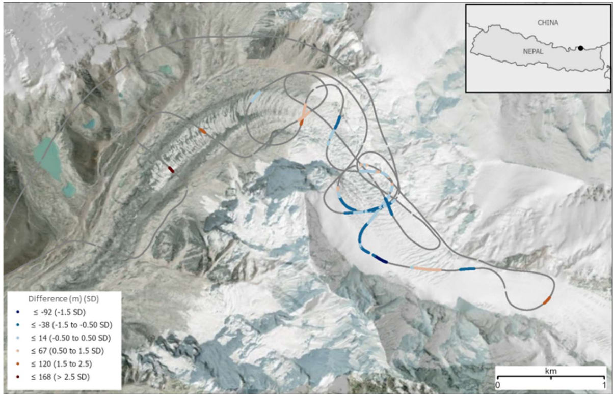
Figure 12 | Surveyed thickness minus modelled Millan thickness (Millan, Mouginot et al. 2022), in metres and multiples of standard deviations (SD) of difference from the mean difference of -12 m for Khumbu Glacier. Negative (blue) values indicate that the model grid is too thick, positive (brown) values that it is too thin. The largest thin biases in this model tend to correspond with the thickest ice and the largest model thick biases tend to correspond with the thinnest ice (cf. Figure 8). Background: shaded-relief topography (Jarvis, Reuter et al. 2008, Shean 2017) overlaid on satellite imagery (Earthstar Geographics Undated).
