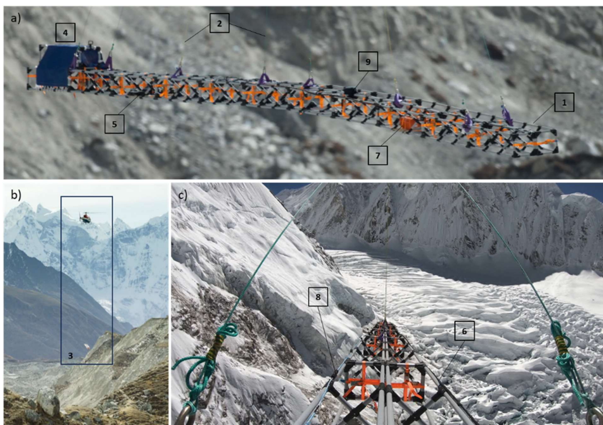
110 Figure 1 | The radar frame consisting of lightweight fibreglass modules strapped together (1), with rope lines (2) 115 to suspend the system under the helicopter (3), a tail (4) to prevent ‘weathercocking’, a pulse transmitter (5) and corresponding, resistively loaded transmit dipole antenna (6), receiver (7) and receive antenna (8) and GPS (9) (Pritchard, King et al. 2020). Panel (c) shows the system approaching the icefall on Khumbu Glacier (Figure 2), with multiple potential sources of radar clutter notably from the surrounding mountains and crevasse walls. Photo credits: Hamish Pritchard.
