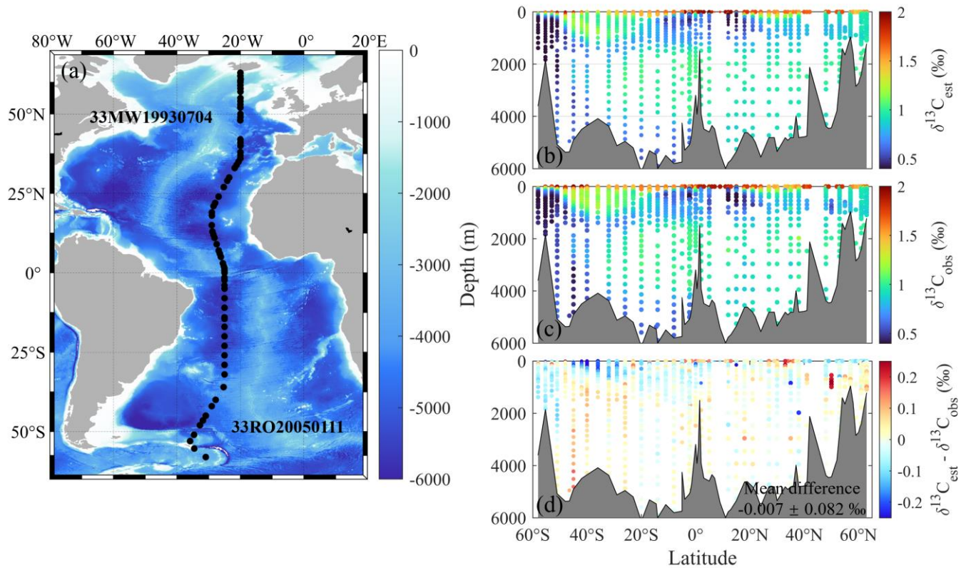
320 Figure 4. (a) Station locations of the independent test cruises 33MW19930704 and 33RO20050111; Depth profile of (b) model-estimated ( \delta^{13}\text{C}_{\text{est}} ) and (c) in-situ observed ( \delta^{13}\text{C}_{\text{obs}} ) \delta^{13}\text{C}_{\text{DIC}} along cruises 33MW19930704 and 33RO20050111, and (d) spatial distribution of mean bias error (MBE) between \delta^{13}\text{C}_{\text{est}} and \delta^{13}\text{C}_{\text{obs}} for the two cruises. Positive MBE values (red) denote product
