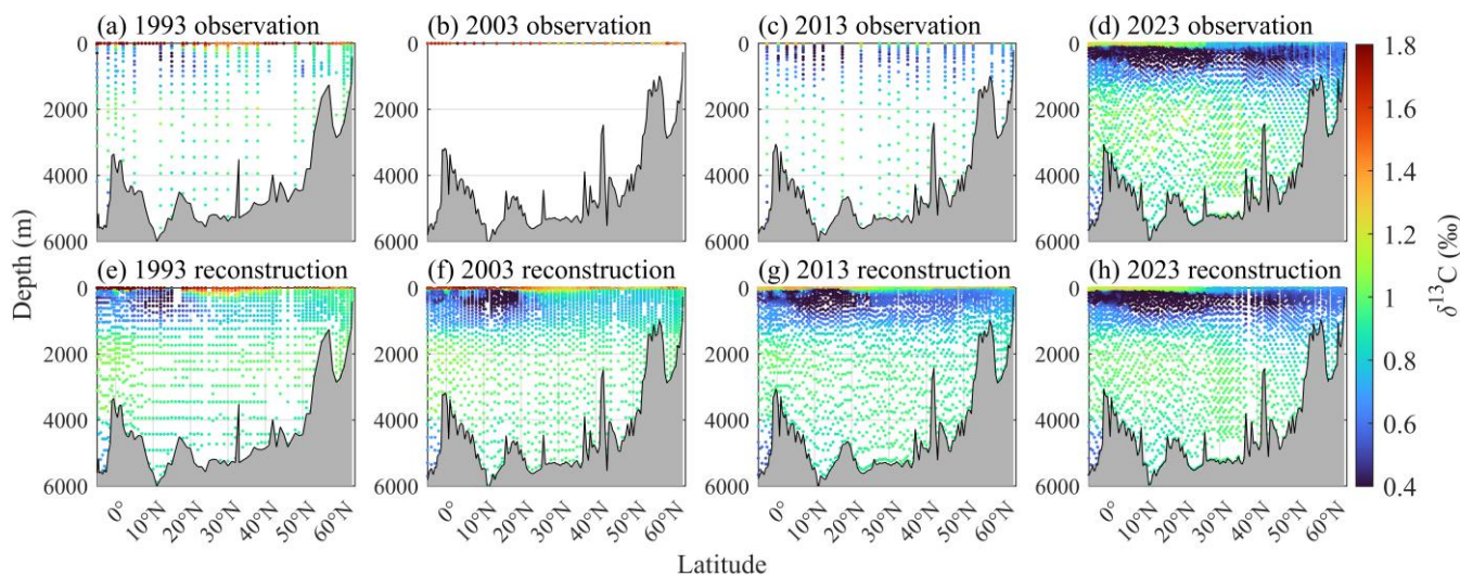
515 Figure 9. Enhancement of spatial resolution for \delta^{13}\text{C}_{\text{DIC}} through GPR model reconstruction along North Atlantic A16N transect. Top panels (a–d) presents in-situ observed \delta^{13}\text{C}_{\text{DIC}} from cruises in (a) 1993 ( n = 493 ), (b) 2003 (surface-only, n = 38 ), (c) 2013 ( n = 473 ), and (d) 2023 ( n = 3,460 ). Bottom panels (e–h) shows corresponding reconstructed \delta^{13}\text{C}_{\text{DIC}} with systematic filling of spatial gaps: (e) the
