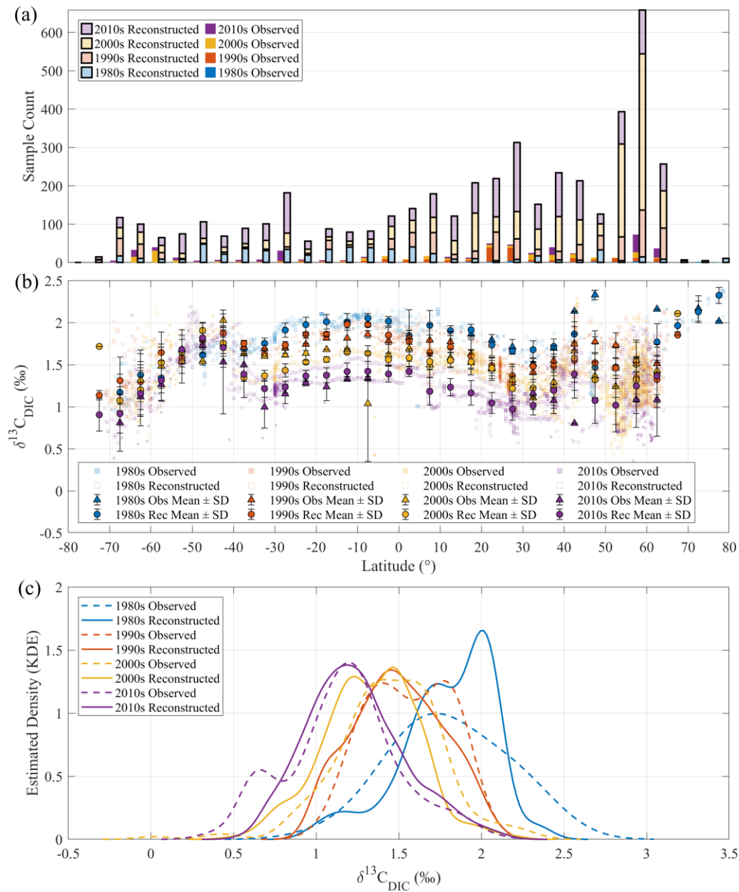
475 Figure 8. Surface distribution of observed and reconstructed \delta^{13}\text{C}_{\text{DIC}} in the Atlantic Ocean across four decades. (a) Number of observed and reconstructed \delta^{13}\text{C}_{\text{DIC}} samples within each 5^\circ latitude band for the 1980s, 1990s, 2000s, and 2010s. For each latitude band, stacked bars represent decadal sample counts. Solid (opaque) bars indicate observations, and semi-transparent bars with black outlines indicate corresponding reconstructions. (b) Surface \delta^{13}\text{C}_{\text{DIC}} distributions (depth \leq 10 m) along latitude for the 1980s, 1990s, 2000s, and 2010s. (c) Kernel Density Estimate (KDE) plot showing the estimated density of \delta^{13}\text{C}_{\text{DIC}} (‰) for the 1980s, 1990s, 2000s, and 2010s.
