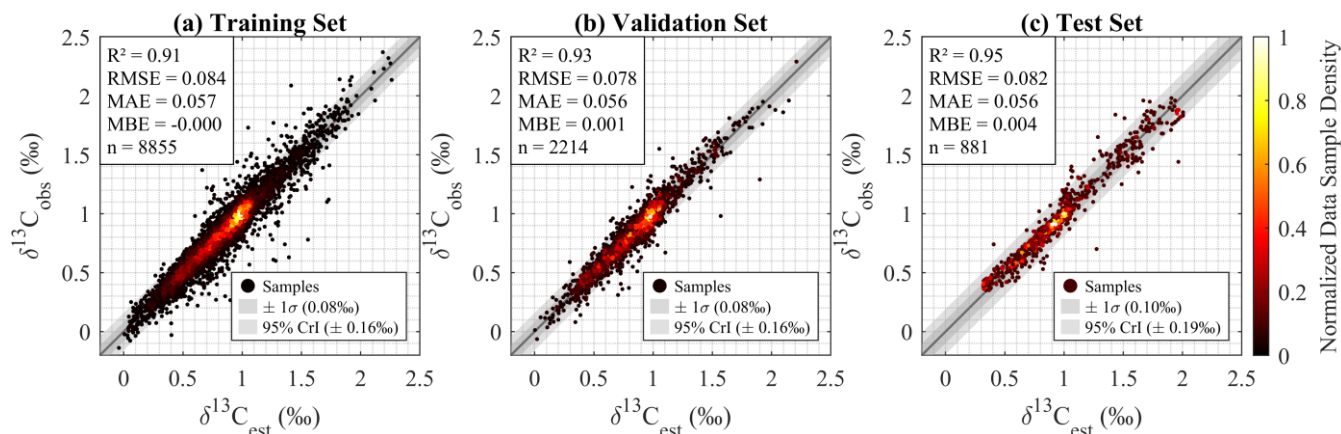
300 Figure 3. Regression model evaluation for \delta^{13}\text{C}_{\text{DIC}} reconstruction: Density scatter plots comparing model-estimated ( \delta^{13}\text{C}_{\text{est}} ) versus observed ( \delta^{13}\text{C}_{\text{obs}} ) \delta^{13}\text{C}_{\text{DIC}} values during (a) training (80 % samples from 35 cruises, with 10-fold cross-validation), (b) validation (20 % samples from 35 cruises), and (c) independent testing (samples from cruises 33RO20050111 and 33MW19930704). Statistical metrics include coefficient of determination ( R^2 ), root-mean-square error (RMSE), mean absolute error (MAE), mean bias error (MBE), and sample size (n). Color indicates normalized local data point density within 2D bins: the plot area is divided into a 100 \times 100 grid, raw density is the number of points per bin, and values are normalized to 0~1 (0 = sparsest, 1 = densest). Shaded bands represent predictive uncertainty, with the darker grey band showing one standard deviation ( \pm 1\sigma ) and the lighter grey band showing the 95 % credible interval (CrI).
