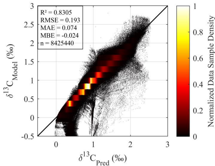
Figure A5. Density scatter plot of native model versus reconstructed \delta^{13}\text{C}_{\text{DIC}} values for the full Atlantic domain prediction phase.
