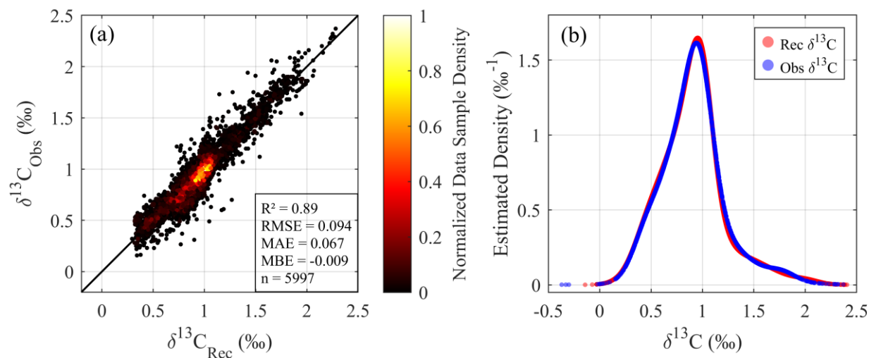
415 Figure 5. Comparison of observed and reconstructed \delta^{13}\text{C}_{\text{DIC}} values derived from the GLODAPv2.2023 dataset. (a) Density scatter plot of observed versus reconstructed \delta^{13}\text{C}_{\text{DIC}} values, using only the intersection of data points with acceptable quality available in both observed and reconstructed datasets ( n = 5997 ). (b) Gaussian kernel density estimations (KDEs) for a comprehensive evaluation of observed and reconstructed \delta^{13}\text{C}_{\text{DIC}} values. In panel b, the blue curve represents all acceptable \delta^{13}\text{C}_{\text{DIC}} observations ( n = 8941 ), while the red curve indicates all acceptable reconstructed \delta^{13}\text{C}_{\text{DIC}} values ( n = 68,435 ), generated by GPR model trained on the GLODAPv2.2023 dataset. The KDEs reveal the overall distribution shape, highlight differences in peak height and spread, and provide a smooth, continuous representation of probability density.
