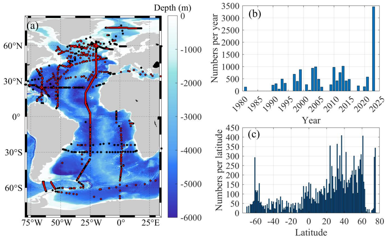
120 Figure 1. Overview of the collected \delta^{13}\text{C}_{\text{DIC}} data. (a) Map of all stations with \delta^{13}\text{C}_{\text{DIC}} data in the Atlantic Ocean, with stations containing samples deeper than 2,000 m highlighted in red. (b) Temporal distribution of \delta^{13}\text{C}_{\text{DIC}} data, organized by year of collection. (c) Total number of \delta^{13}\text{C}_{\text{DIC}} samples aggregated by each degree of latitude.
