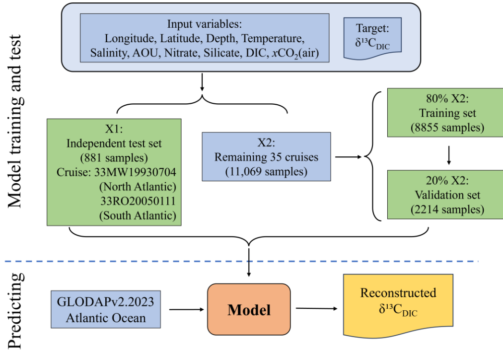
230 Figure 2. A flowchart illustrating the machine-learning regression model for reconstructing the \delta^{13}\text{C}_{\text{DIC}} product. The blue boxes represent the input, and the yellow box represents output datasets, while the green boxes depict the model training, validation, and independent testing processes. The orange box indicates the final trained model used for prediction.
