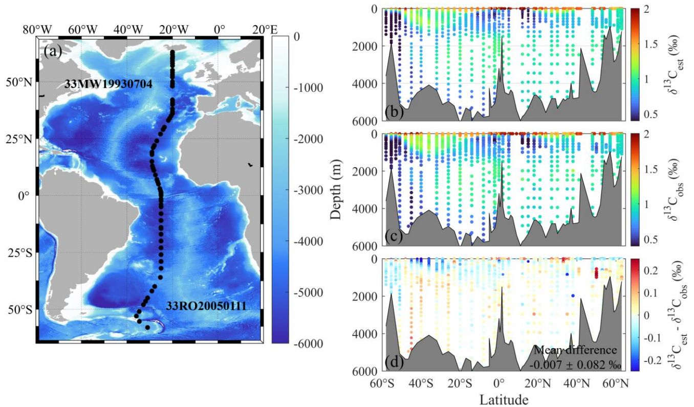
Figure 4. (a) Station locations of the independent test cruises 33MW19930704 and 33RO20050111; Depth profile of (b) model-estimated ( \delta^{13}\text{C}_{\text{est}} ) and (c) in-situ observed ( \delta^{13}\text{C}_{\text{obs}} ) \delta^{13}\text{C}_{\text{DIC}} along cruises 33MW19930704 and 33RO20050111, and (d) spatial distribution of mean bias error (MBE) between \delta^{13}\text{C}_{\text{est}} and \delta^{13}\text{C}_{\text{obs}} for the two cruises. Positive MBE values (red) denote product
