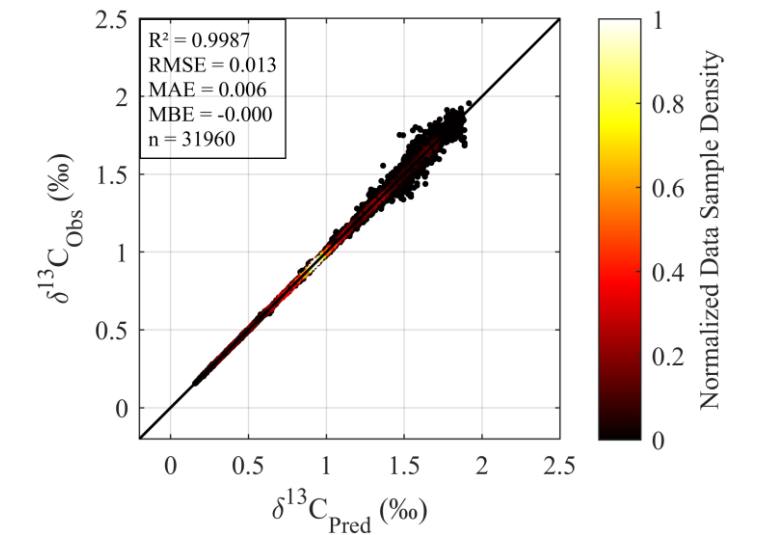
Figure A2 Density scatter plot comparing numerical model outputs \delta^{13}\text{C}_{\text{DIC}} ( \delta^{13}\text{C}_{\text{Obs}} ) versus predicted \delta^{13}\text{C}_{\text{DIC}} ( \delta^{13}\text{C}_{\text{Pred}} ) values.
