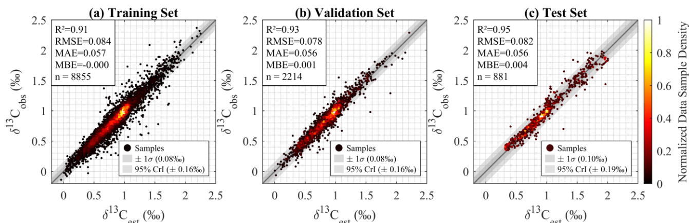
305 Figure 3. Regression model evaluation for \delta^{13}\text{C}_{\text{DIC}} reconstruction: Density scatter plots comparing model-estimated ( \delta^{13}\text{C}_{\text{est}} ) versus in- site -observed ( \delta^{13}\text{C}_{\text{obs}} ) \delta^{13}\text{C}_{\text{DIC}} values during (a) training (80 % samples from 35 cruises, with 10-fold cross-validation), (b) validation (20 % samples from 35 cruises), and (c) independent testing (samples from cruises 33RO20050111 and 33MW19930704). Statistical metrics include coefficient of determination ( R^2 ), root-mean-square error (RMSE), mean absolute error (MAE), mean bias error (MBE), and sample size ( n ). Color indicates normalized local data point density within 2D bins: the plot area is divided into a 100 \times 100 grid, raw density is the number of points per bin, and values are normalized to 0~1 (0 = sparsest, 1 = densest). Shaded bands represent predictive uncertainty, with the darker grey-gray band showing one standard deviation ( \pm 1\sigma ) and the lighter graygrey band showing the 95 % credible interval (CrI).
