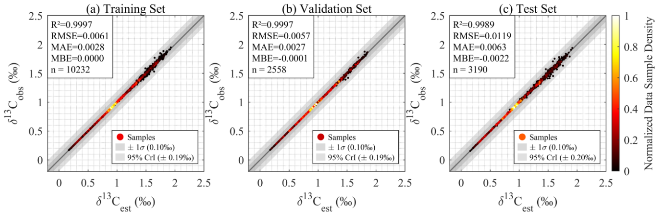
675 Figure A1. GPR model evaluation for numerical model \delta^{13}\text{C}_{\text{DIC}} reconstruction: Density scatter plots comparing GPR model-estimated ( \delta^{13}\text{C}_{\text{est}} ) versus numerical model outputs \delta^{13}\text{C}_{\text{DIC}} ( \delta^{13}\text{C}_{\text{obs}} ) values during (a) training, (b) validation, and (c) independent testing.
