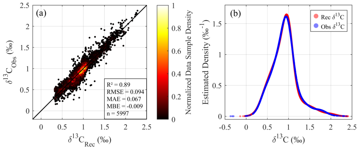
420 Figure 5. Comparison of observed and reconstructed \delta^{13}\text{C}_{\text{DIC}} values derived from the GLODAPv2.2023 dataset. (a) Density scatter plot of observed versus reconstructed \delta^{13}\text{C}_{\text{DIC}} values, using only the intersection of data points with acceptable quality available in both 425 observed and reconstructed datasets ( N_{\text{int}} = 5997 ). (b) Gaussian kernel density estimations (KDEs) for a comprehensive evaluation of observed and reconstructed \delta^{13}\text{C}_{\text{DIC}} values. In panel b, the blue curve represents all acceptable \delta^{13}\text{C}_{\text{DIC}} observations ( n_{\text{N}}=8941 ), while the red curve indicates all acceptable reconstructed \delta^{13}\text{C}_{\text{DIC}} values ( N_{\text{int}}=68,435 ), generated by GPR model trained on the GLODAPv2.2023 dataset. The KDEs reveal the overall distribution shape, highlight differences in peak height and spread, and provide a smooth, continuous representation of probability density.
