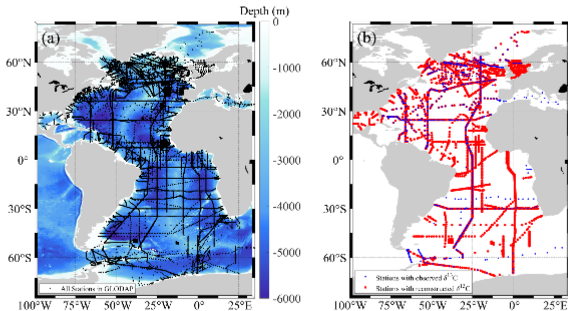
435 Figure 6. Station maps for the GLODAPv2.2023 Atlantic Ocean dataset. (a) Locations of all stations included in the dataset. (b) Stations with observed (blue dots) and reconstructed (red dots) \delta^{13}\text{C}_{\text{DIC}} .
