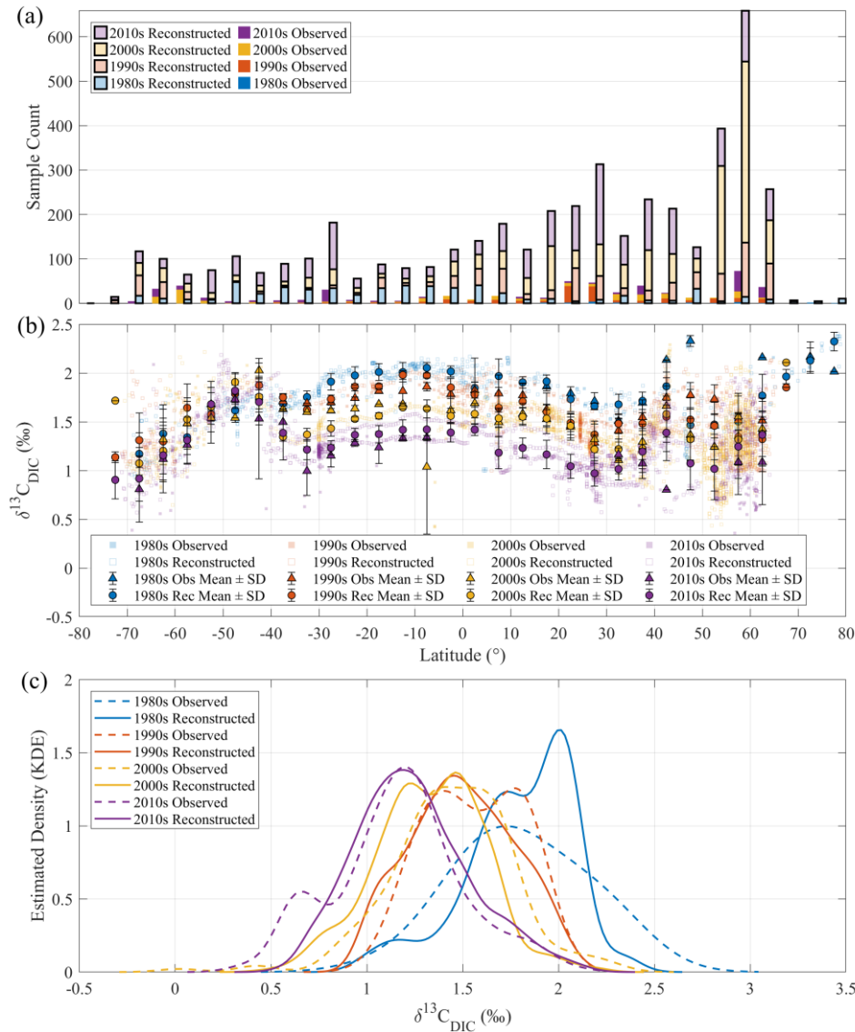
495 Figure 8. Surface distribution of observed and reconstructed \delta^{13}\text{C}_{\text{DIC}} in the Atlantic Ocean across four decades. (a) Number of of observed and reconstructed \delta^{13}\text{C}_{\text{DIC}} samples within each 5^\circ latitude band for the 1980s, 1990s, 2000s, and 2010s. For each latitude band, stacked bars represent decadal sample counts. Solid (opaque) bars indicate observations, and semi-transparent bars with black outlines indicate corresponding reconstructions. (b) Surface \delta^{13}\text{C}_{\text{DIC}} distributions (depth \leq 10 m) along latitude for the 1980s, 1990s, 2000s, and 2010s. Colored scatter points indicate individual \delta^{13}\text{C}_{\text{DIC}} values from observations (circles) and reconstructions (dots), while the black 500 markers with corresponding face color and error bars represent the mean \pm standard deviation of \delta^{13}\text{C}_{\text{DIC}} within each 5^\circ latitude bin, triangles for observed data and diamonds for reconstructed values. (c) Gaussian kernel density estimates (KDEs) of surface \delta^{13}\text{C}_{\text{DIC}} for each decade
