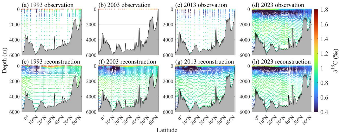
520 Figure 9. Enhancement of spatial resolution for \delta^{13}\text{C}_{\text{DIC}} through GPR model reconstruction along North Atlantic section–A16N transect . Top panels (a–d) presents in-situ observed \delta^{13}\text{C}_{\text{DIC}} from cruises in (a) 1993 ( n = \del{526493}), (b) 2003 (surface-only, n = 38 ), (c) 2013
