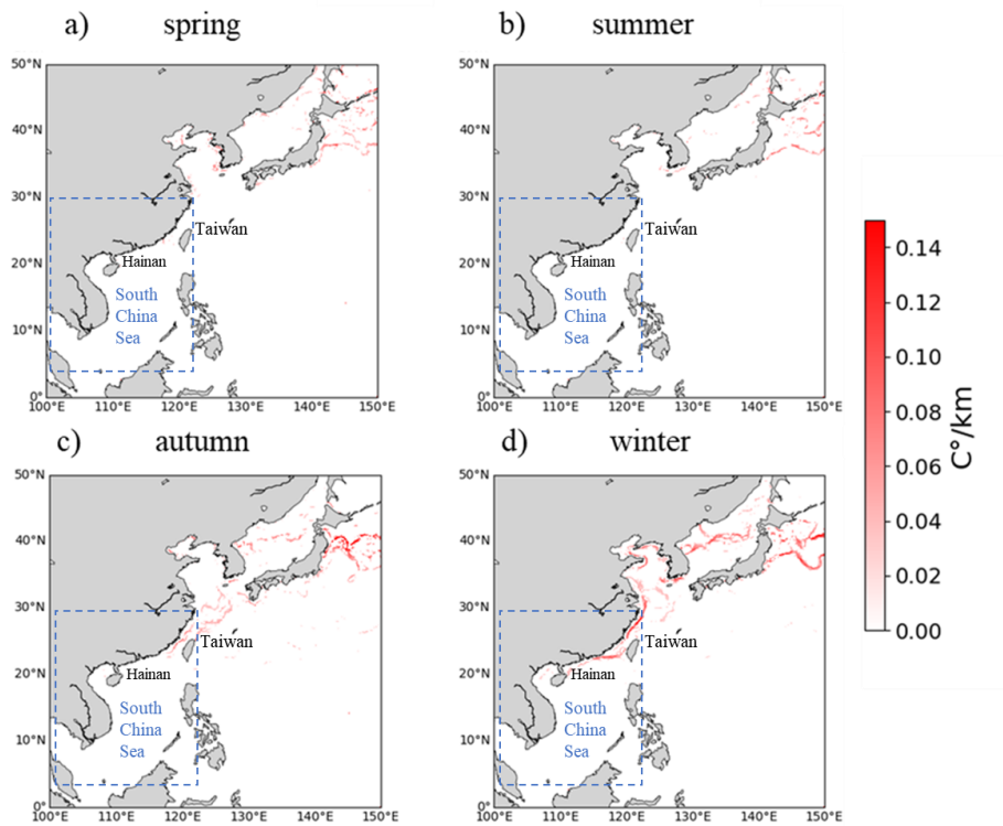
Figure 9. Seasonal spatial-temporal distribution map of ocean fronts in 2023 (The blue dashed box indicates the South China Sea)
