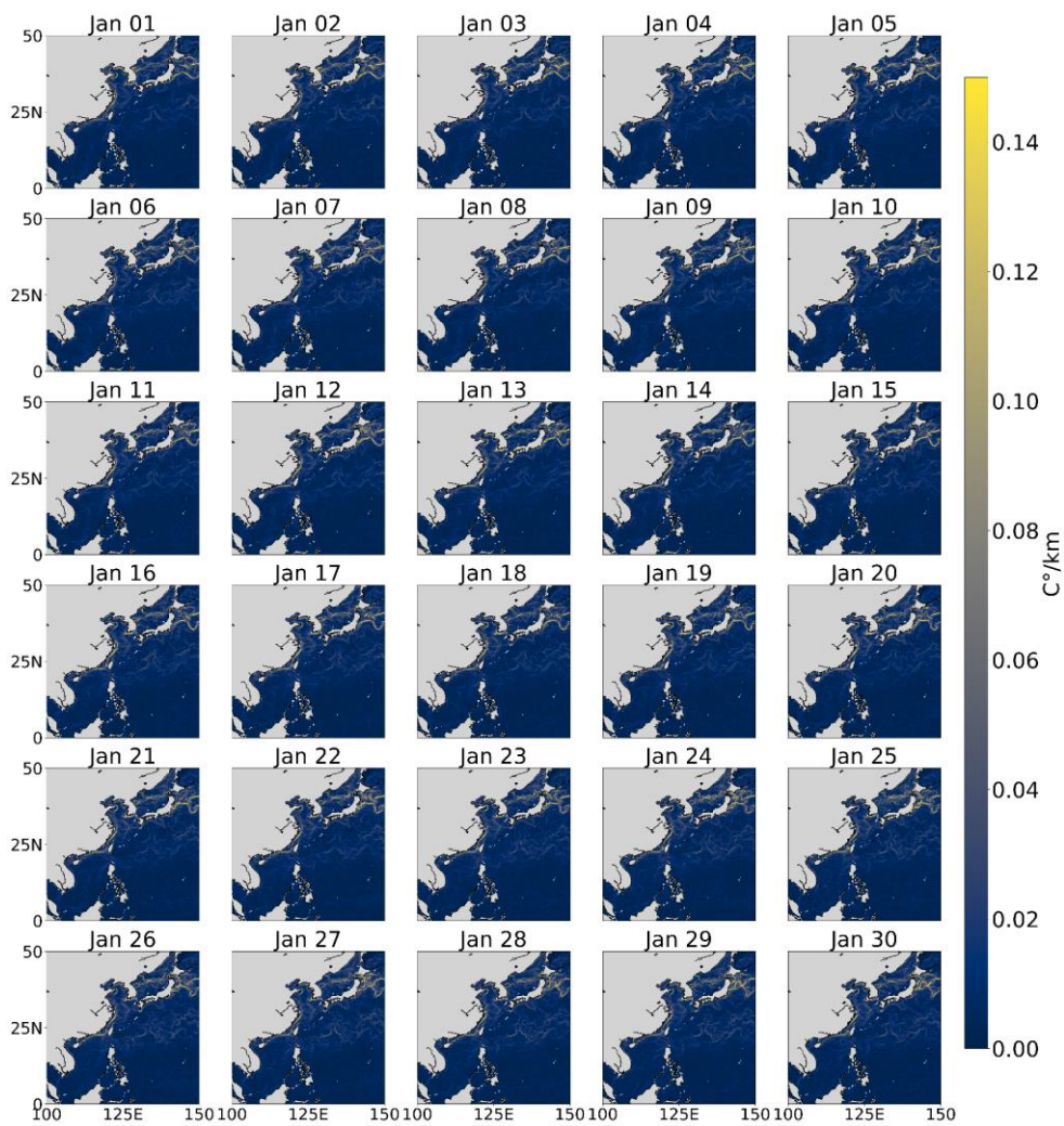
Figure 5. Gradient image of ocean fronts Ocean-Front (Time sSeries in January 2023)
