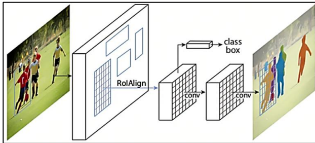
Figure 2. Mask R-CNN network architecture (He et al., 2017)
