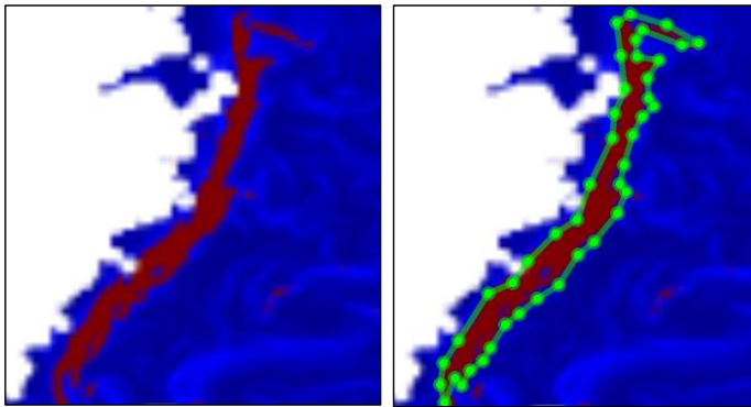
240 Figure 6. Comparison of the original temperature gradient image and its manual annotation for ocean fronts.
