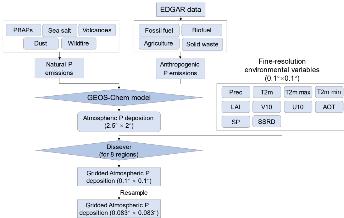
Figure 3. Workflow of developing atmospheric phosphorus input data. Where PBAPs represent Primary Biological Aerosol Particles. Prec refers to precipitation. T2m indicates the 2-meter air temperature, while T2m max and T2m min refer to the maximum and minimum air temperatures at 2-meter height. U10 and V10 denote the eastward and northward wind speeds at 10-meter height, respectively. AOT stands for Aerosol Optical Thickness. SP represents Surface Pressure, and SSRD refers to Surface Solar Radiation Downwards.
