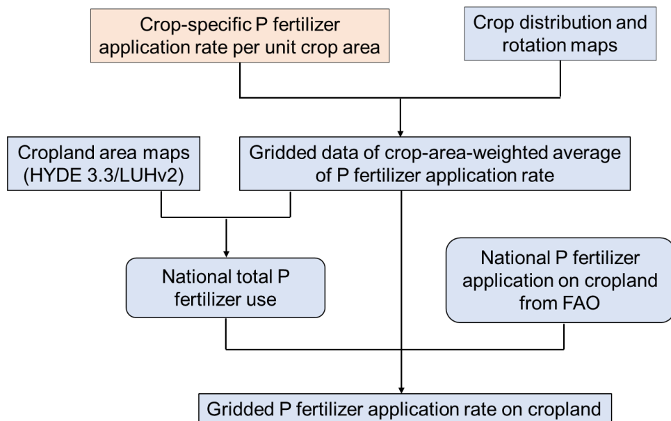
Figure 1. Workflow of developing data for phosphorus fertilizer application on
