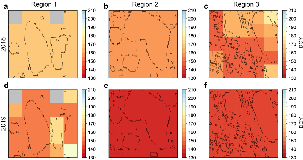
374 375 Figure 7. The lake ice break-up dates in 2019 (d–f) were generally earlier than those in 2018 (a–c) across the three selected regions in the 376 ACP (Fig. 1). Each subplot shows a 5 × 5 km area where water bodies are delineated by black lines. The phenology dates are calculated 377 based on 1-km S1 ice fraction data, and the color of each 1-km grid cell indicates the break-up date in day of year (DOY).
