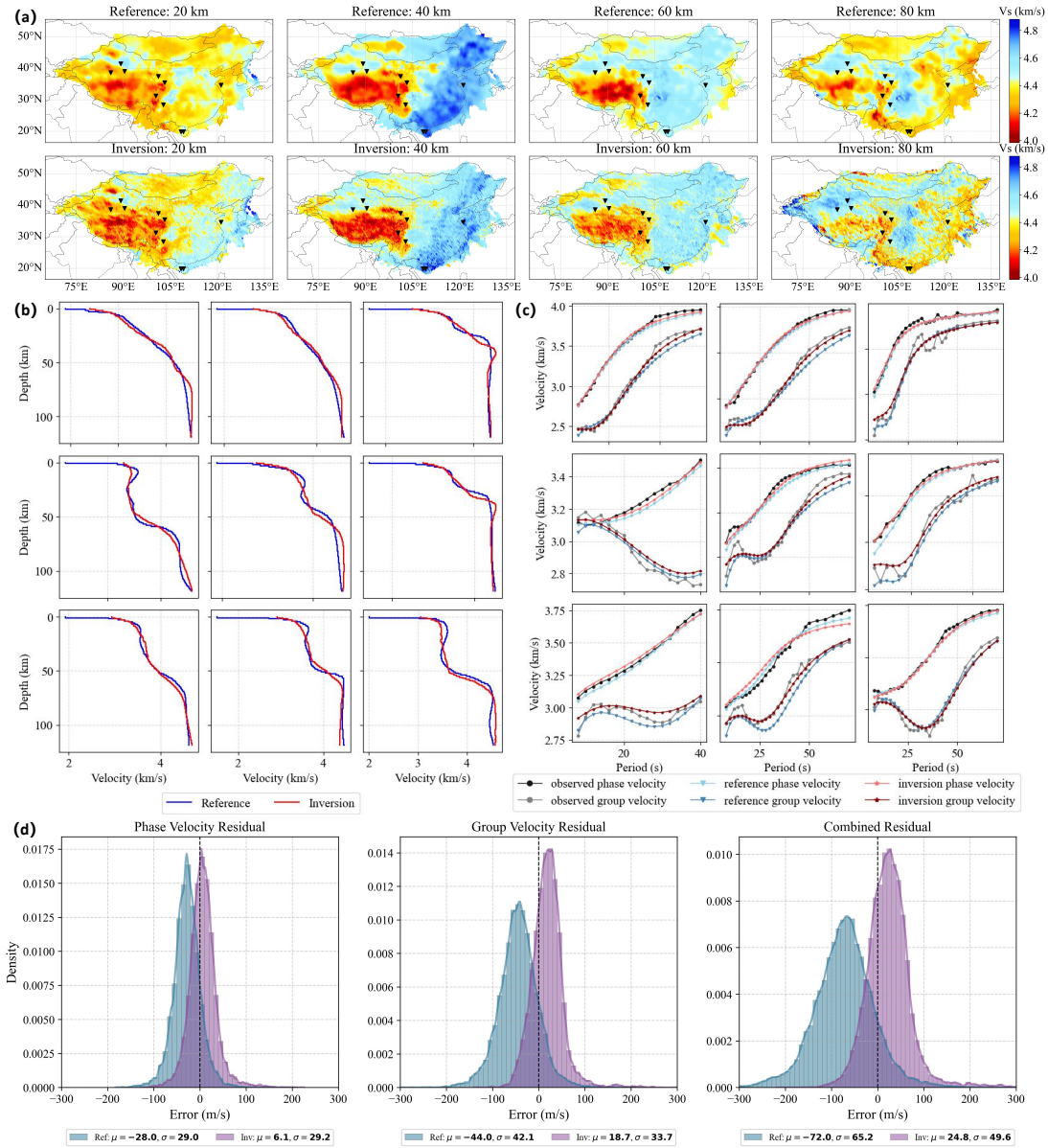
Figure 13. Generalization performance on real-world CSRM data from the OpenSWI-real dataset. (a) Reference (Xiao et al., 2024) and predicted v_s slices at depths of 20, 40, 60, and 80 km. (b) 1-D v_s profiles at nine representative locations, with reference and predicted models shown in blue and red, respectively. (c) Comparison of phase and group velocity dispersion curves, including observed curves (black), synthetic curves from the reference model (blue for group velocity, light blue for phase velocity), and from the predicted model (red for group velocity, pink for phase velocity). (d) Error distributions of phase velocity (left), group velocity (middle), and their sum (right) with respect to observed curves, based on synthetic dispersion curves from the reference (blue) and predicted (purple) models.
