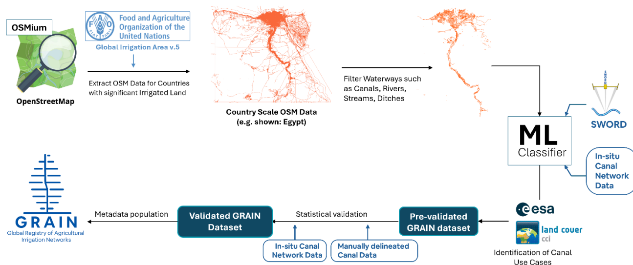
Figure 3. Workflow for the development of the GRAIN dataset. OSM data are extracted for countries with significant irrigated land (based on FAO Global Irrigation Area v.5), filtered for relevant hydrographic features, and classified using a machine learning pipeline informed by in-situ canal datasets, SWORD river networks, and ESA CCI land cover data. The resulting canal network undergoes validation and metadata population to produce the final GRAIN dataset.
