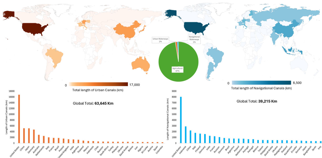
Figure A. 3. Distribution of [left] Urban Canals and [right] Navigational Waterways, with list of top 30 countries. Pie chart in the centre shows the proportion of urban (2%) and navigational canals (1%) to agricultural canals (97%).
