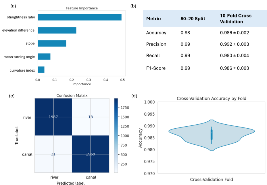
675 Figure A. 1. Random Forest classification model training performance. (a) Feature importance bar plot showing the relative contribution of each engineered variable to the model, (b) Macro averaged Accuracy, precision, recall, and F1-Scores for 80-20 train-test and 10-fold cross validation test, (c) Confusion matrix for 80-20 train-test, illustrating true and false positives and negatives. (d) Violin plot showcasing the spread of the accuracy scores for the 10-fold cross validation test.
