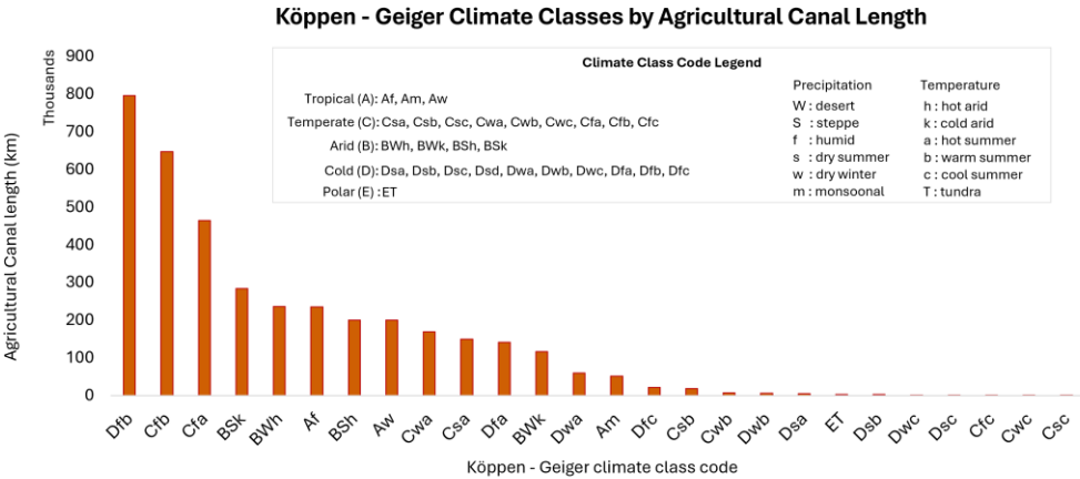
Figure 8. Distribution of agricultural irrigation canals in GRIN by Köppen-Geiger Climate zones. Cold and Temperate zones such as Dfb (Cold, humid and warm summer), Cfb (Temperate, humid and warm summer), and Cfa (Temperate, humid and hot summer) contains the majority of canal networks. Readers are encouraged to refer to Beck et al., 2023 for details on these climate zone distributions.
