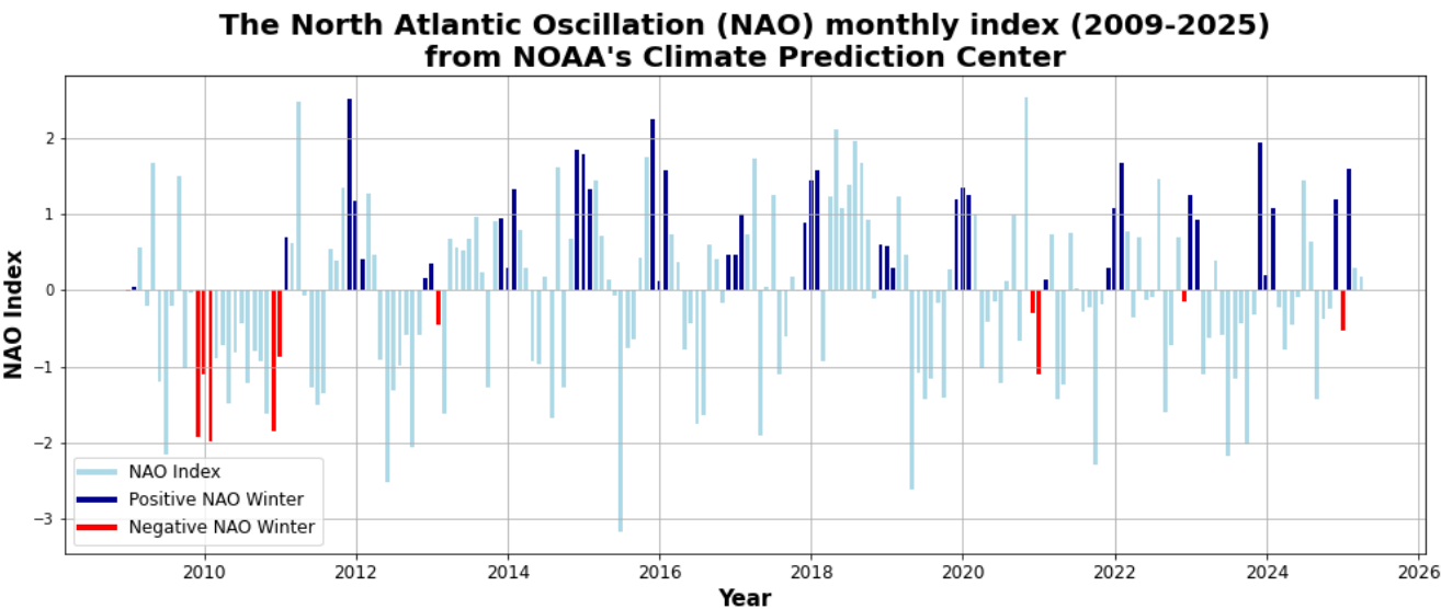
Figure A1. The monthly index of the North Atlantic Oscillation between 2009 and 2025. Data from NOAA’s Climate Prediction Center.
