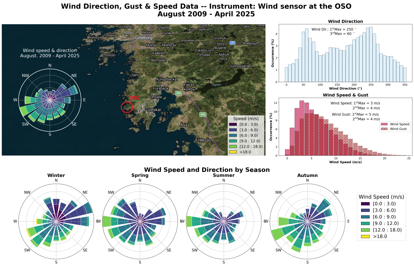
Figure 4. Wind direction and speed recorded at the OSO from 2009 to 2025. The central map (Source: Google Maps – https://maps.google.com ) shows the location of the OSO on the Swedish west coast for geographic context. The wind rose diagram (left on the map) displays the distribution of wind direction and speed data (1-minute temporal resolution) over the entire period. Top right: Wind direction (in °) histogram (i.e. frequency distribution) and wind speed (solid bars) and wind gust (hatched bars) histogram. Bottom panels: Seasonal wind roses (Winter, Spring, Summer, Autumn). Colours represent different wind speed classes.
