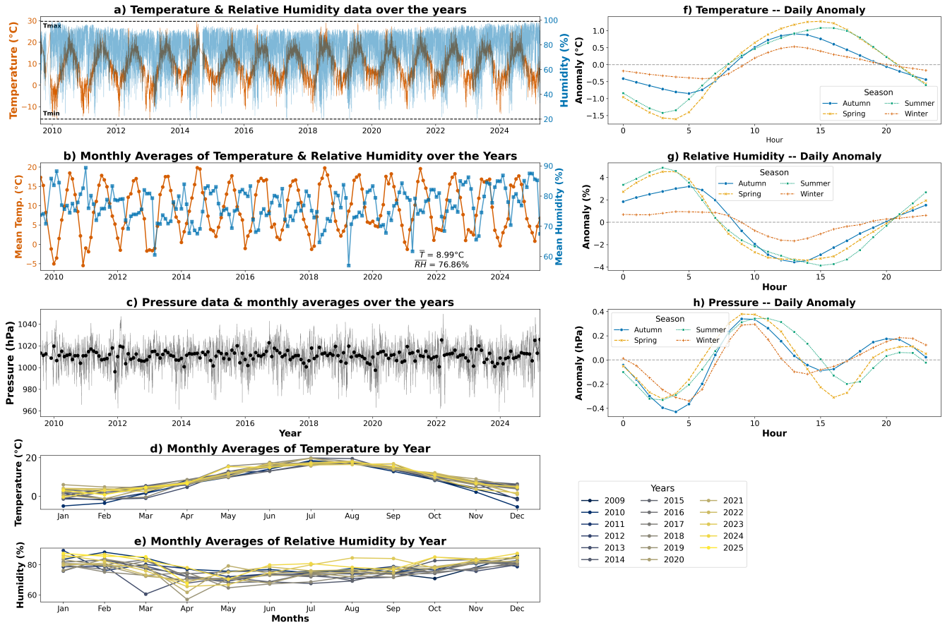
Figure 2. Temperature, relative humidity, and atmospheric pressure recorded at \sim 16 m a.s.l. by the Vaisala Weather transmitter WXT520 at the OSO over a 15-year and 8-month period. (a) Time series (1-minute temporal resolution) of temperature ( ^{\circ}\text{C} , red) and relative humidity ( \% , blue) data. (b) Monthly mean values (derived from a) of temperature and relative humidity, with overall means. (c) Time series of atmospheric pressure (hPa, grey) at \sim 16 m a.s.l., at 1-minute resolution, including monthly means (black). (d) Monthly mean temperature by year, color-coded by calendar year. (e) Monthly mean relative humidity by year, color-coded by calendar year. (f–h) Diurnal anomalies (from daily mean) of temperature (f), relative humidity (g), and pressure (h) averaged by season.
