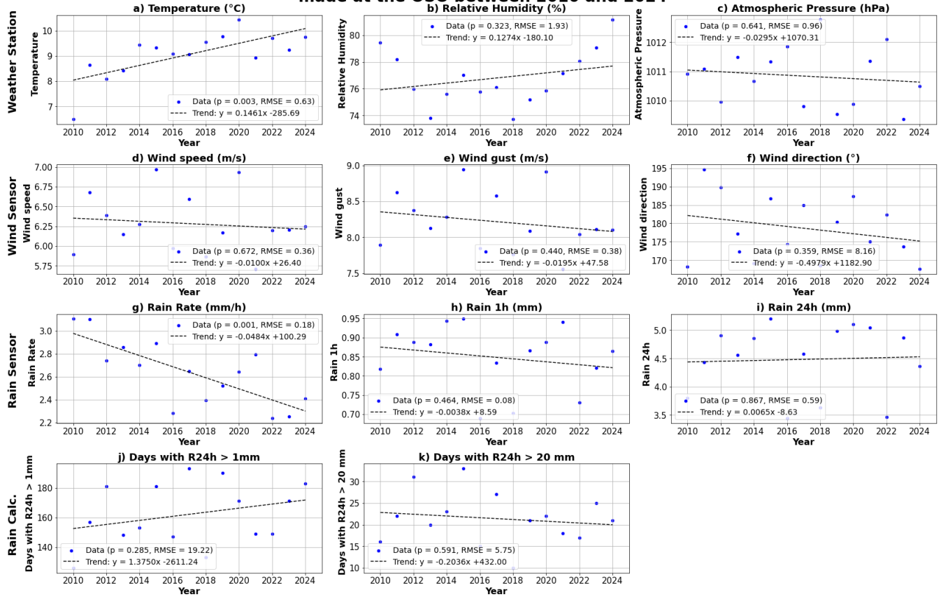
Figure 6. Annual mean values and linear trends of atmospheric variables recorded at the OSO from 2010 to 2024. Panels (a–c) show (a) temperature, (b) relative humidity, and (c) atmospheric pressure; panels (d–f) display wind characteristics: (d) wind speed, (e) gust speed, and (f) wind direction; panels (g–i) present precipitation metrics: (g) rain rate, (h) total rainfall in 1 h, and (i) total rainfall in 24 h; and panels (j–k) summarize rainfall occurrence: (j) number of days with \text{R24h} \geq 1 mm and (k) days with \text{R24h} \geq 20 mm. Dotted lines denote the best-fit linear trends, and p-values and RMSE for trend significance are indicated in each panel’s legend.
