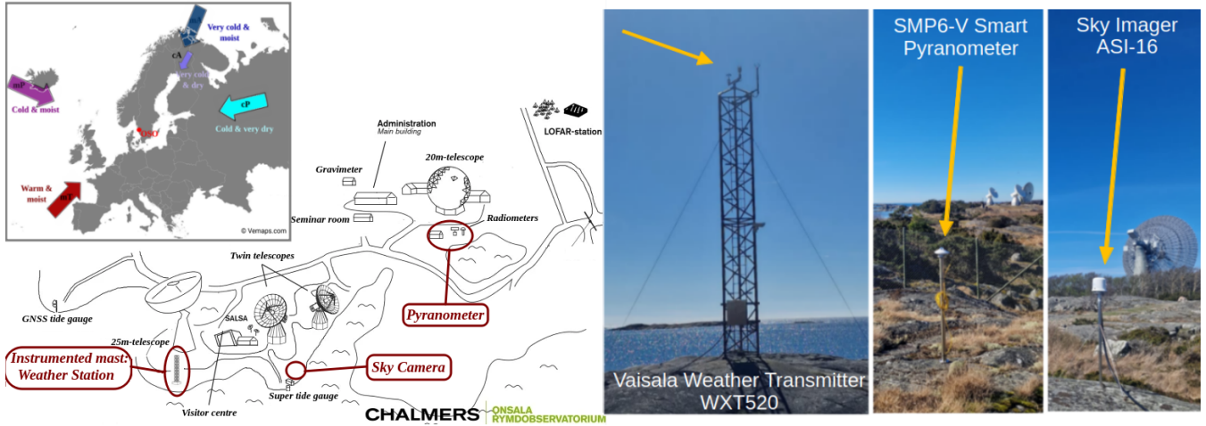
Figure 1. Locations and geographical context of the different measurements made at the OSO. Top left: Large-scale map ( source: https://vemaps.com ) and main air masses. Center: OSO map with instrument locations (atmospheric sensors highlighted in red). Right: Photos of each instrument used (Vaisala Weather transmitter WXT520, SMP6-V Smart Pyranometer and Sky Imager ASI-16). Photos made by drone for context.
