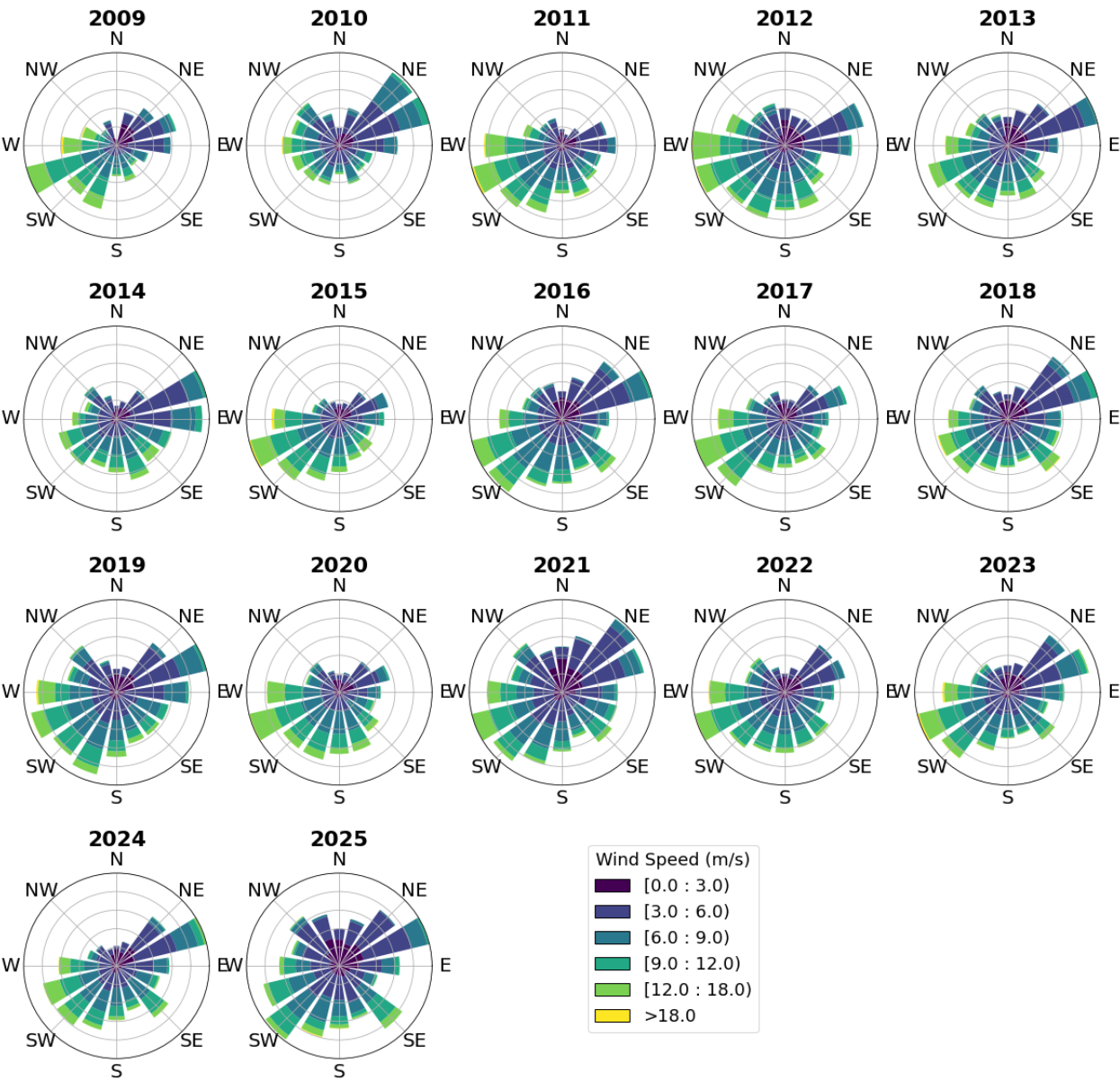
Figure B1. Annual wind-rose diagrams depicting the distribution of wind direction and speed from August 2009 to April 2025. Each panel represents one calendar year (2009–2025). Note that 2009 and 2025 are not complete years.
