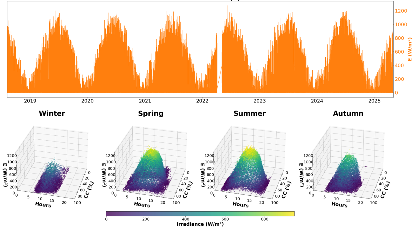
Figure 5. Temporal evolution and seasonal characteristics of solar irradiance ( E ) and cloud cover ( CC ), as measured by the pyranometer and estimated from the sky camera. Top panel: Time series of solar irradiance ( E , measured every minute, in \text{W/m}^2 ) from August 2018 to April 2025. Lower panel: 3D scatter plots of E as a function of CC and hour of day for each season (Winter, Spring, Summer, Autumn) between September 2019 and April 2025. For these scatter plots, only data at 15-min resolution are used, corresponding to the CC time step.
