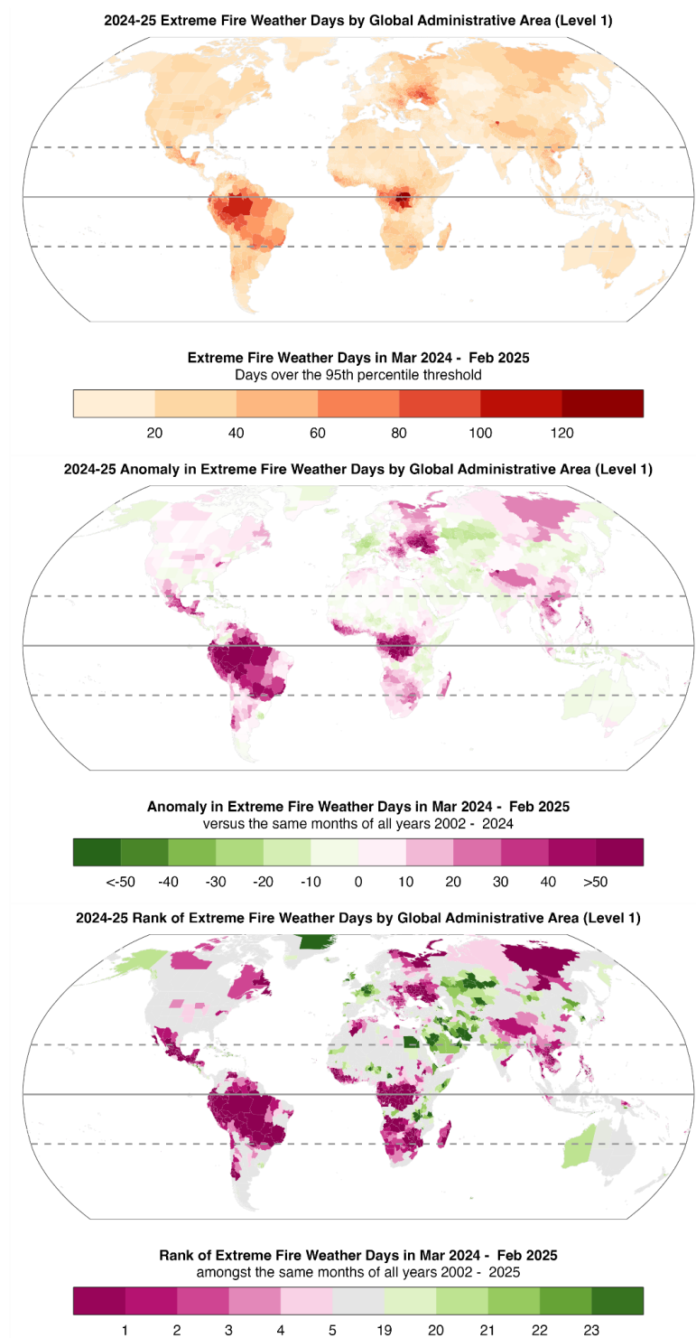
Figure S2: Extreme fire weather in the past fire season, including (top panel) the number of days with extreme (95 th percentile) fire weather during the 2024-25 fire season, (middle panel) the anomaly versus the mean of all prior fire seasons 2002-2024, and (bottom panel) rank amongst all fire seasons since 2002.
