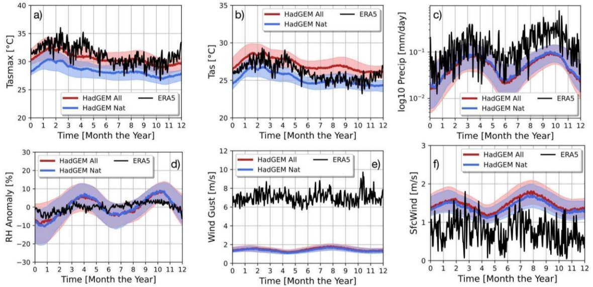
Figure S54: Same as in figure S52, but for the Congo Basin.
