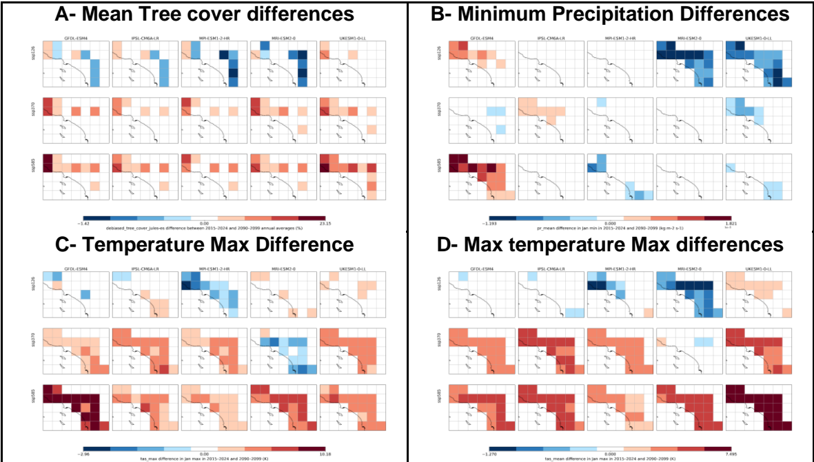
1317 Figure S42 Future projections of key bioclimate drivers of fire for Southern California, 1318 expressed as difference 2090s vs 2020s. Panels show (A) mean tree cover differences, (B) 1319 minimum precipitation differences, (C) mean maximum temperature differences, and (D) 1320 maximum temperature extremes differences. 1321 1322
