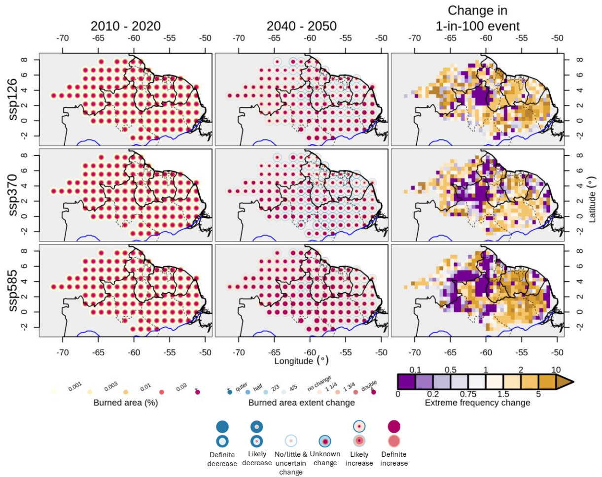
Figure S31: Same as Figure S30 for 2040s.
