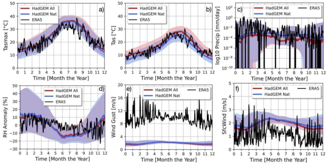
Figure S55: Same as in figure S52, but for the Southern California region.
