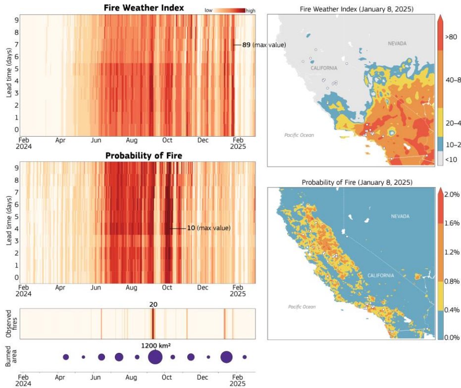
470 Figure S12: Southern California fire forecast (as for Figure 8 in the main text). Chicklet plots 471 displaying seamless FWI and POF fire predictions over 10 days forecast. The x-axis 472 corresponds to specific dates throughout the year, while the y-axis denotes either observations 473 or the time leading up to the date when a forecast was generated. The vertical colour 474 coherence allows for quick identification of the time windows of predictability associated to the 475 observed fire activity both provided in terms of number of detected active in a day fires and 476 total BA in a month (circles). The maps represents a snapshot in time at day 0 to allow the 477 comparison of the spatial distribution of the forecasts and the recorded fire activity by MODIS.
