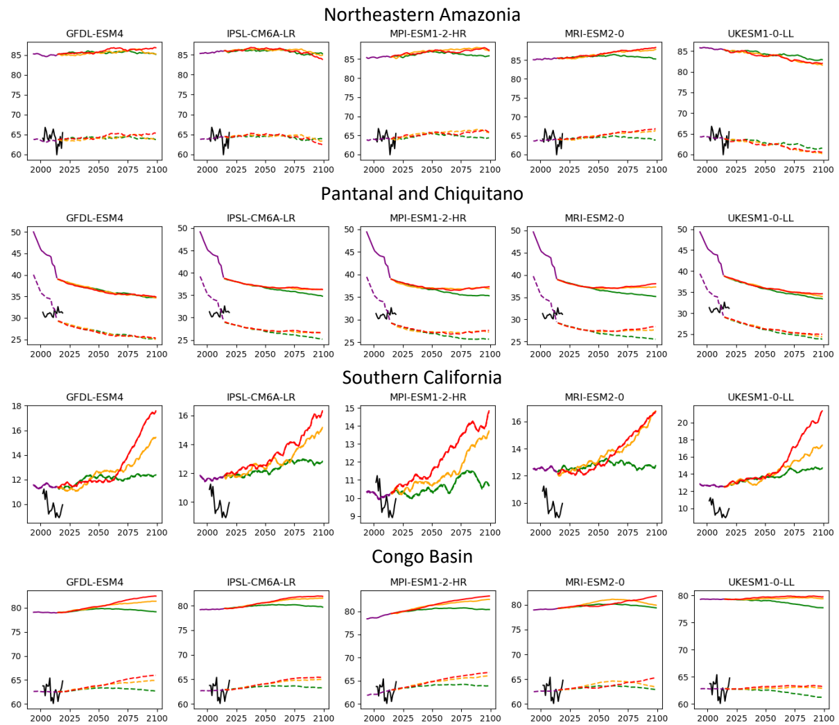
Figure S28: Time series of tree cover over each focal region for different climate models, both with historical and future scenario runs, raw model in solid lines, bias corrected models in dashed lines and MODIS VCF in black. Note that for Southern California, bias and non-bias corrected time series overlap one another.
