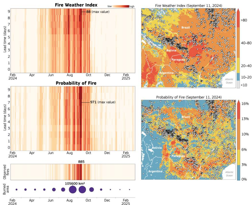
Figure S11: Pantanal and Chiquitano fire forecast (as for Figure 8 in the main text ). Chicklet plots displaying seamless FWI and POF fire predictions over 10 days forecast. The x-axis corresponds to specific dates throughout the year, while the y-axis denotes either observations or the time leading up to the date when a forecast was generated. The vertical colour coherence allows for quick identification of the time windows of predictability associated to the observed fire activity both provided in terms of number of detected active in a day fires and total BA in a month (circles). The maps represents a snapshot in time at day 0 to allow the comparison of the spatial distribution of the forecasts and the recorded fire activity by MODIS.
