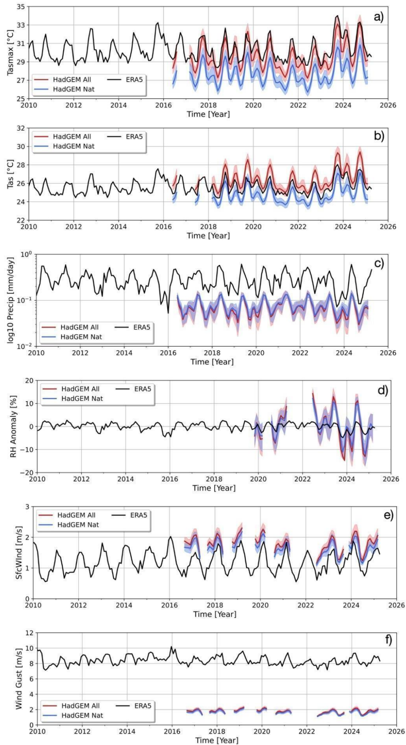
Figure S48: January 2010 to April 2025 time series of individual component variables of the FWI from HadGEM (red: all forcing scenario, blue: natural forcing scenario) compared to ERA5 reanalysis (black) over northeast Amazonia region. We show monthly mean a) daily maximum temperature, b) temperature, c) total precipitation, d) relative humidity, e) wind speed as well as f) wind gusts. Shading represents the 5th-95th percentile confidence interval.
