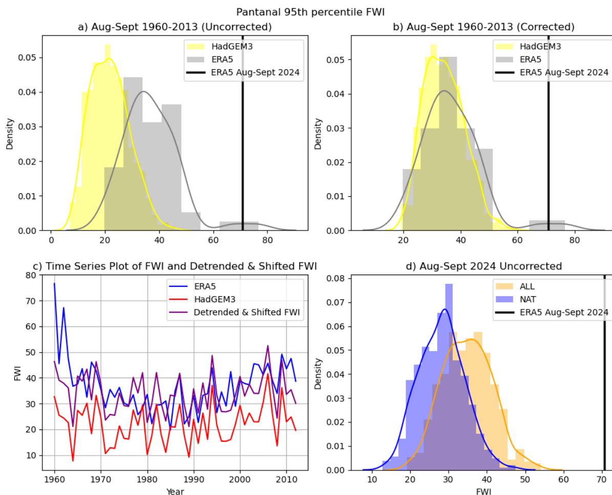
Figure S57: As for Figure S56 , but for Pantanal & Chiquitano
