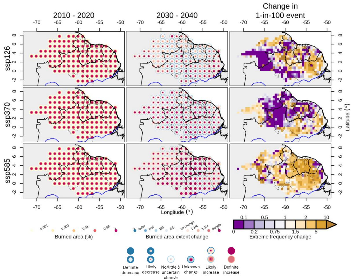
Figure S30: Projected changes in January-March 2024 BA over Northeast Amazonia by 2030–2040 under three SSP scenarios, with BA simulated by ConFLAME. (Left) Average JFM BA fraction (%) for 2010–2020. (Middle) Relative change in JFM BA extent projected for 2030–2040 period, expressed as a multiplier of 2010–2020 values. (Right) Increased (or decreased) frequency in the 2030s period of a 1-in-100 year event defined for the period 2010–2020, expressed as a multiplier of 2010–2020 values. In the left column, the size of the dot in each grid cell indicates the likelihood (larger = higher likelihood) of a BA fraction being greater than the threshold indicated by the coloured dot (see legend at the base). Likewise, in the middle column the size of the dot varies with likelihood that the BA fraction exceeds the threshold indicated by the coloured dot (see legend at the base). For example, a large pale orange dot in the left column indicates a high likelihood of the BA fraction exceeding 0.03%, whereas a small dark red dot indicates a small (but non-zero) likelihood of the BA fraction exceeding 0.03%+.
