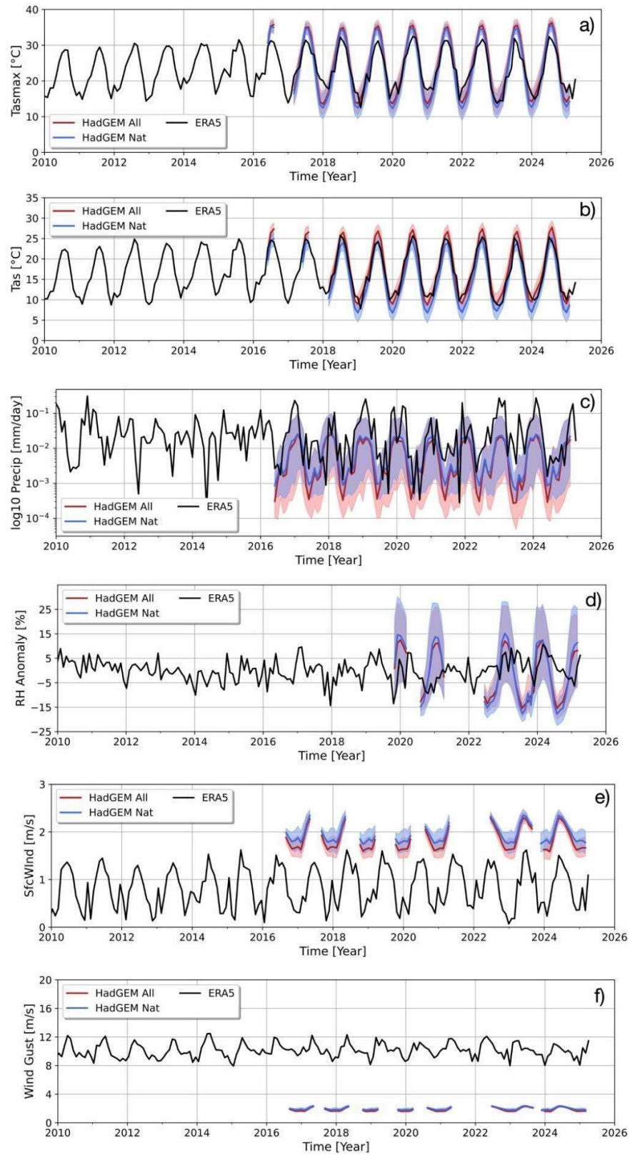
Figure S51: Same as in figure S48, but for the Southern California region.
