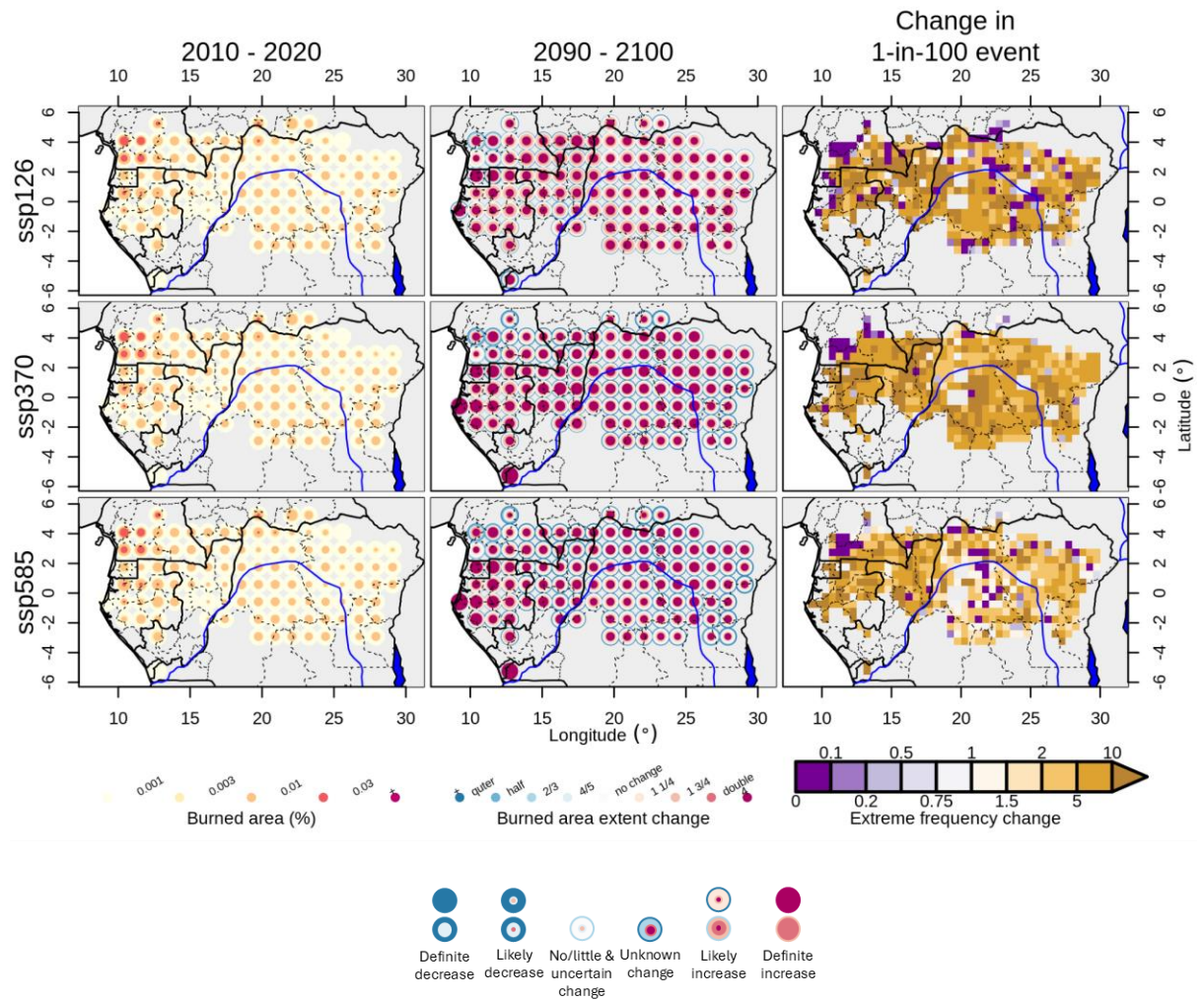
Figure S41: Same as Figure S39 for 2090s.
