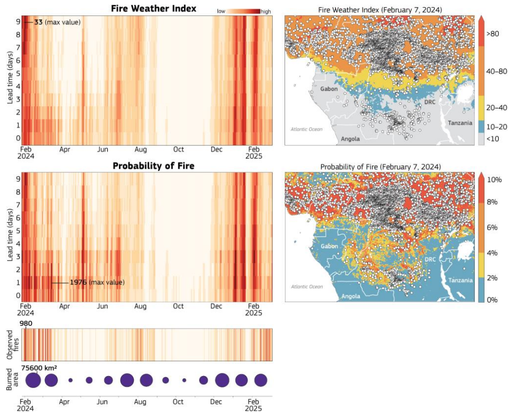
479 Figure S13: Congo basin fire forecast (as for Figure 8 in the main text ). Chicklet plots 480 displaying seamless FWI and POF fire predictions over 10 days forecast. The x-axis 481 corresponds to specific dates throughout the year, while the y-axis denotes either observations 482 or the time leading up to the date when a forecast was generated. The vertical colour 483 coherence allows for quick identification of the time windows of predictability associated to the 484 observed fire activity both provided in terms of number of detected active in a day fires and 485 total BA in a month (circles). The maps represents a snapshot in time at day 0 to allow the 486 comparison of the spatial distribution of the forecasts and the recorded fire activity by MODIS.
