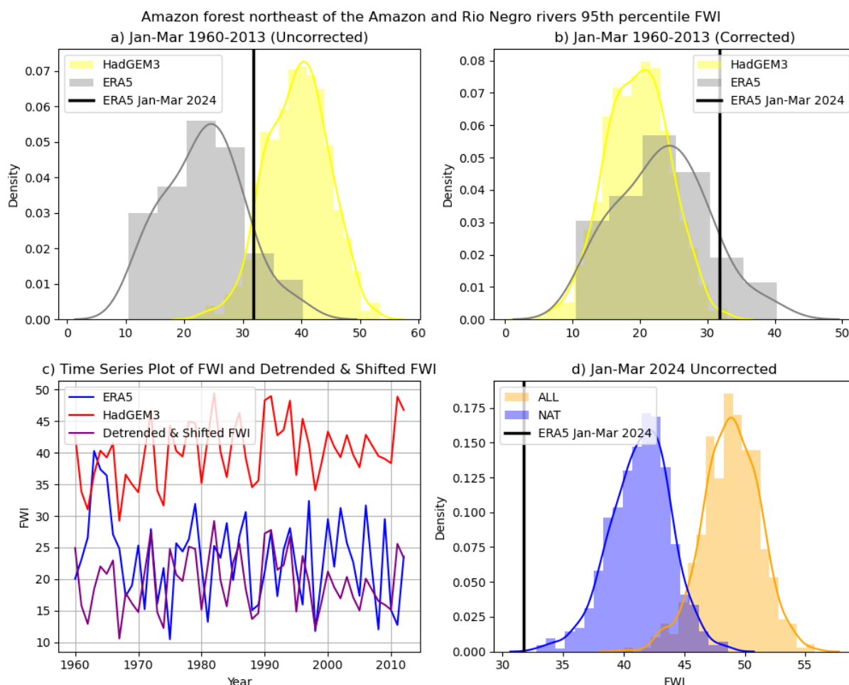
Figure S56: Bias correction for Amazon forest northeast of the Amazon and Rio Negro rivers. Historical ensemble of HadGEM3 (yellow) compared to ERA5 (grey) 95th percentile of FWI for the historical period (1960-2013), shown as probability density before correction (a) and after correction (b), and one member shown as a time series (c, where HadGEM3 is shown in red, ERA5 in blue and corrected HadGEM3 in purple). HadGEM3 ensemble for 2024 shown before bias-correction (d). ERA5 2024 event shown as black vertical line on all probability density plots.
