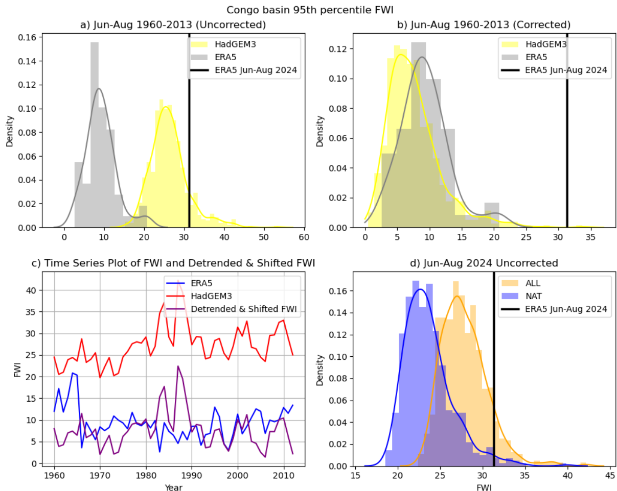
Figure S58: As for Figure S56 , but for Congo basin
