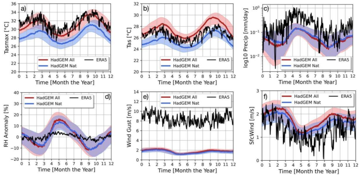
Figure S52: Seasonal cycle of individual component variables of the FWI from HadGEM (red: all forcing scenario, blue: natural forcing scenario) compared to ERA5 reanalysis (black) across 2024 over the northeast Amazonia region. We show daily a) maximum temperature, b) mean temperature, c) total precipitation, d) relative humidity, e) wind gusts as well as f) mean wind speed. Shading represents the 5th-95th percentile confidence interval.
