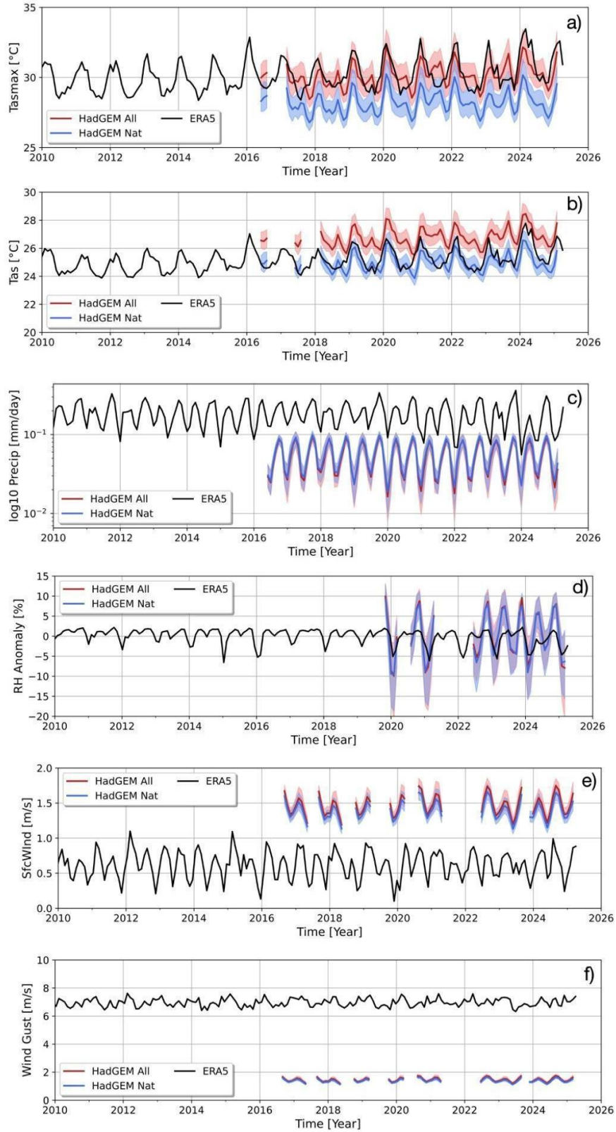
Figure S50: Same as in figure S48, but for the Congo Basin.
