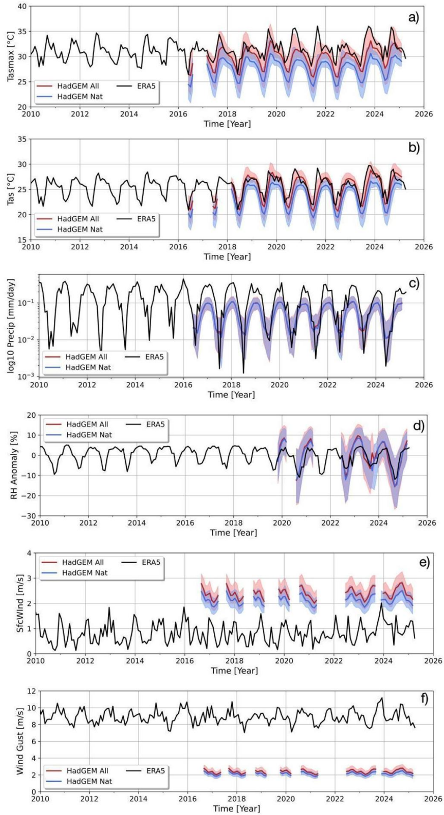
Figure S49: Same as in figure S48, but for the Pantanal-Chiquitano.
