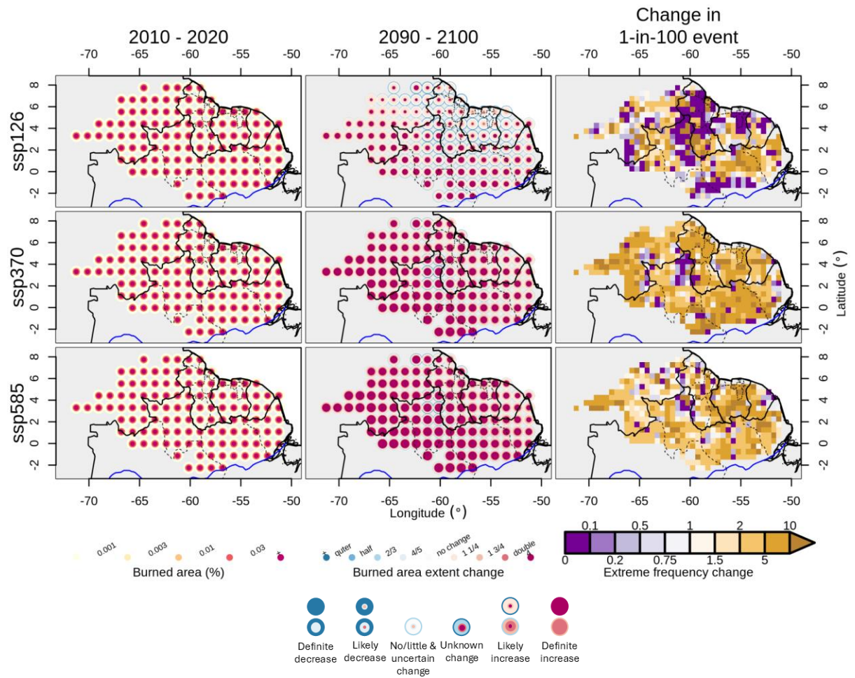
Figure S32: Same as Figure S30 for 2090s.
