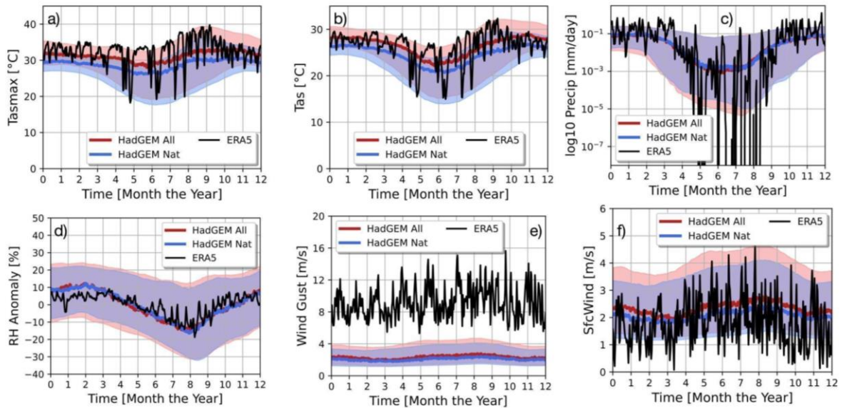
Figure S53: Same as in figure S52, but for the Pantanal-Chiquitano.
