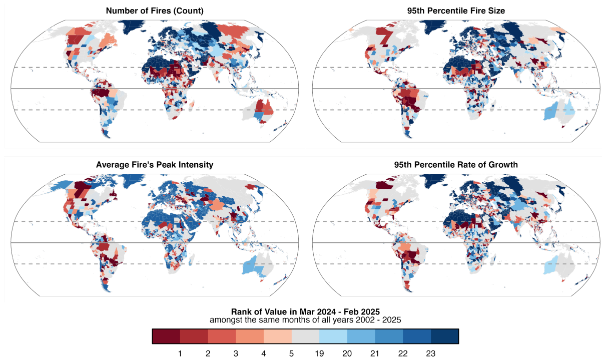
Figure 4: Ranks of selected individual fire properties during the March 2024-February 2025 fire season versus previous March-February periods (n = 23 global fire seasons), including (top left) fire count, (top right) 95th percentile fire size, (bottom left) the average value of a the peak intensity (95th percentile FRP within fire perimeters) considering all regional fires, and (bottom right) 95th percentile daily rate of growth. Results are shown at the scale of states or provinces (GADM administrative level 1 regions).
