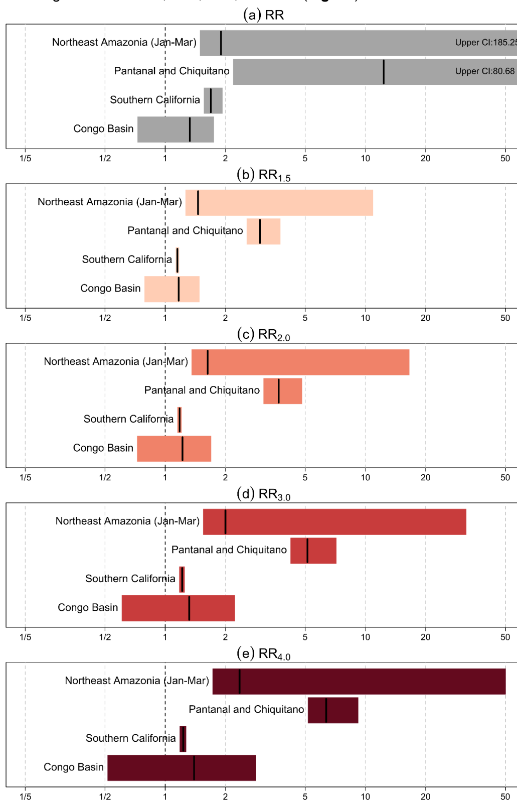
Figure 17: Risk Ratio (RR) estimates based on the comparison between (a) the past climate of 1850-1859 and the recent climate of 2016-2025, (b) the recent climate of 2016-2025 and
