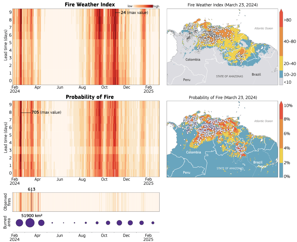
Figure 8: Northeast Amazonia forecasts of the FWI and PoF with lead times up to 10 days prior for the period February 2024-February 2025 as an average value over the focal area. The total percentage of PoF values over the focal region translates into a number of predicted hotspots and this is directly comparable to the detections observed by MODIS. The x-axis corresponds to specific dates throughout the year, while the y-axis denotes either observations or the time leading up to the date when a forecast was generated. The vertical colour coherence allows for quick identification of the time windows of predictability associated with the observed fire activity both provided in terms of number of detected active fires per day and total monthly BA (circles). The maps represent a snapshot in time at day 0 to allow the comparison of the spatial distribution of the forecasts and the recorded fire activity by MODIS.
