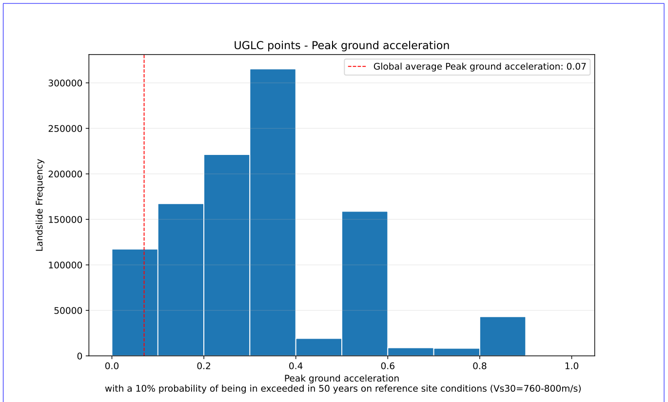
Figure 11. UGLC Landslide Points compared with global seismic hazard expressed as peak ground acceleration (PGA) from the Global Earthquake Model (GEM), corresponding to a 10% probability of exceed in 50 years under reference site conditions ( V_{s30} = 760\text{--}800\text{ m/s} ).
