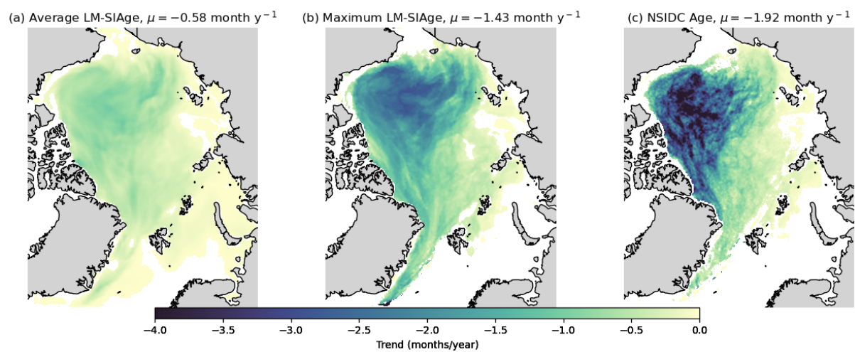
Figure 15. Linear trends in reduction of sea ice age [month/year] between 1995 – 2024 from three sources: weighted average LM-SIAge (a), max LM-SIAge (b), and NSIDC Age (bc). Insignificant trends are masked by white colour.
