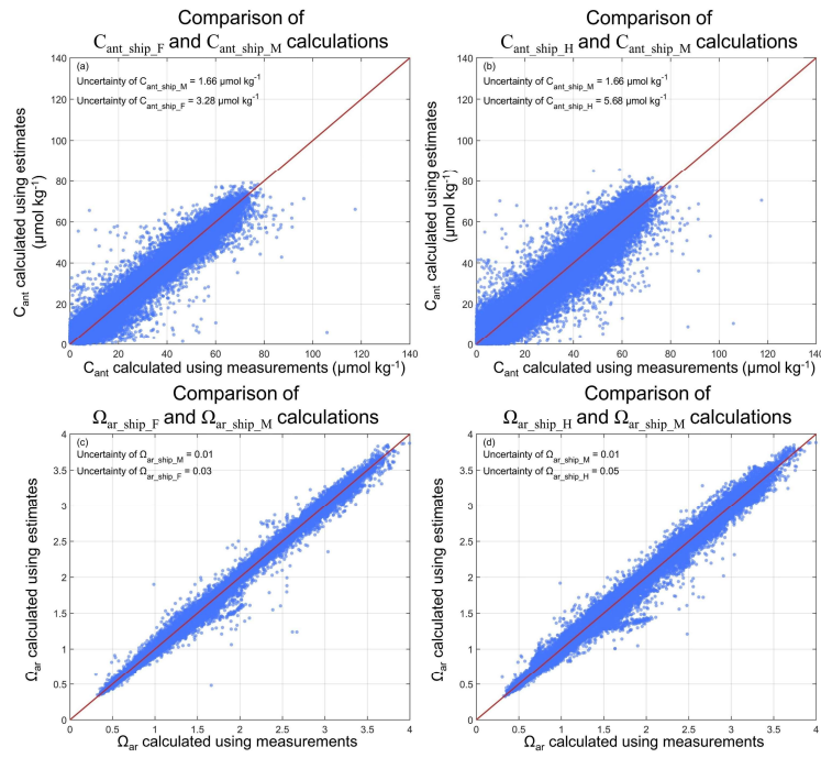
Figure A3. Intercomparison between C_{\text{ant}} and \Omega_{\text{ar}} calculations based on ESPER_NN-derived variables and direct measurements. (a-b) Scatterplots of C_{\text{ant}} concentration calculated using ESPER_NN-derived variables and direct shipboard measurements. (c-d) Same as (a-b), but for \Omega_{\text{ar}} values. The uncertainties are shown in the left-top of subplot a-d.
