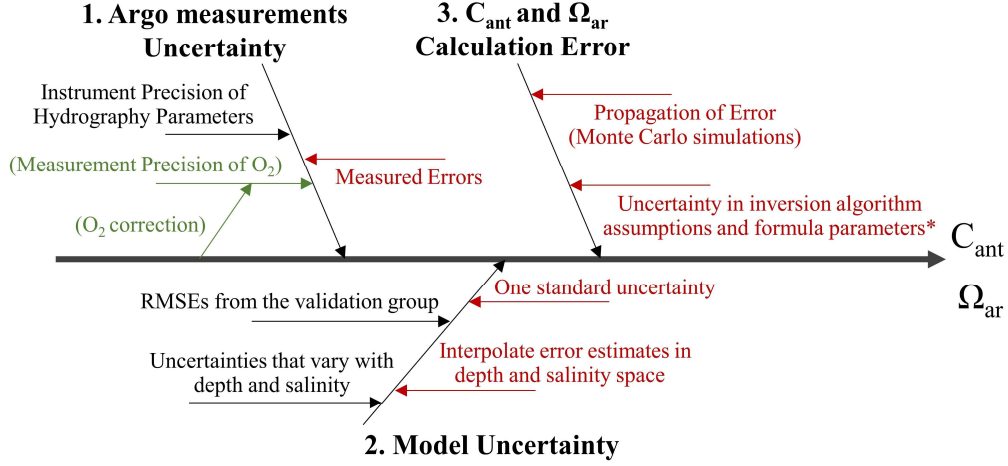
285 Figure 4. Error propagation that may arise during the calculation process of reconstructed variables and calculated values ( C_{ant} and \Omega_{ar} ).
