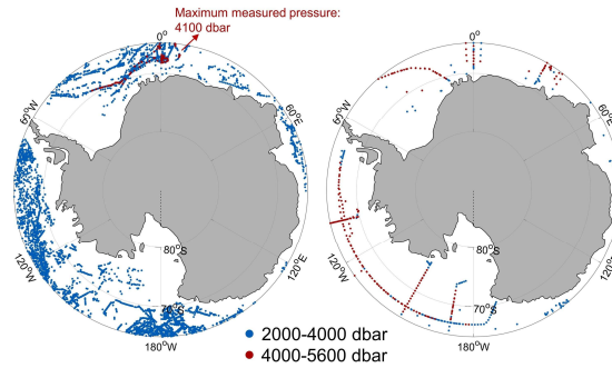
Figure A6. The location of the observations measured by Argo floats (a) or ship (b) in south of 65^\circ\text{S} . The blue and red symbol denotes measurement in the intermediate layer (2000-4000 dbar) and the abyssal layer (4000-5600 dbar), respectively.
