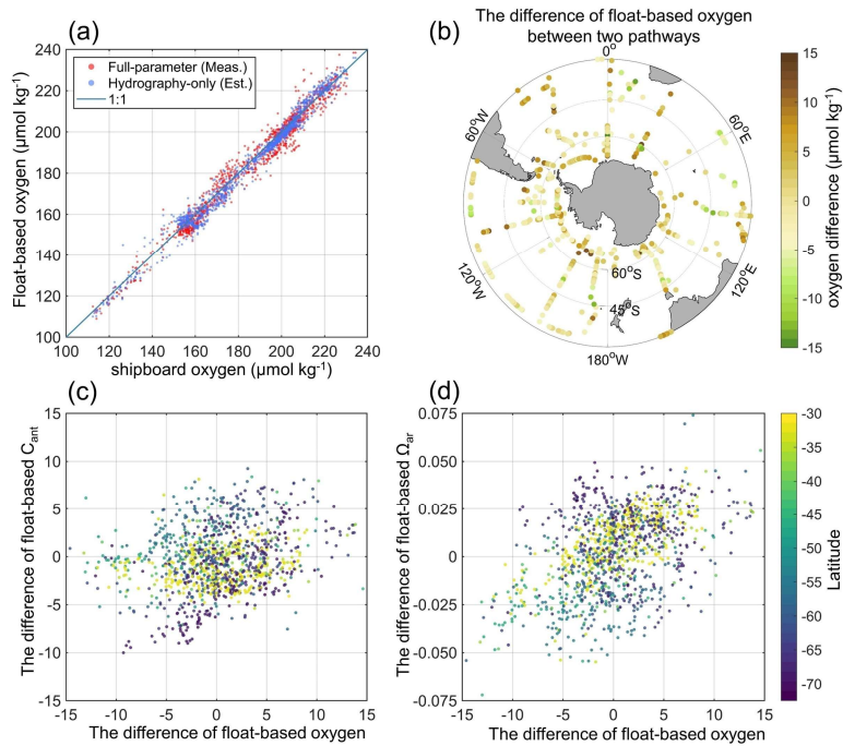
Figure 6. Scatter comparisons and spatial distributions of difference in O_2 , C_{ant} and \Omega_{ar} between the two reconstruction pathways, restricted to the 1,400-2,100 dbar range. (a) scatter plot comparing float-based and ship-based oxygen measurements
