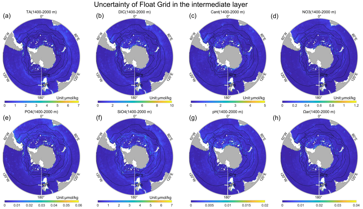
Figure A8. The uncertainty of the Float Grid in the intermediate layer (1400-2000 m) for (a) TA, (b) DIC, (c) C_{\text{ant}} , (d) NO 3 , (e) PO 4 , (f) SiO 4 , (g) pH, and (h) \Omega_{\text{ar}} .
