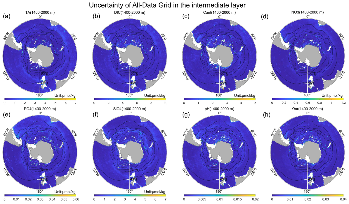
Figure A7. The uncertainty of the All-Data Grid in the intermediate layer (1400-2000 m) for (a) TA, (b) DIC, (c) C_{\text{ant}} , (d) NO 3 , (e) PO 4 , (f) SiO 4 , (g) pH, and (h) \Omega_{\text{ar}} .
