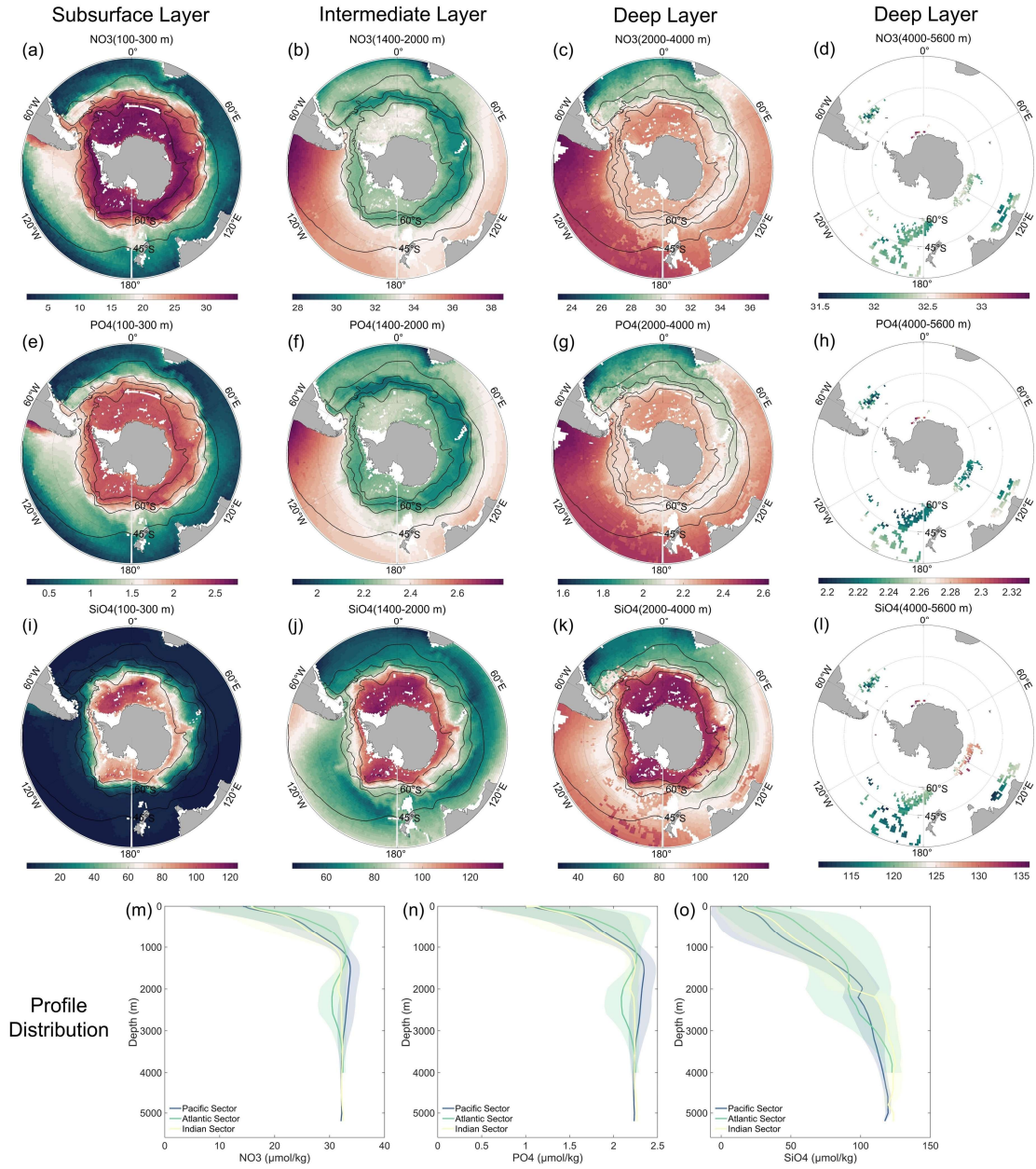
Figure A5. Averaged climatological distribution of \text{NO}_3 (a-d), \text{PO}_4 (e-h), and \text{SiO}_4 (i-l) in oceanic sectors (m-o) and four layers: subsurface layer (100 to 300 m), intermediate layer (1400 to 2000 m), deep layer (2000 to 4000 m), and abyssal layer (4000 to 5600 m). The climatology is based on the Float Grid derived from Argo profile data spanning 2001-2024. The thin black lines show, from north to south, the Subtropical Front (STF), the Subantarctic Front (SAF), the Polar Front (PF), and the Southern Antarctic Circumpolar Current Front (SACCF) (Oris et al., 1995). Note that the color scales differ among the individual maps.
