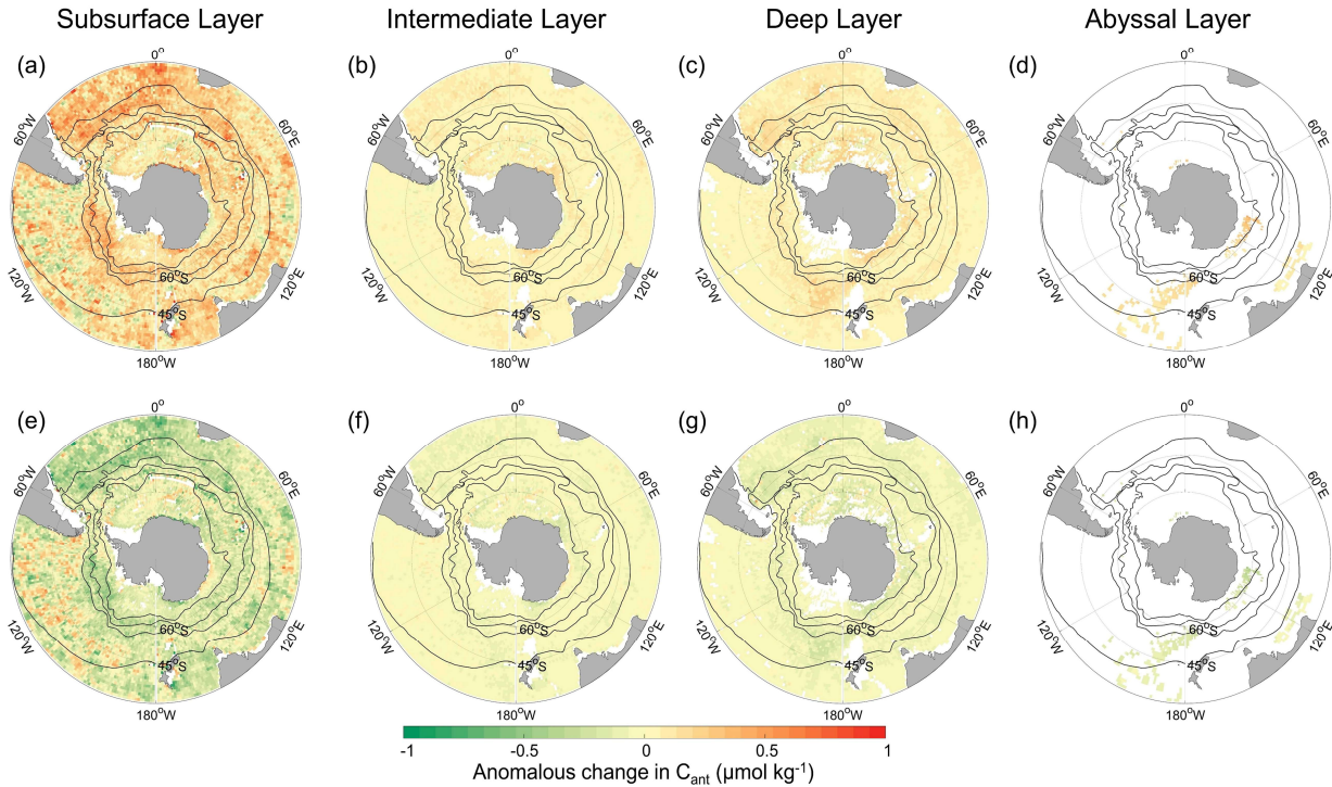
Figure B1. Sensitivity of anomalous change in C_{\text{ant}} distribution to the value of the scaling factor \alpha=0.44 (a-d) and \alpha=0.52 (e-h) in four layers: subsurface layer (100 to 300 m), intermediate layer (1400 to 2000 m), deep layer (2000 to 4000 m), and abyssal layer (4000 to 5600 m).
