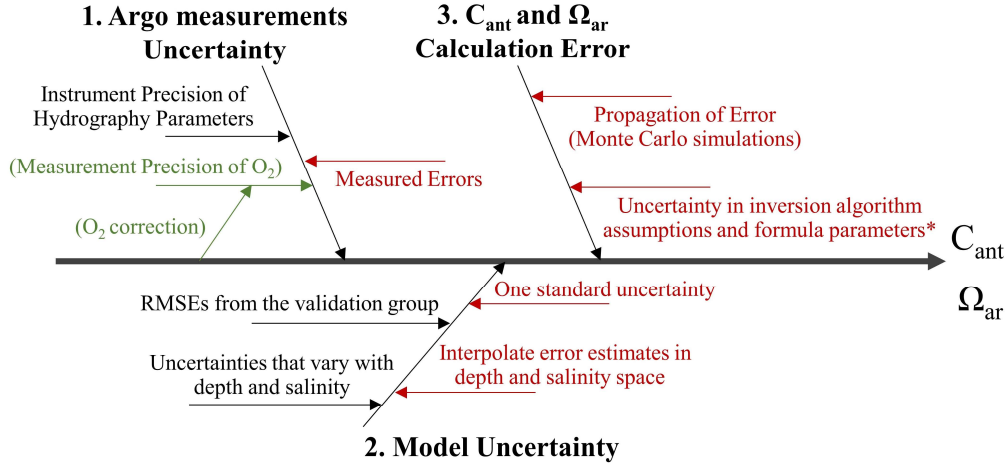
Figure 4. Error propagation that may arise during the calculation process of reconstructed variables and calculated values ( C_{ant} and \Omega_{ar} ).
