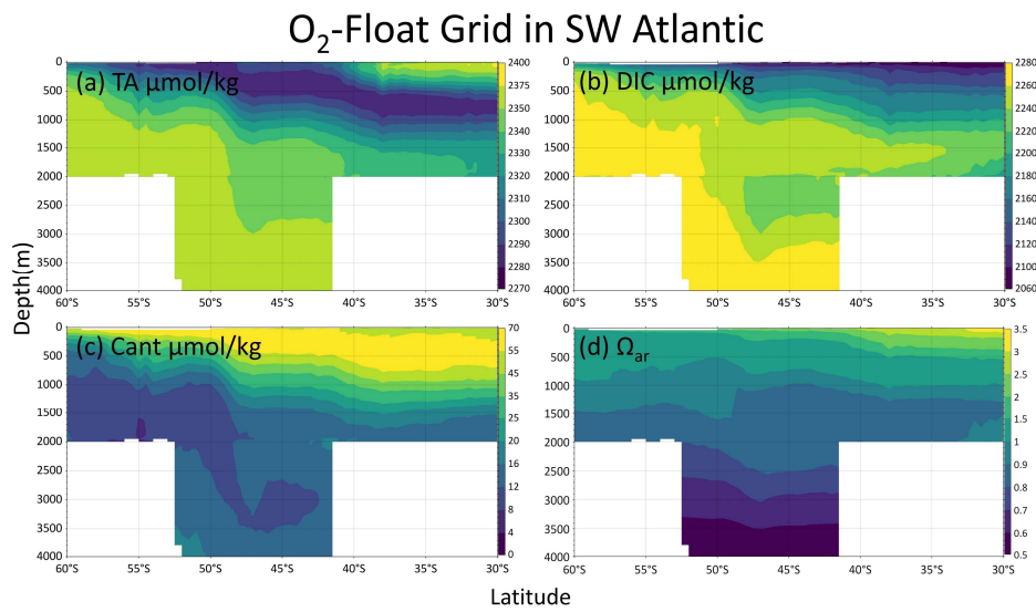
Figure B4. Zonal-mean sections (averaged between 60°W and 30°W) of TA (a), DIC (b), C ant (c), and Ω ar (d) from 60°S to 30°S in the southwestern Atlantic Ocean. The profiles are from the O 2 -Float Grid.
