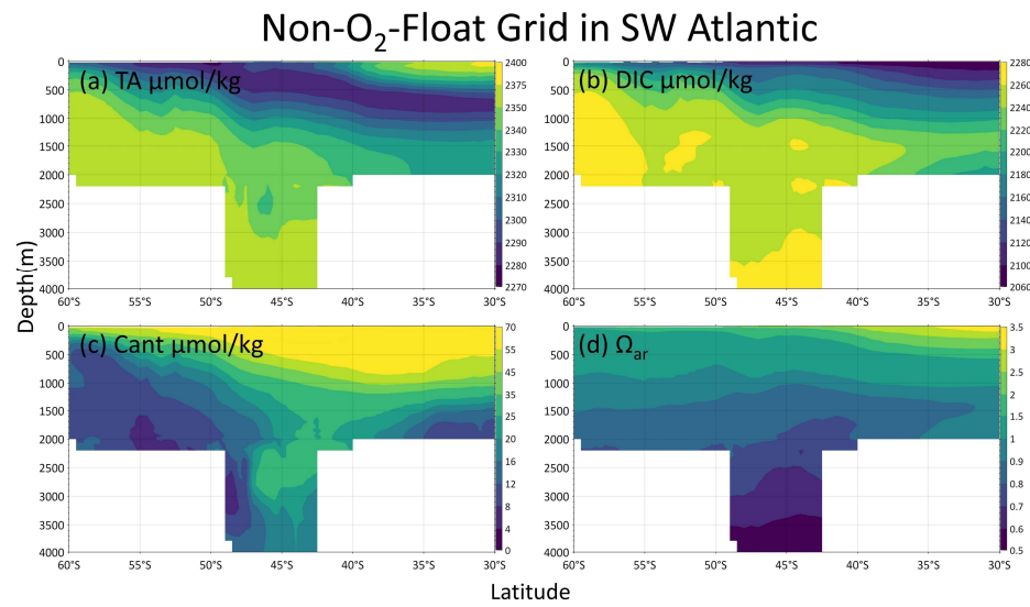
Figure B5. Zonal-mean sections (averaged between 60°W and 30°W) of TA (a), DIC (b), C ant (c), and Ω ar (d) from 60°S to 30°S in the southwestern Atlantic Ocean. The profiles are from the Non-O 2 -Float Grid.
