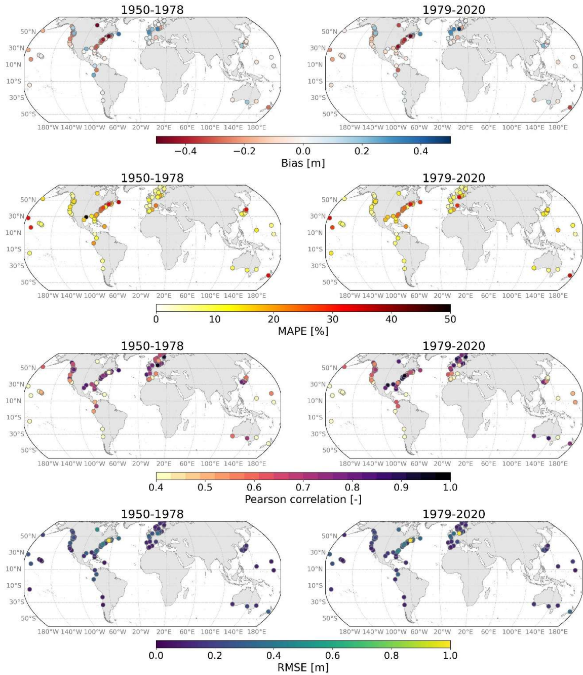
Figure 2: Global map showing the comparison between the modelled and observed annual maxima water levels for two periods: 1950-1978 (left) and 1979-2020 (right) for the following metrics (from top to bottom): bias, mean absolute percentage error (MAPE), Pearson correlation coefficient and RMSE.
