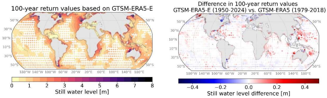
265 Figure 5: Global maps showing the 100-year return values based on 1950-2024 water levels (left) and a difference between 100- 270 year return values between the GTSM-ERA5-E dataset (1950-2024) and the original GTSM-ERA5 dataset (1979-2018). The difference plots are calculated by subtracting the GTSM-ERA5 100-year water levels from the GTSM-ERA5-E 100-year water levels.
