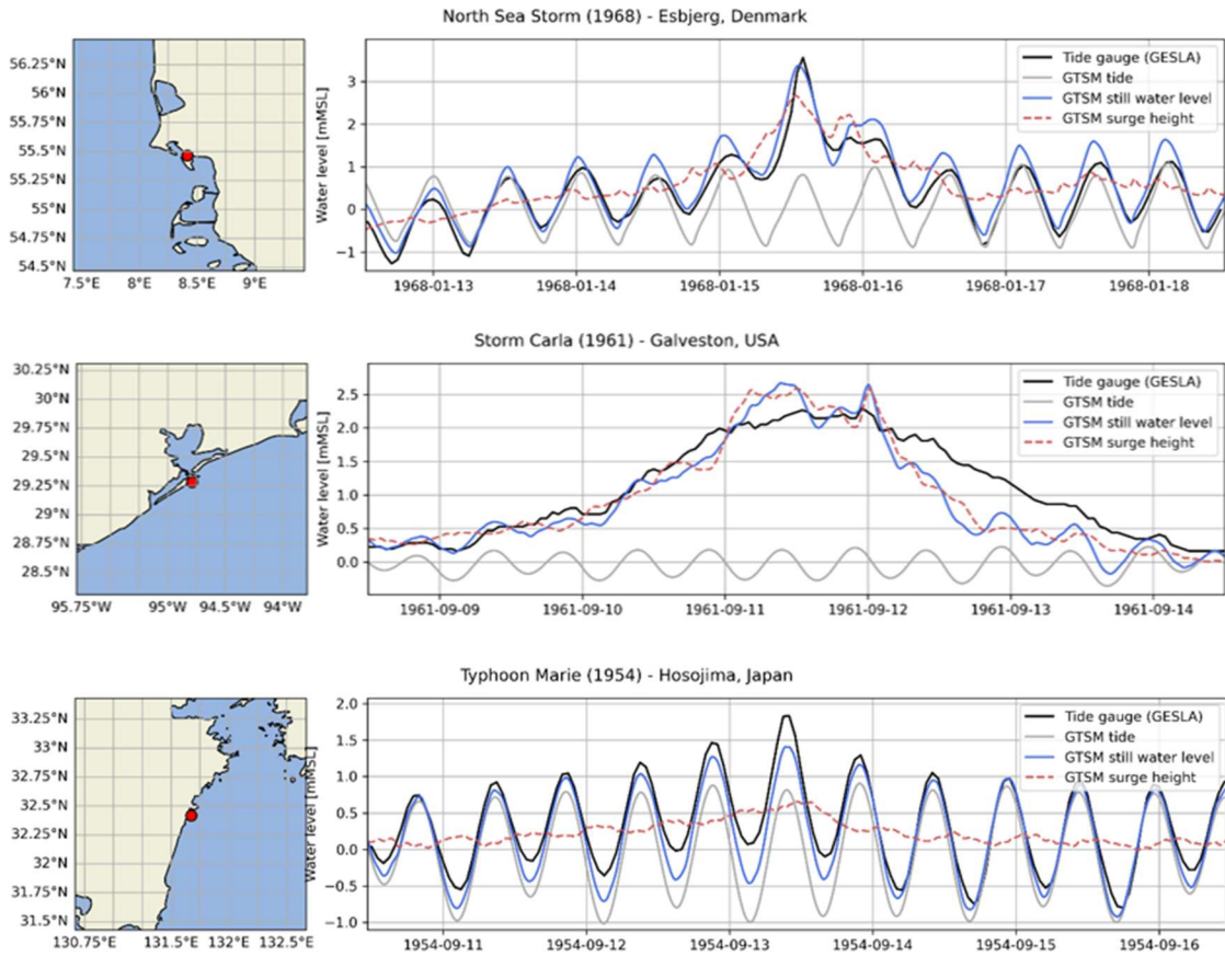
Figure 3: Water levels, tides and surge heights extracted from the GTSM-ERA5-E database for locations affected by high surges during historical storm events, including the North Sea storm in 1968, hurricane Carla (1961), and typhoon Marie (1954).
