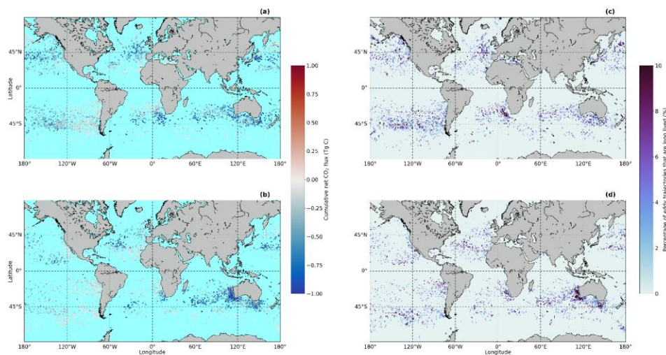
Figure 2 Figure 4: (a) The cumulative air-sea CO 2 flux into the anticyclonic eddies where the scatter points are plotted at the formation location of each eddy. (b) same as (a) but for cyclonic eddies. (c) The percentage of long lived anticyclonic eddy trajectories compared to all eddy trajectories that form in 1 degree by 1 degree regions. (d) same as (c) but for cyclonic eddies. Basemap from Natural Earth v4.0.0 ( https://www.naturalearthdata.com/ ). Supplementary Figure S1 shows the equivalent of (a) and (b) in Tg C d -1 to remove the differences in eddy lifetime.
