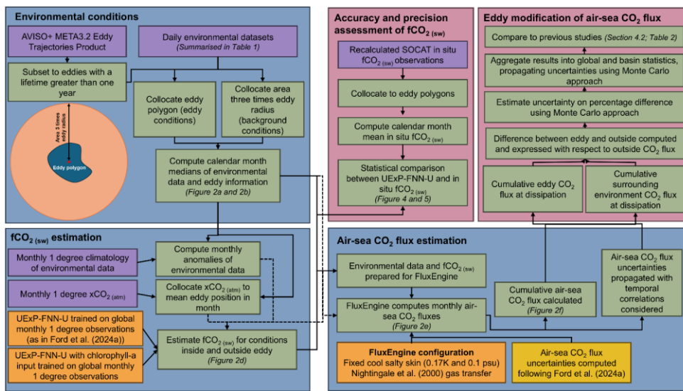
Figure 1: Schematic showing the processing steps to estimate the air-sea \text{CO}_2 flux within long lived eddies (Blue box background). The pink background boxes indicate the analysis completed to evaluate the accuracy and precision of the dataset. In figure acronyms are: fugacity of \text{CO}_2 in seawater ( \text{fCO}_2(\text{sw}) ), atmospheric dry mixing ratio of \text{CO}_2 ( \text{xCO}_2(\text{atm}) ) and University of Exeter feed forward neural network with uncertainties (UExP-FNN-U).
