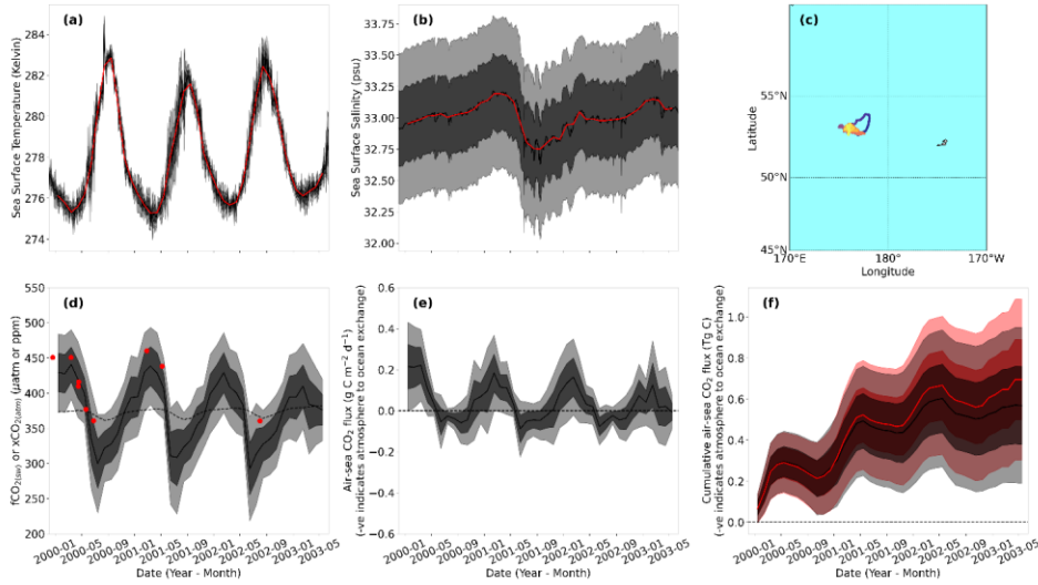
Figure 3 Figure-2: Exemplar eddy trajectory (eddy 194465) in the North Pacific Ocean with calculated air-sea CO 2 fluxes (a) Sea surface temperature (SST) for the example eddy's lifetime. Black line is the daily SST, where dark grey and light grey shading indicates the 1 sigma (~67% confidence) and 2 sigma (~95% confidence) uncertainties. Red line is the median monthly SST. (b) same as (a) for sea surface salinity. (c) Geographical eddy trajectory, where colour indicates the age of eddy (blue is eddy formation and yellow is eddy dissipation). (d) Monthly timeseries of fugacity of CO 2 in seawater ( f\text{CO}_2(\text{sw}) ; solid line) and dry mixing ratio of CO 2 in the atmosphere ( x\text{CO}_2(\text{atm}) ; dashed line) for the eddy. Dark grey and light grey shading indicates the 1 sigma (~67% confidence) and 2 sigma (~95% confidence) uncertainties on the f\text{CO}_2(\text{sw}) . Red dots indicate f\text{CO}_2(\text{sw}) in situ observations from the Surface Ocean CO 2 Atlas within the eddy. (e) same as (d) but for the air-sea CO 2 flux where a positive flux means CO 2 outgassing. Dashed black line indicates an air-sea CO 2 flux of 0. (f) same as (d) but for the cumulative air-sea CO 2 flux. Red line and banding indicate the cumulative air-sea CO 2 flux for the surrounding environment.
