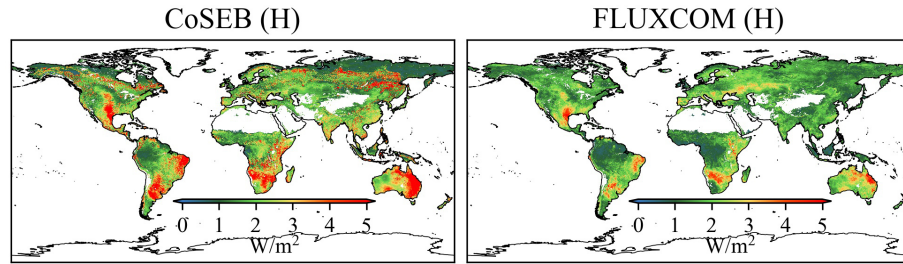
Figure 17. Spatial distribution of interannual variability (standard deviation) of sensible heat flux ( H ) from 2001 to 2018 by the CoSEB-based datasets and FLUXCOM.
