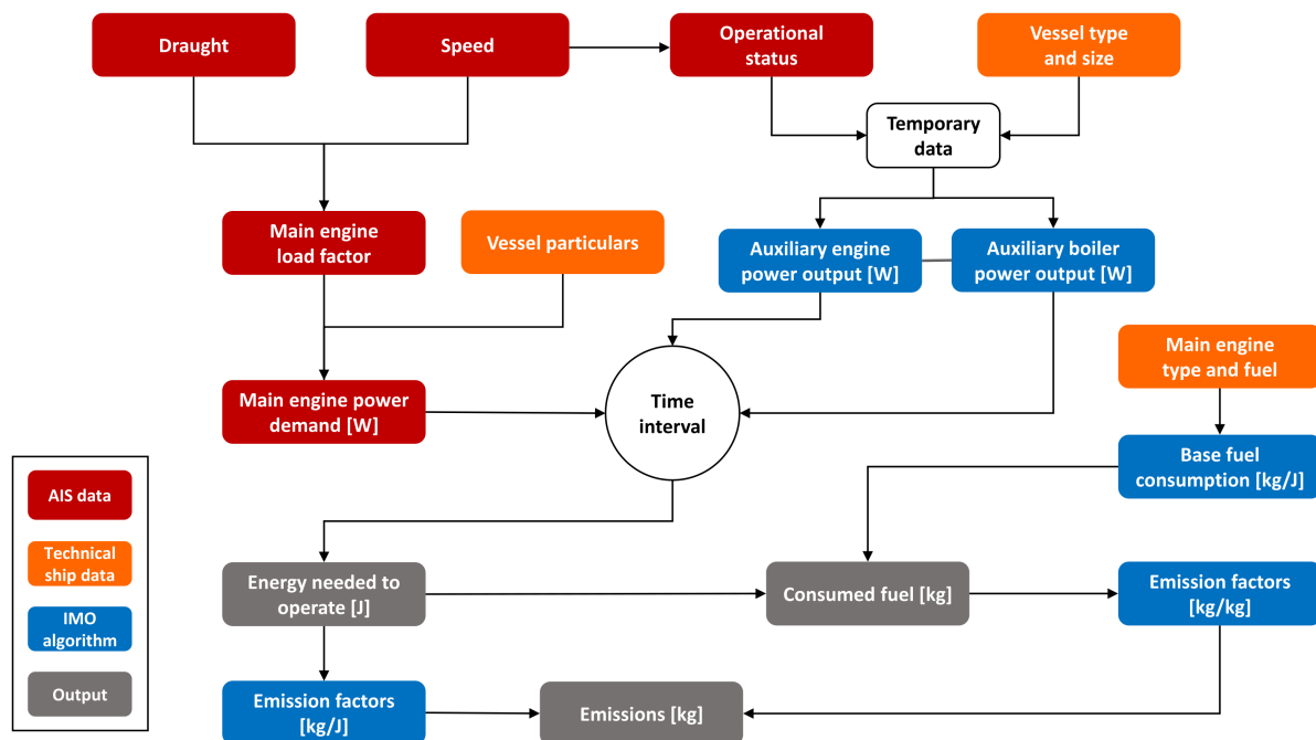
Figure 3. Schematic overview of the method applied for calculating the emissions from international shipping.
