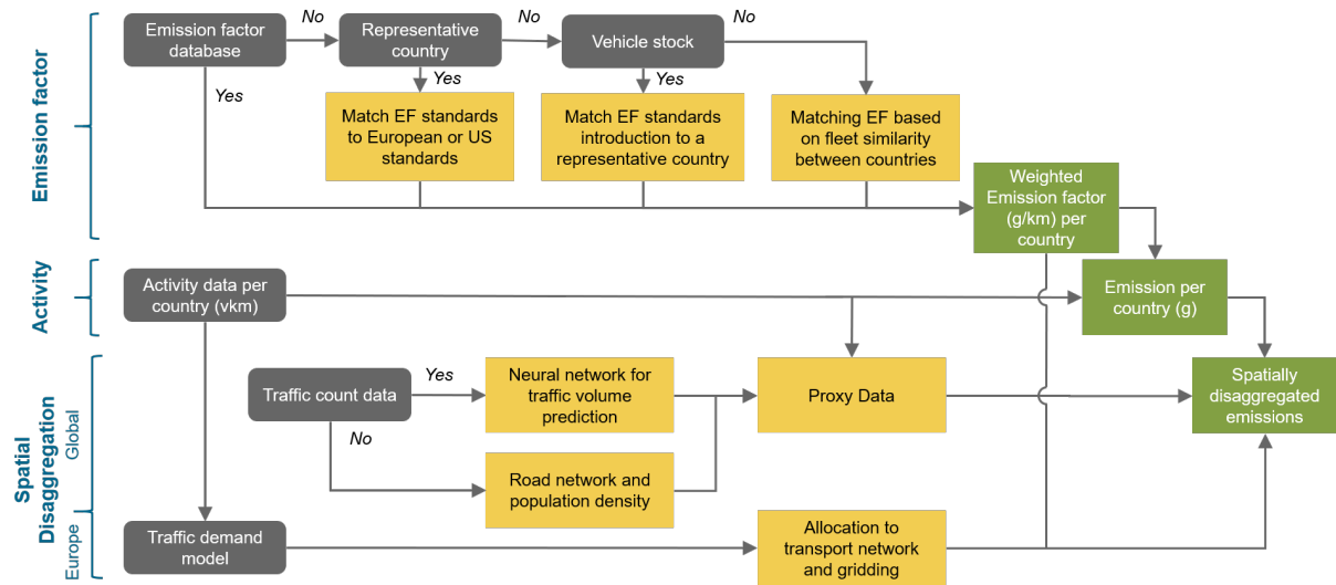
Figure 1. Schematic of the emission computation for a given vehicle category.
