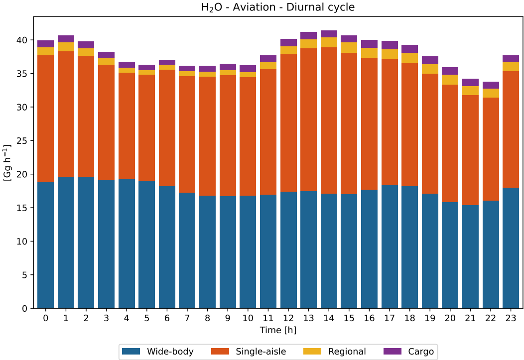
Figure 14. Aviation: Diurnal cycle of the annual total aviation H 2 O emissions by hour (UTC) and subsector for an average day.
