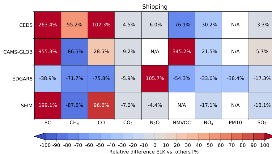
Figure 10. As in Fig. 7, but for shipping emissions. Note that the CEDS and EDGAR8 inventories do not include inland navigation in the shipping sector.
