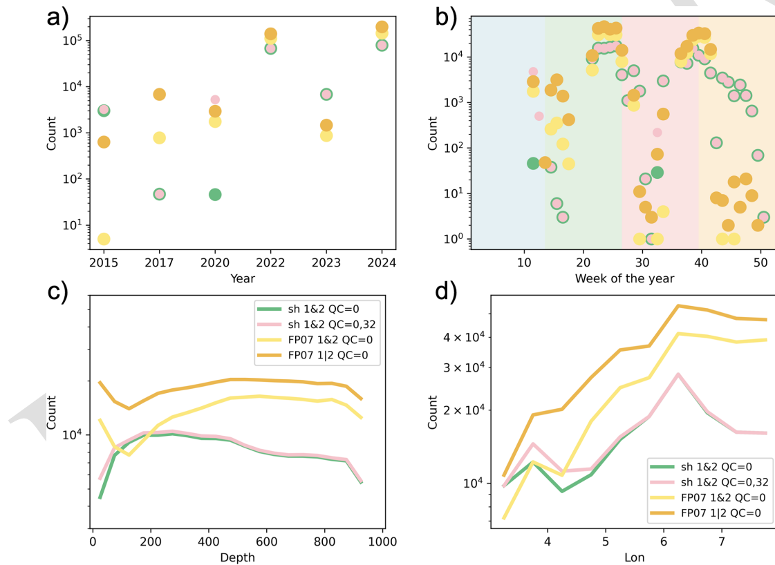
Figure 7. Count of passing data by bins of: years, week of the year, depth, and longitude. Green indicates the (best) cross-probe choice for shears and pink as a secondary cross-probe choice considering a relaxed despiking fraction criteria. Yellow indicates that both FP07 estimates pass; orange one on two.
