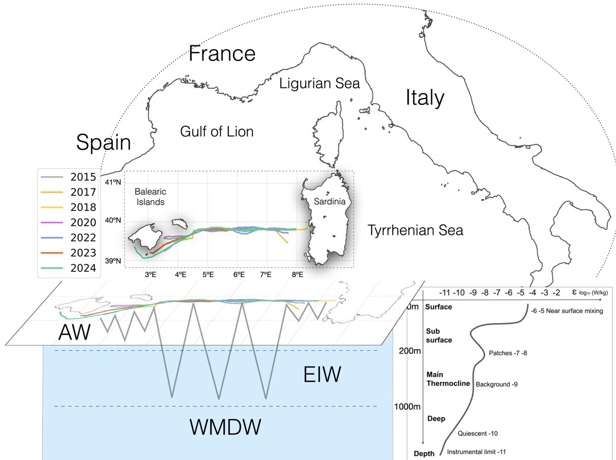
Figure 1. Glider Teresa mission along its longitudinal transect, by years (in colors). The scheme indicates the deployment between Sardinia and Balearic Islands in the Western Mediterranean Sea. Sawtooth black lines indicate a schematic trajectory from surface up to 1000 m-depth, encountering layers of the Atlantic Water (AW) in surface, the Eastern Intermediate Water (EIW) and the Western Mediterranean Deep Water (WMDW). Depth levels associated to these water masses (respectively 0–200 m, 200–1000 m, 1000 m+) are indicative. The lower-right panel provides a schematic representation of typical ranges of turbulent kinetic energy dissipation rates ( \epsilon , logarithmic scale) as a function of depth.
