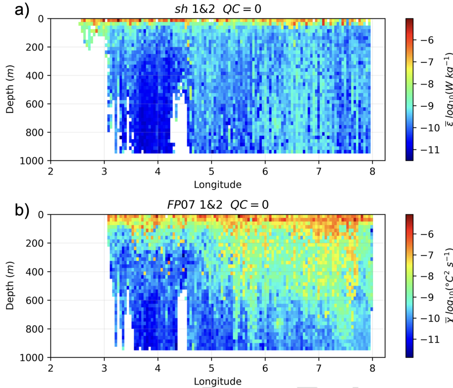
Figure 8. Synthetic sections of all good estimates of \epsilon and \chi (all years considered) averaged by depth bins of 25 m, and longitudinal bins of 0.045^\circ (circa 5 km).
