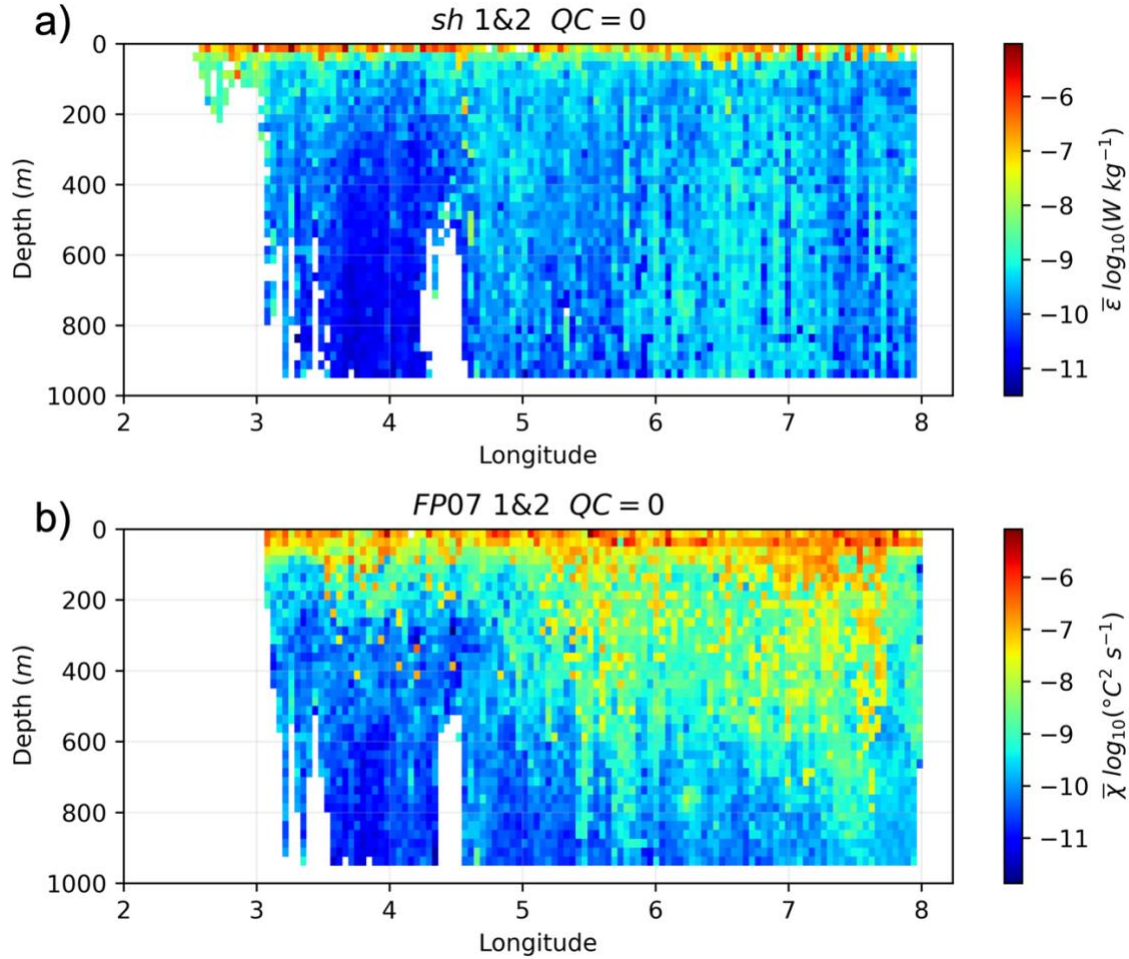
665 Figure 8: Synthetic sections of all good estimates of \varepsilon and \chi (all years considered) averaged by depth bins of 25m, and longitudinal 670 bins of 0.045^\circ (circa 5 km).
