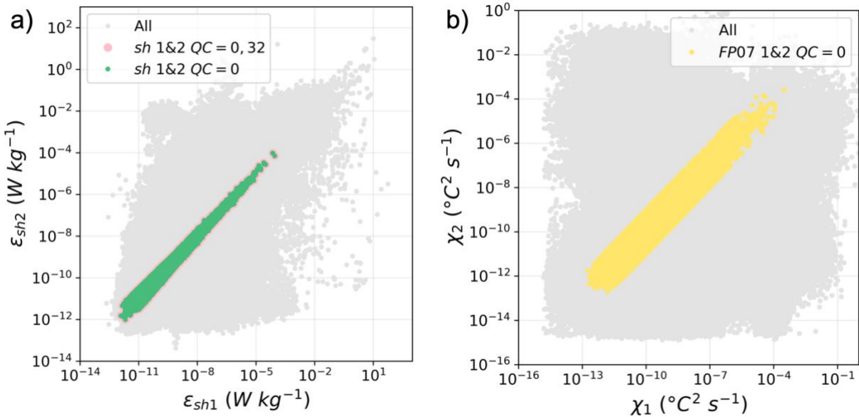
Figure 5 : Scatter plots of cross-checked estimates of (\epsilon_1, \epsilon_2) and (\chi_1, \chi_2) . Gray points indicate all estimates; (Left) green indicates the (best) cross-probe choice; (Right) yellow indicates that both FP07 estimates pass.
