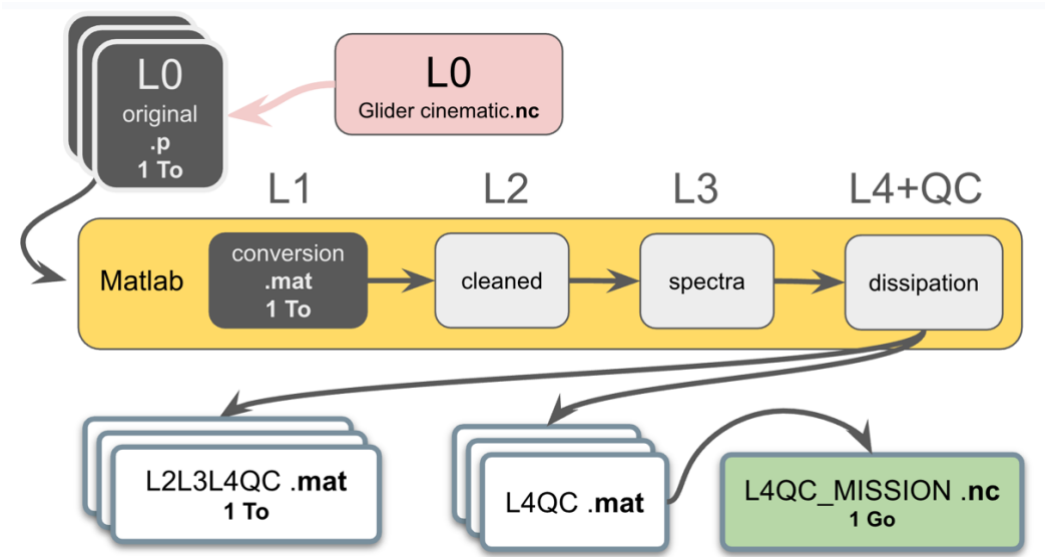
Figure 2: Scheme of the processing steps along the various levels.
