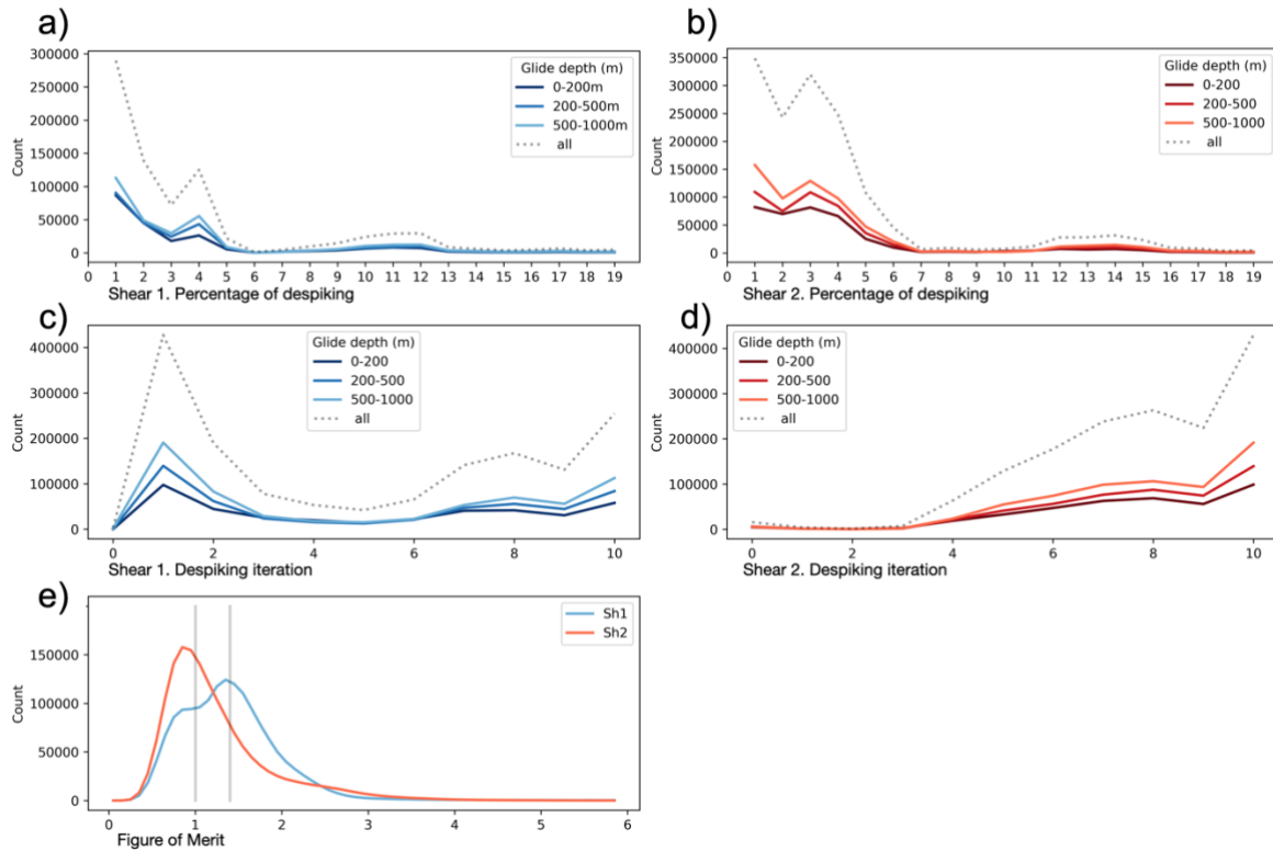
Figure 3: Count of spiking fraction (a,b) and pass count (c,d) for shear 1 (blue) and shear 2 probes (red), by bins of glider depth extension, in meter (i.e. from short to long glide). Count of FOM values (e) for shear 1 (blue) and shear 2 (red).
