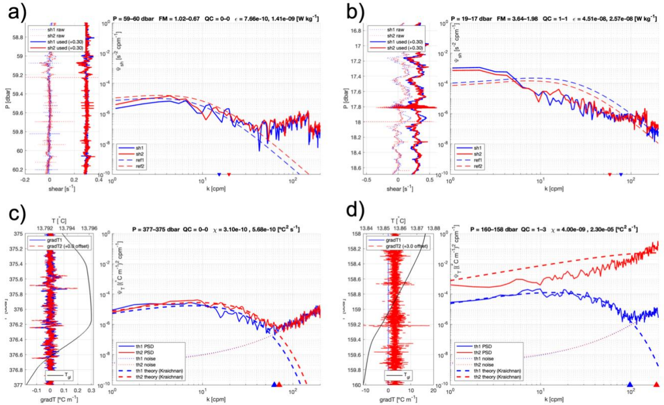
Figure 4. Examples of shear- and thermistor-based spectra illustrating accepted and rejected estimates.
