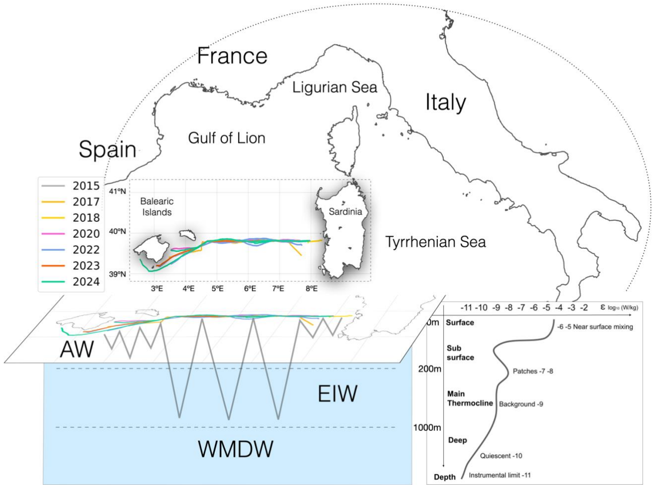
Figure 1. Glider Teresa mission along its longitudinal transect, by years (in colors). The scheme indicates the deployment between Sardinia and Balearic Islands in the Western Mediterranean Sea. Sawing black lines indicate a schematic trajectory from surface up to 1000m-depth, encountering layers of the Atlantic Water (AW) in surface, the Eastern Intermediate Water (EIW) and the Western Mediterranean Deep Water (WMDW). Depth levels associated to these water masses (respectively 0-200m, 200-1000m, 1000m+) are indicative. The lower-right panel provides a schematic representation of typical ranges of turbulent kinetic energy dissipation rates ( \epsilon , logarithmic scale) as a function of depth.
