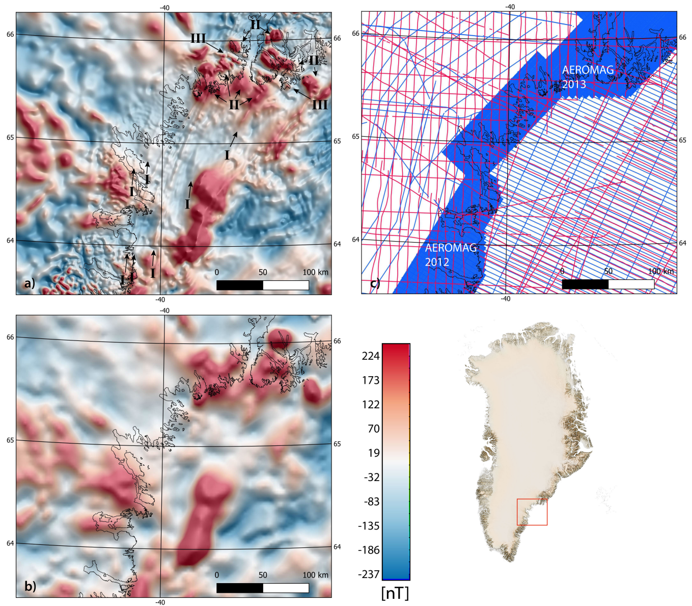
Figure 9. The magnetic anomaly data of (a) the new compilation and (b) the CAMP-M compilation (Gaina et al., 2011) are shown for the southeastern part of Greenland. c) Only data shown in red are used for the CAMP-M compilation, but both red and blue colored data points are used in the new compilation.
