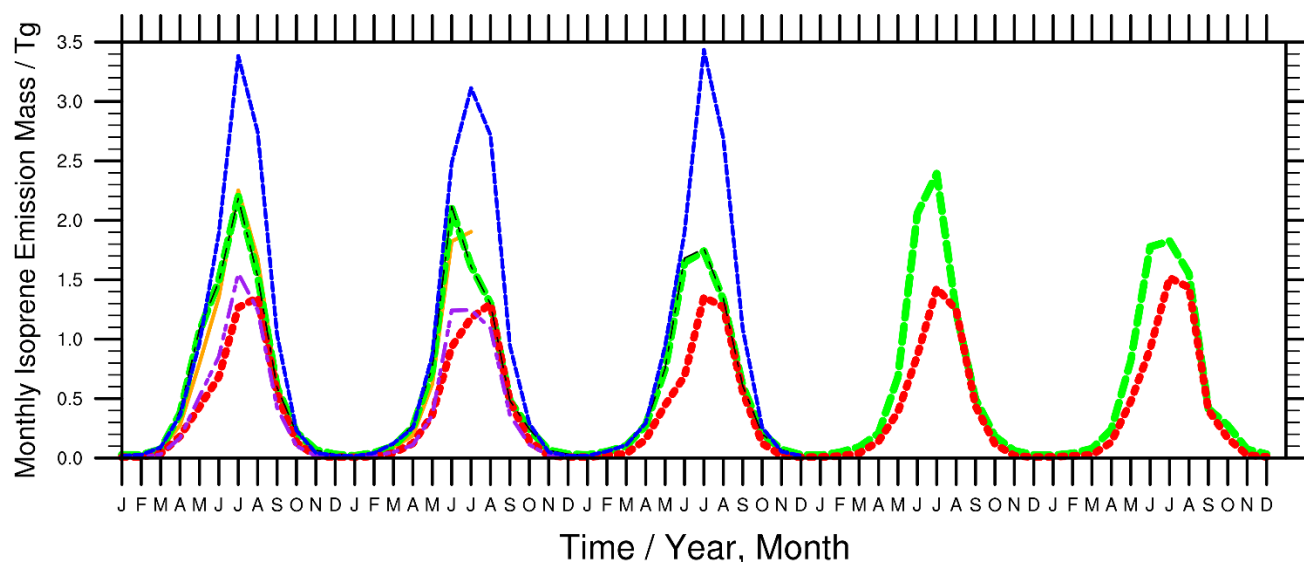
Figure 16. A time series of the monthly mean total emitted isoprene over the 2018-2022 period as calculated the SURFEX-MEGAN3.0 OL (green solid), SURFEX-MEGAN3.0 Analysis (black dot-dash), MEGAN-MACC (blue dash), CAMS-GLOB-BIOv1.2 (orange solid), CAMS-GLOB-BIOv3.0 (purple dash), and CAMS-GLOB-BIOv3.1 (red dash), emission inventories. The units of the isoprene emission totals are in Tg. The SURFEX-MEGAN3.0 OL and CAMS-GLOB-BIOv3.1 emission inventories are available over the full time period of 2018-2022, while the SURFEX-MEGAN3.0 Analysis and MEGAN-MACC emissions are only available over the period 2018-2020, the CAMS-GLOB-BIOv1.2 are only available 2018-July 2019, and the CAMS-GLOB-BIOv3.0 are only available 2018-2019.
