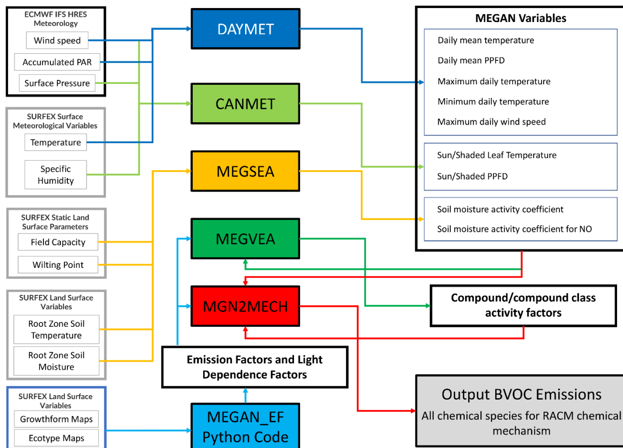
245 Figure 2. A detailed flow diagram of the MEGAN3.0 BVOC emission model as used in our application. The five modelling components of MEGAN3.0 are shown in the coloured boxes (DAYMET in dark blue, CANMET in light green, MEGSEA in orange, MEGVEA in dark green, MGN2MECH in red). Note that MEGAN3.0 has to be run sequentially in this order. The MEGAN emission factor pre-processor shown in a light blue box must be run prior to the final MEGAN3.0 step (MGN2MECH). Note that the input and output flows for each model sub-component are represented using corresponding colour coded arrows. 250 The various intermediate inputs and outputs are shown in light grey boxes. Lastly, the output BVOC emissions calculated by MEGAN3.0 from the MGN2MECH routine are shown in the grey-filled box.
