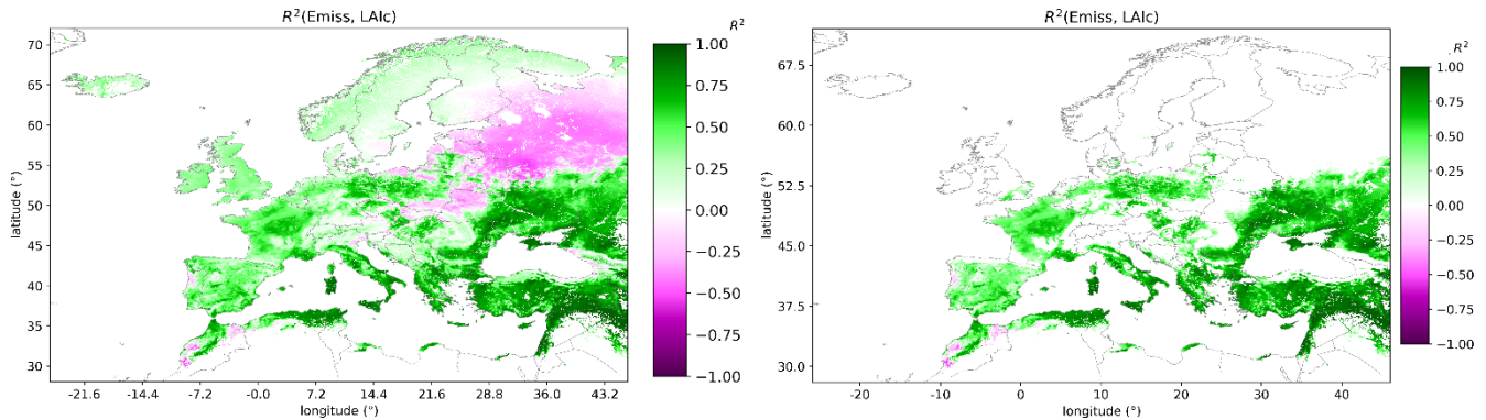
665 Figure 12. Maps of the correlation between LAI and the daily mean isoprene emissions over the CAMS European domain for the June to August 2019 time period. The left-hand panel shows the correlations for all grid cells within Europe while the right-hand panel shows the correlations only in locations where the LAI decreased between June 1 st and August 31 st . The colour bar shows green areas where the correlation was positive while the red areas shows where the correlation was negative.
