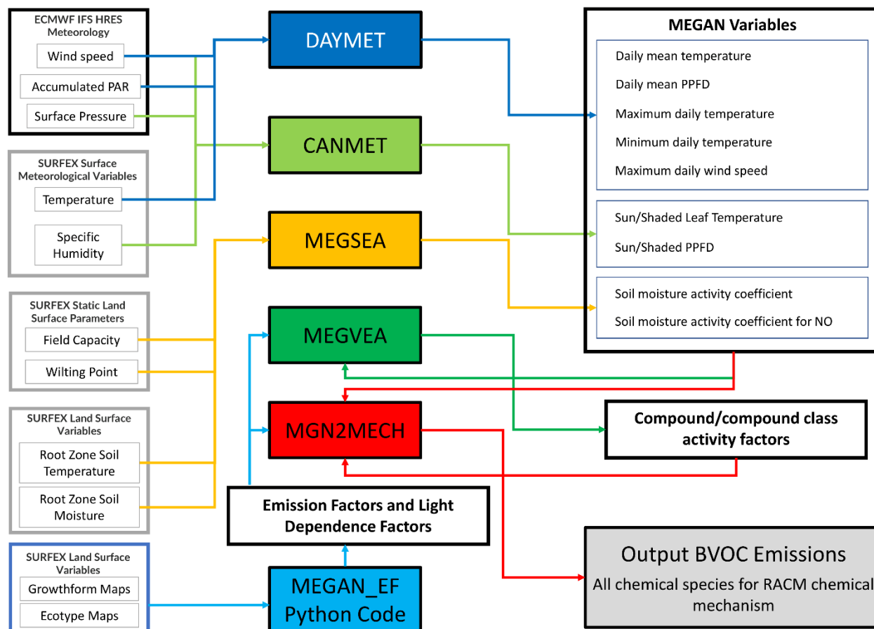
260 Figure 2. A detailed flow diagram of the MEGAN3.0 BVOC emission model as used in our application. The five modelling components of MEGAN3.0 are shown in the coloured boxes (DAYMET in dark blue, CANMET in light green, MEGSEA in orange, MEGVEA in dark green, MGN2MECH in red). Note that MEGAN3.0 has to be run sequentially in this order. The MEGAN emission factor pre-processor shown in a light blue box must be run prior to the final MEGAN3.0 step (MGN2MECH). Note that the input and output flows for each model sub-component are represented using corresponding colour coded arrows. 265 The various intermediate inputs and outputs are shown in light grey boxes. Lastly, the output BVOC emissions calculated by MEGAN3.0 from the MGN2MECH routine are shown in the grey-filled box.
