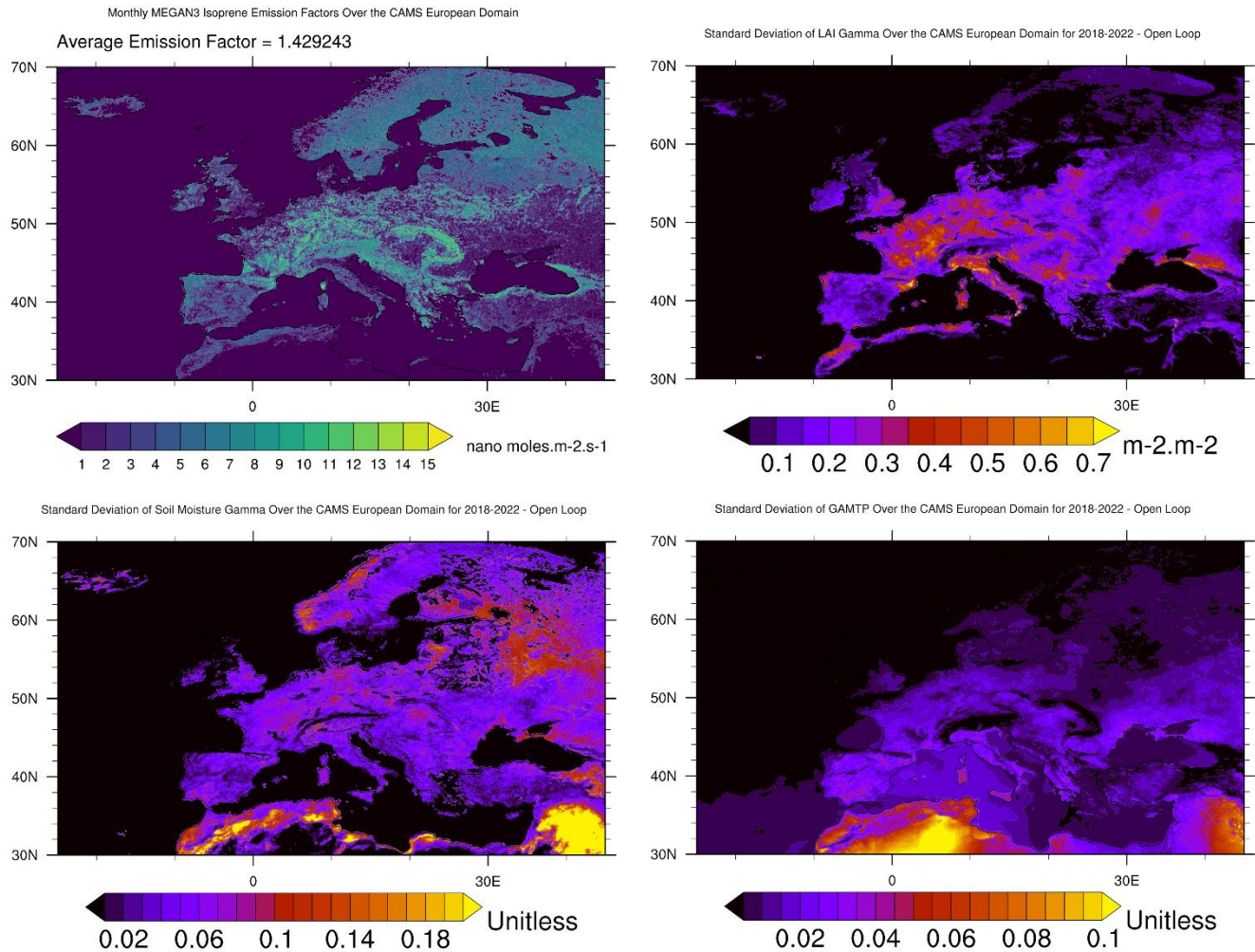
Figure 7. Maps of the MEGAN3.0 EFP isoprene emission factors in units of nano moles m^{-2} s^{-1} (top left), the LAI gamma in units of m^{-2}.m^{-2} (top right), the soil moisture gamma (unitless) (bottom left), and the temperature-radiation gamma in the bottom right.
