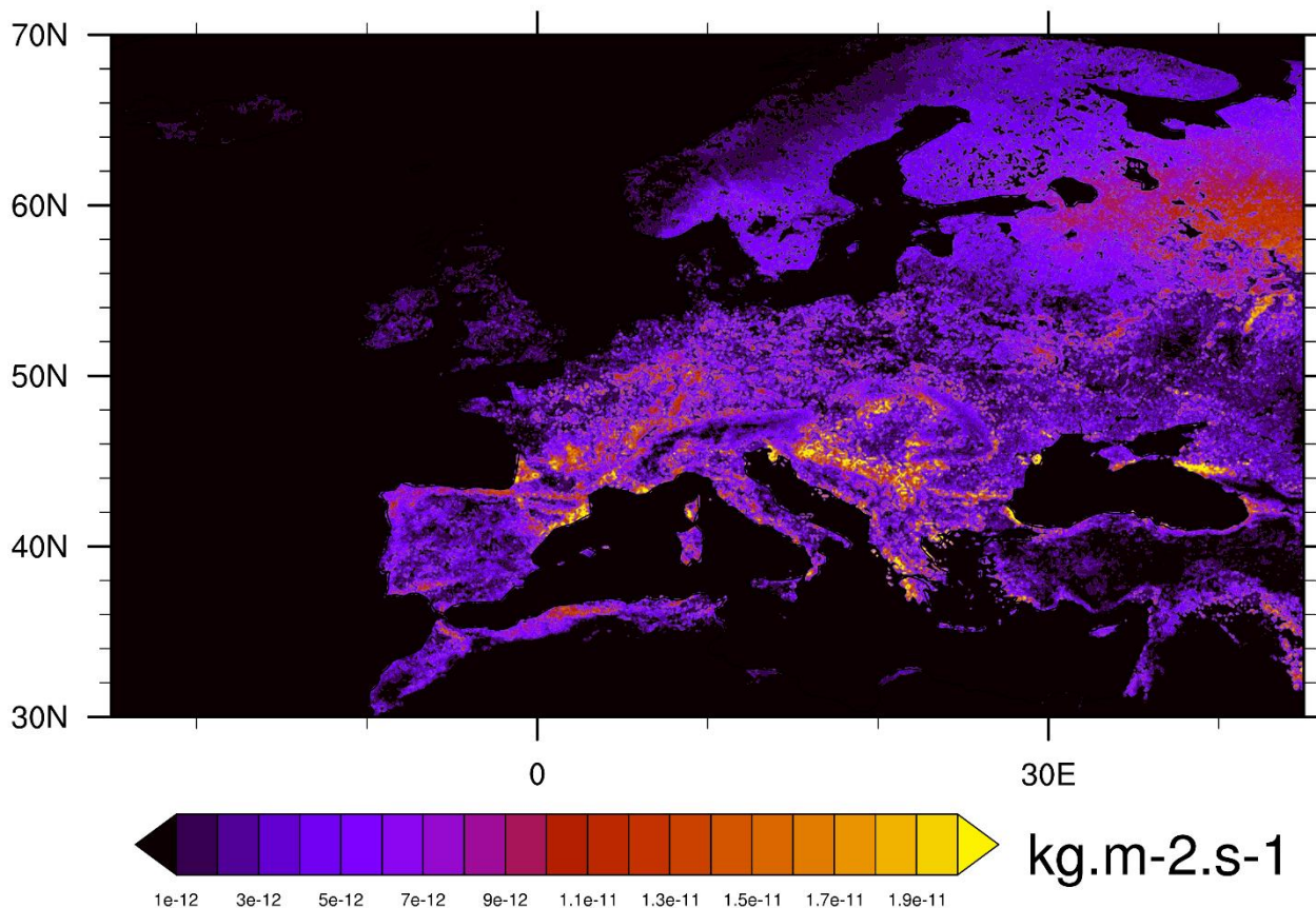
565 Figure 6. The standard deviation of isoprene emissions over the CAMS European domain for the 2018-2022 period based on the SURFEX model open-loop simulations. Note that the standard deviation is expressed in the units of the emissions ( \text{kg.m}^{-2}\text{s}^{-1} ).
