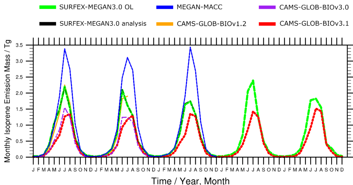
940 Figure 16. A time series of the monthly mean total emitted isoprene over the 2018-2022 period as calculated the SURFEX- MEGAN3.0 OL (green solid), SURFEX-MEGAN3.0 analysis (black dot-dash), MEGAN-MACC (blue dash), CAMS-GLOB- BIOv1.2 (orange solid), CAMS-GLOB-BIOv3.0 (purple dash), and CAMS-GLOB-BIOv3.1 (red dash), emission inventories. The units of the isoprene emission totals are in Tg. The SURFEX-MEGAN3.0 OL and CAMS-GLOB-BIOv3.1 emission inventories are available over the full time period of 2018-2022, while the SURFEX-MEGAN3.0 analysis and MEGAN-MACC emissions are only 945 available over the period 2018-2020, the CAMS-GLOB-BIOv1.2 are only available 2018-July 2019, and the CAMS-GLOB- BIOv3.0 are only available 2018-2019.
