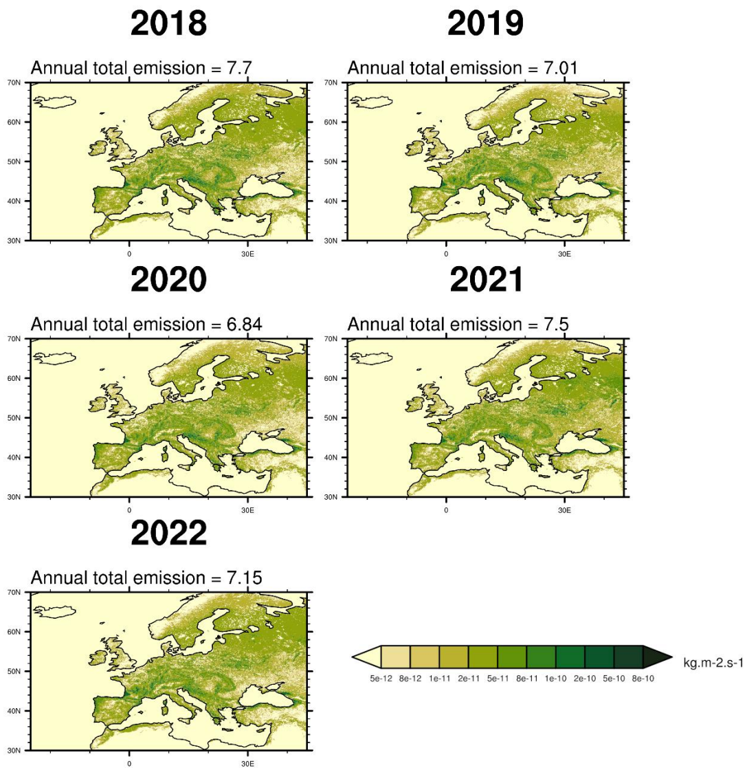
560 Figure 5. Maps of annual mean isoprene emissions (units of \text{kg}\cdot\text{m}^{-2}\cdot\text{s}^{-1} ) calculated using the SURFEX-MEGAN3.0 algorithms over the period 2018-2022 using the open-loop configuration of SURFEX. The panels show each year over this time period moving sequentially from 2018 to 2022 from left to right. The colour bars indicate increasing mean isoprene emissions as the colours transition from pale yellow to dark green. Note that the colour bar has a quasi-logarithmic scale. The annual total mass of isoprene emissions (units of Tg) are shown above each plot.
