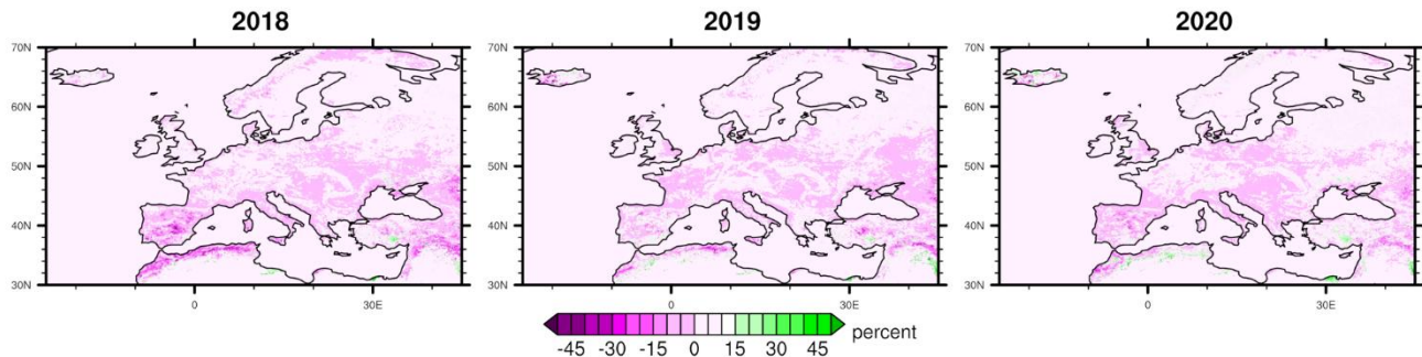
Figure 14. Maps of annual mean isoprene emissions (units of \text{kg}\cdot\text{m}^{-2}\cdot\text{s}^{-1} ) calculated using the SURFEX-MEGAN3.0 LAI analysis configuration of SURFEX (top-row), the difference between the LAI analysis minus the open-loop configurations (middle-row), and the percentage difference between the LAI analysis minus open-loop over the period 2018-2020. The panels show each year over this time period moving sequentially from 2018 to 2020 from left to right. The top-row colour bars indicate increasing mean isoprene emissions as the colours transition from pale yellow to dark green. The middle-row colour bars indicate the difference in annual mean isoprene emissions between the LAI-analysis and open-loop configurations with red colours indicating larger annual mean open-loop emissions and green indicating larger LAI-analysis based emissions. The bottom-row colour bar indicates the percentage difference in mean annual isoprene emissions between the LAI-analysis and open-loop with green indicating larger LAI-analysis based emissions and red indicating larger open-loop based emissions. The annual total mass of isoprene emissions
