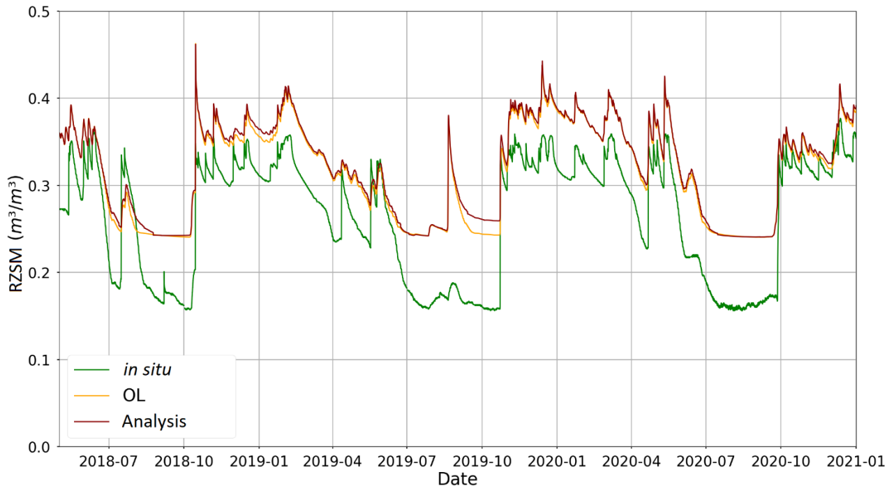
525 Figure 4. Time series of observed in-situ RZSM at the Saint-Felix de Lauragais SMOSMANIA monitoring station (green), the RZSM from the SURFEX open-loop simulation (yellow), and the RZSM from the SURFEX analysis simulation (red).
