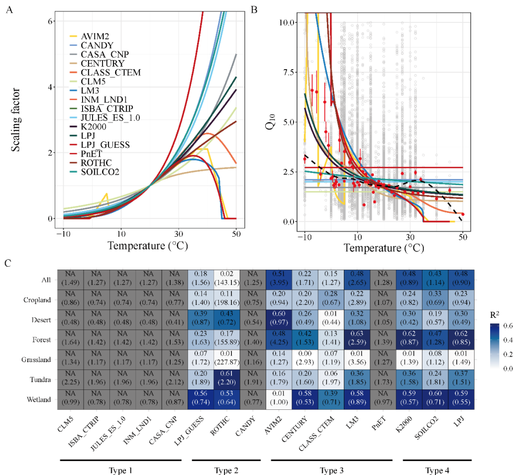
180 Figure 3: Performance of soil carbon temperature response functions. Temperature response functions of soil organic carbon mineralization (A), temperature sensitivity ( Q_{10} ) predicted by the temperature response functions (B), and function performance by comparing function predicted and observed Q_{10} (C). Gray open points in panel B represent observed Q_{10} values at different temperatures, while the black dashed curve shows the best-fit relationship between Q_{10} and temperature based on locally weighted polynomial regression. Red points indicate the mean values under the corresponding temperatures, and error bars represent one standard error of the observations. Panel C compares the observed mean Q_{10} values at different temperatures with the Q_{10} values predicted by the temperature response functions, presented for both global average and subsets grouped by ecosystem type. In panel C, numbers outside the parentheses represent the coefficient of determination ( R^2 ), while numbers inside the parentheses indicate the root mean square error. Grey grids represent cases where R^2 could not be calculated due to constant Q_{10} values defined by the respective temperature response functions.
