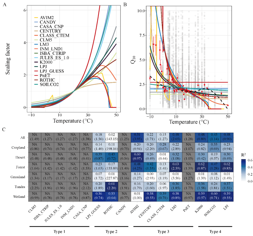
180 Figure 3: Performance of soil carbon temperature response functions. Temperature response functions of soil organic carbon mineralization (A), temperature sensitivity ( Q_{10} ) predicted by the temperature response functions (B), and function performance by comparing function predicted and observed Q_{10} (C). Gray open points in panel B represent observed Q_{10} values at different temperatures, while the black dashed curve shows the best-fit relationship between Q_{10} and temperature based on locally weighted polynomial regression. Red points indicate the mean values under the corresponding temperatures, and error bars represent one standard error of the observations. Panel C compares the observed mean Q_{10} values at different temperatures with the Q_{10} values predicted by the temperature response functions, presented for both global average and subsets grouped by ecosystem type. In panel C, numbers outside the parentheses represent the coefficient of determination ( R^2 ), while numbers inside the parentheses indicate the root mean square error. Grey grids represent cases where R^2 could not be calculated due to constant Q_{10} values defined by the respective temperature response functions.
