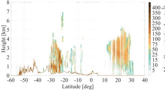
(h) Pure-dust Mass Concentration
