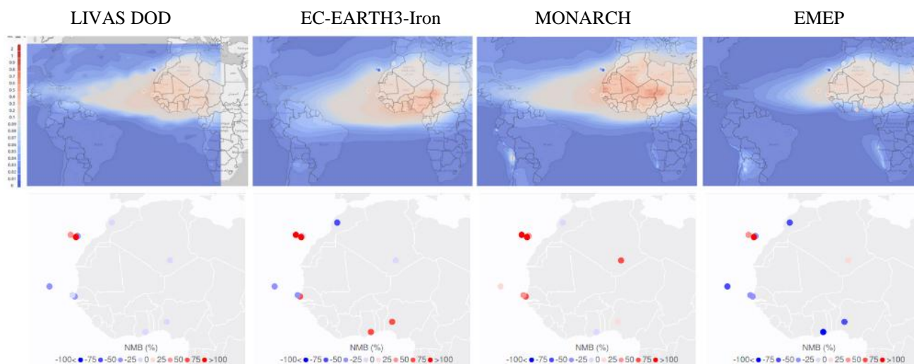
795 Figure 8: Yearly mean DOD (upper panels) and Normalized Mean Bias with respect to AERONET coarse-mode AOD (lower panels) for LIVAS, EC-Earth3, MONARCH, and EMEP for the year 2020. On the upper maps, AERONET data is also presented by the circles.
