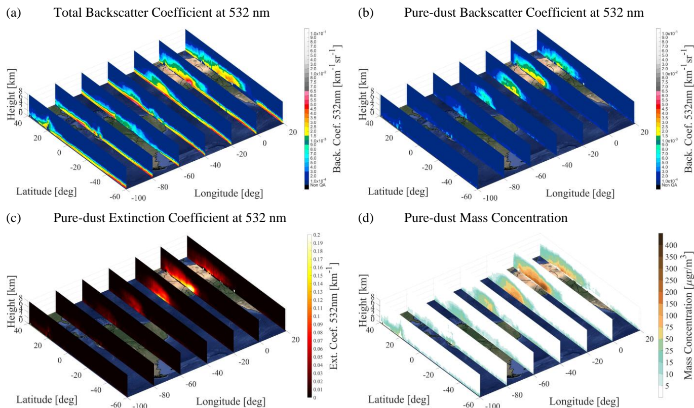
380 Figure 3: Annual-mean four-dimensional (4D) reconstruction of the atmosphere in terms of total backscatter coefficient at 532 nm (Fig. 3a), pure-dust backscatter coefficient at 532 nm (Fig. 3b), pure-dust extinction coefficient at 532 nm (Fig. 3c), and pure-dust mass concentration (Fig. 3d) in 1^\circ \times 1^\circ spatial resolution and for the period 12/2006-11/2022.
