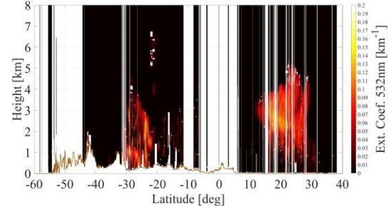
(g) Pure-dust Extinction Coefficient at 532 nm
