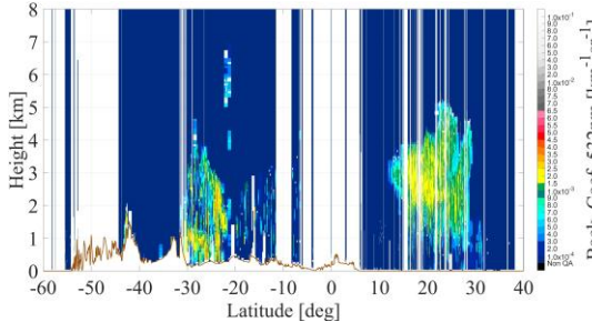
(f) Pure-dust Backscatter Coefficient at 532 nm
