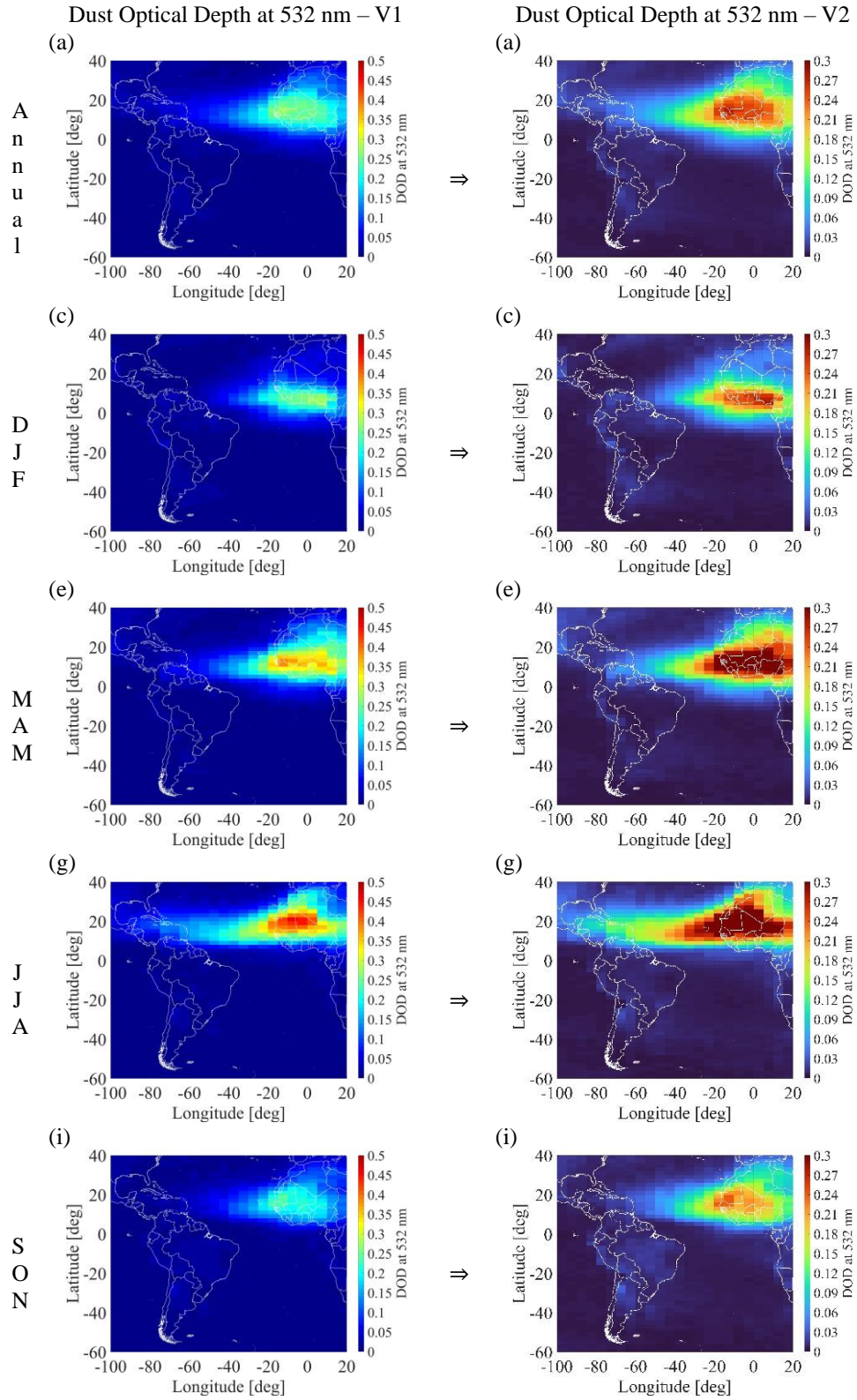
Figure: LIVAS Dust Optical Depth at 532 nm (DOD), provided in annual-mean, DJF, MAM, JJA, and SON, estimated for the period 12/2006-11/2022. Left column: Initial version of figures. Right column: updated version of figures.
