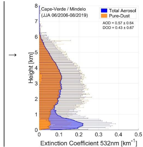
Extinction Coefficient at 532nm profile
