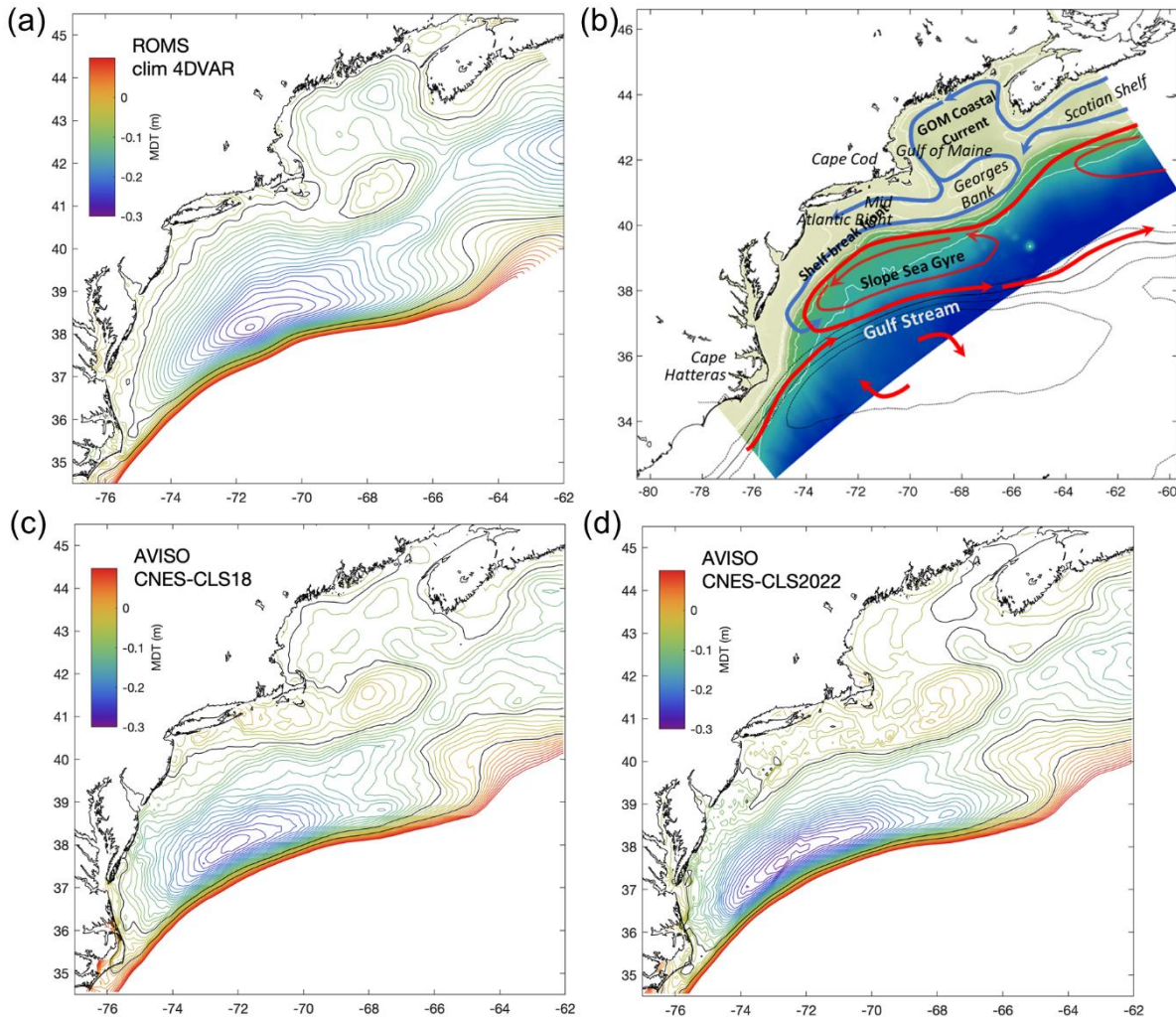
345 Figure 7: (a) ROMS model MDT contours, (b) Mid Atlantic Bight circulation, (c) CNES-CLS18 MDT contours and (d) CNES-CLS22 MDT contours. Black lines represent MDT contours at 0.05 m and -0.05 m.
