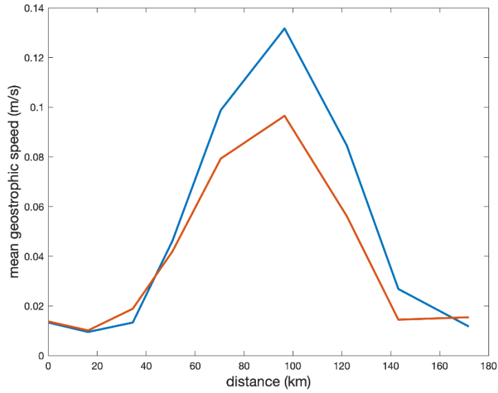
390 Figure 9: The mean geostrophic speed derived from CNES-CLS22 MDT (blue) and CNES-CLS18 MDT (red) across the Mohn Ridge (location of the transect shown in Fig. 9).
