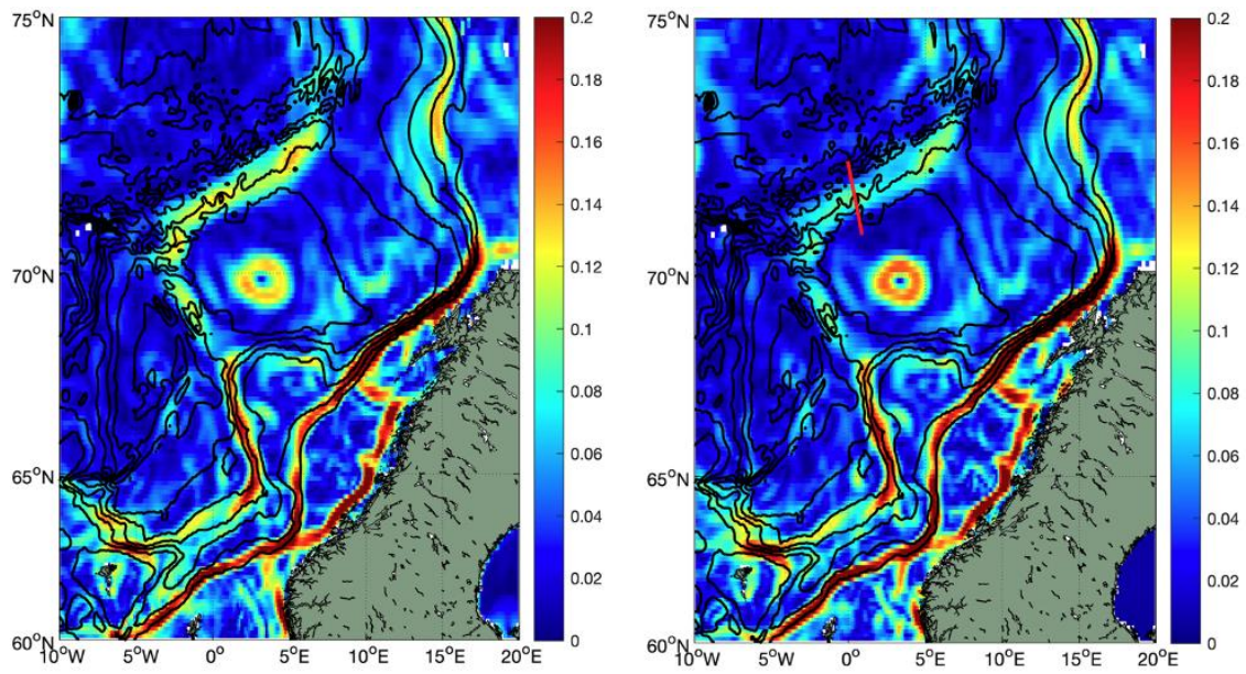
375 Figure 8: Mean geostrophic speeds (m/s) derived from: CNES_CLS22 MDT (left panel); and CNES_CLS18 MDT (right). The red line in the right panel indicates the location of the transect shown in Fig. 10. Isobaths are drawn in black.
