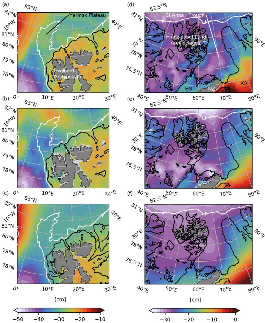
300 Figure 6: (a) CNES-CLS22 MDT, (b) CNES-CLS18 MDT and (c) DTUHH22 MDT in Yermak Plateau area. The white line represents the 1000 m isobath and the black line the 200 m isobath. Figure 7a shows the bathymetric and geographical features: the Yermak Plateau and Svalbard Archipelago. (d) CNES-CLS22 MDT, (e) CNES-CLS18 MDT and (f) DTUHH22 MDT in St Anna Through area. The white line represents the 1000 m isobath and the black line the 200 m isobath. Figure 7d shows the geographical features: the St Anna Through, the Franz Josef Land Archipelago, the Novaya Zemlya (NZ), the Barents Sea (BS) and the Kara Sea 305 (KS).
